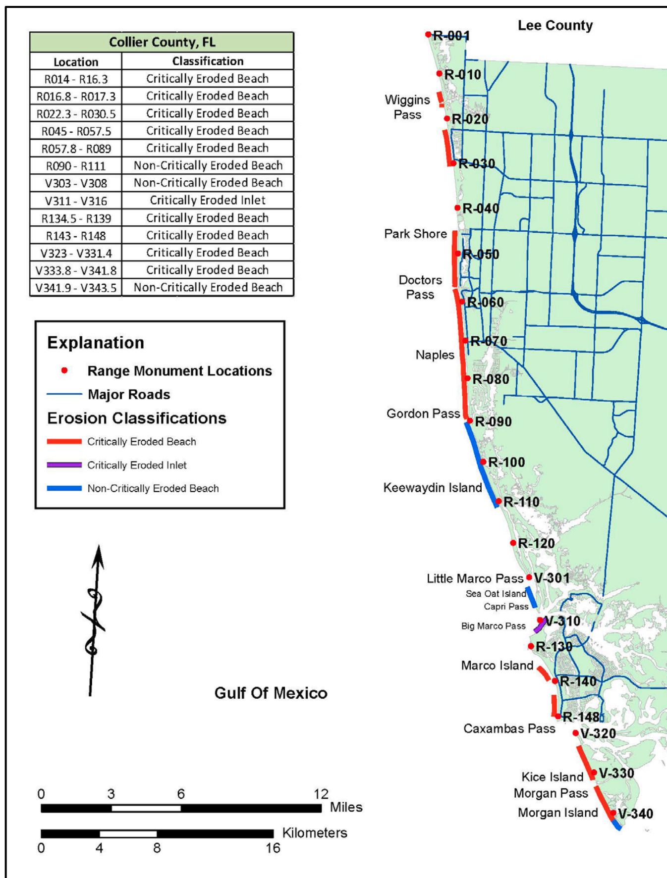
Figure 32. Critically eroded shoreline within Collier County.
