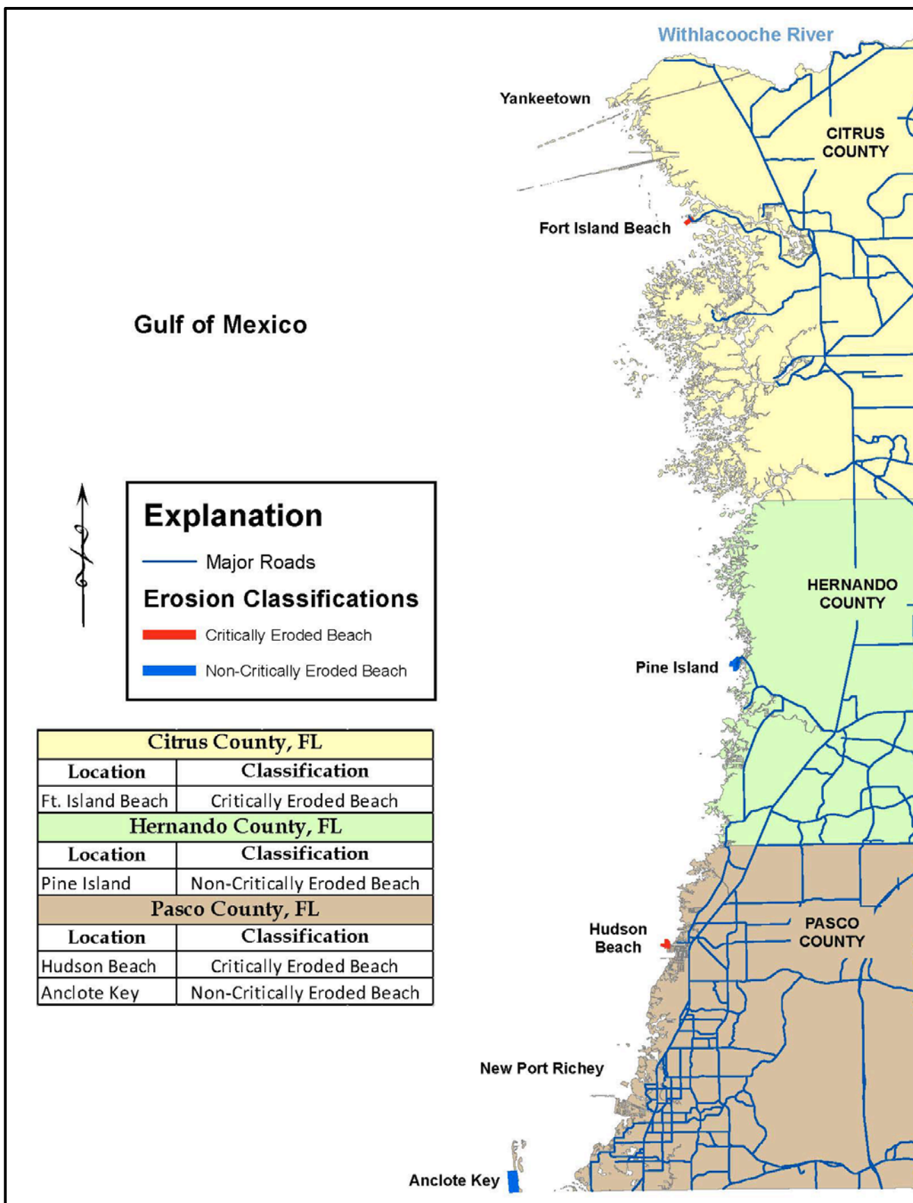
Figure 25. Critically eroded shoreline within Citrus, Hernando and Pasco Counties.
