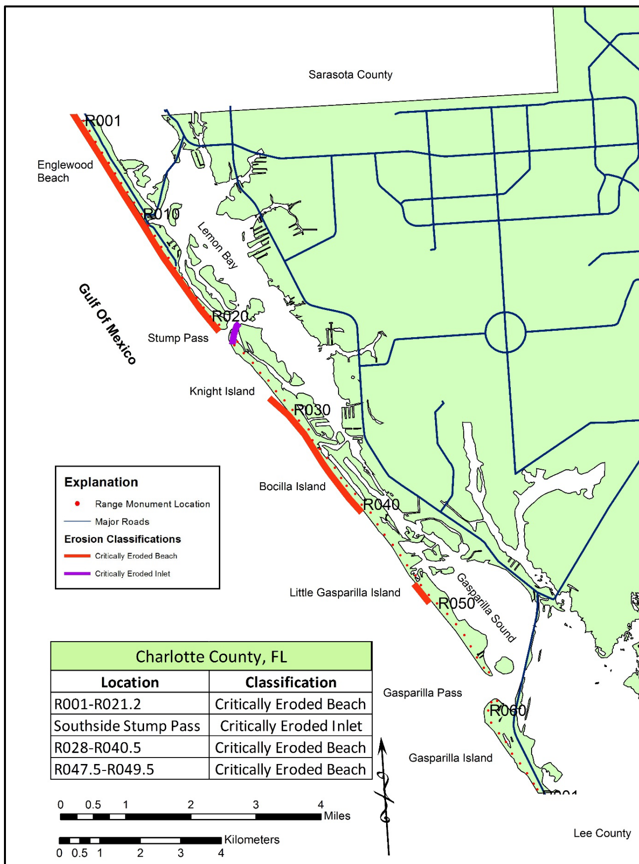
Figure 30. Critically eroded shoreline within Charlotte County.
