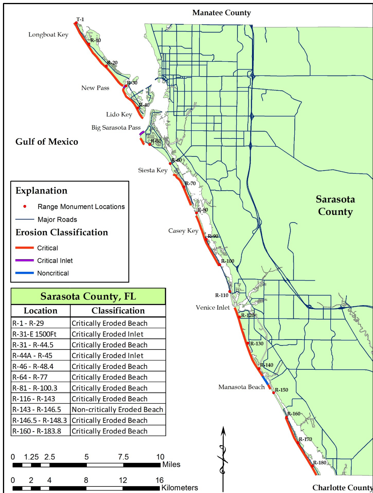
Figure 29. Critically eroded shoreline within Sarasota County.
