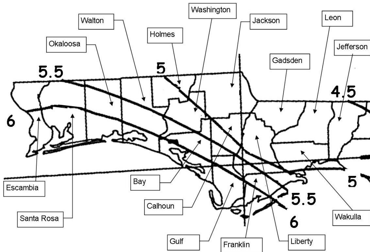
Figure 2.5-1 2-year, 24-hour Maximum Rainfall depth.
