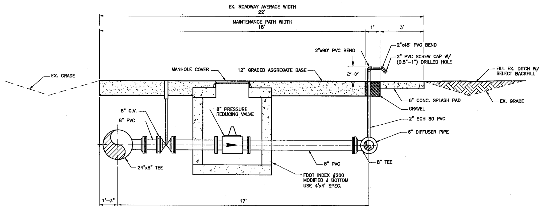
CROSS-SECTION OF DISTRIBUTION SYSTEM ALONG EXIST. ACCESS ROAD
