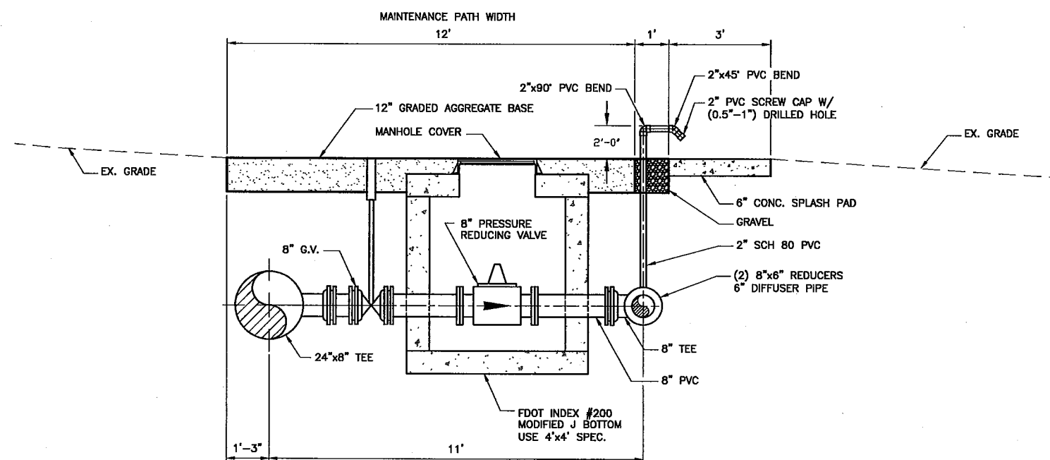
CROSS-SECTION OF DISTRIBUTION SYSTEM BEYOND EXIST. ACCESS ROAD
