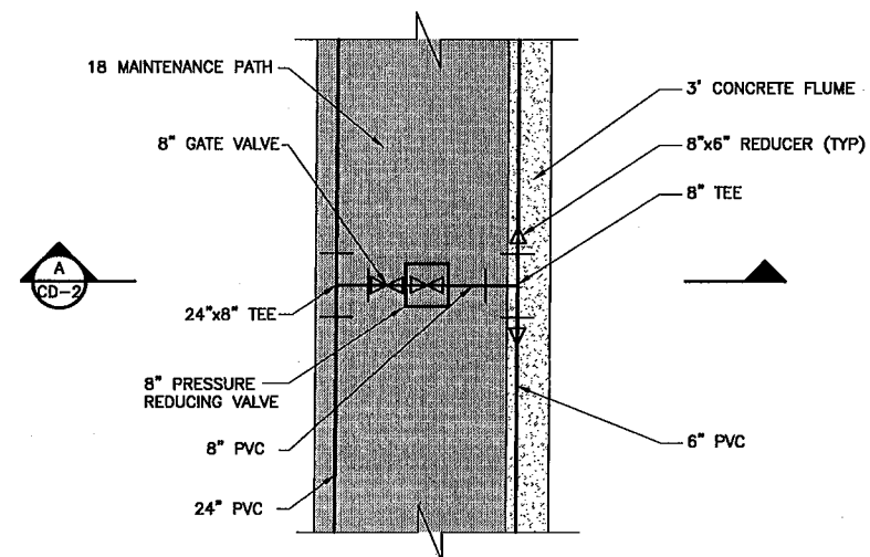
DISTRIBUTION LINE CROSSING EXIST. ACCESS ROAD
