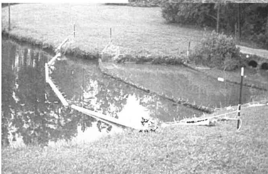
(Left) A series of particle curtains collect suspended flocculated material resulting in progressively clearer water.
