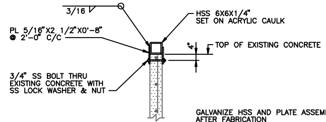
SECTION 8 NO SCALE SEE THIS DWG
