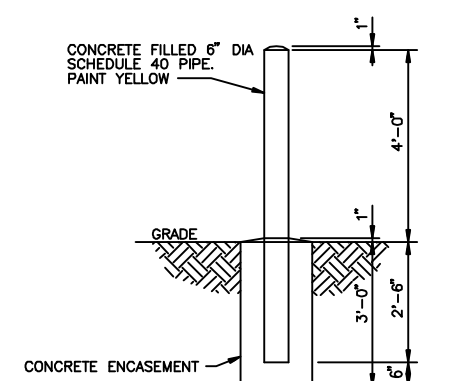
TYPICAL GUARD POST NO SCALE
