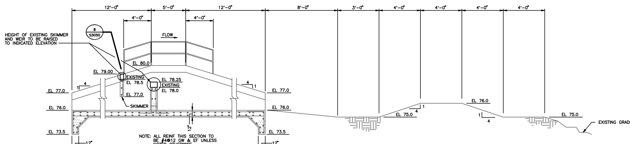
SECTION 6 NO SCALE SEE THIS DWG
