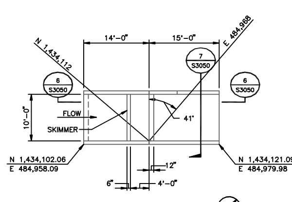
DETAIL 5 EXISTING DISCHARGE STRUCTURE NO. 2 SCALE: 1"=10' SEE DWG S3003
