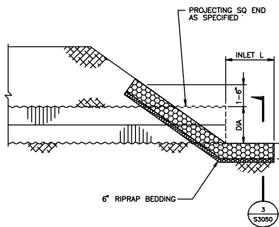
INLET END SEE RIPRAP TABLE
