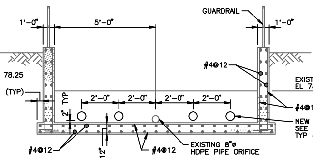
SECTION 7 NO SCALE SEE THIS DWG
