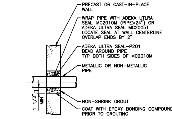
WALL PENETRATION DETAIL NO SCALE
