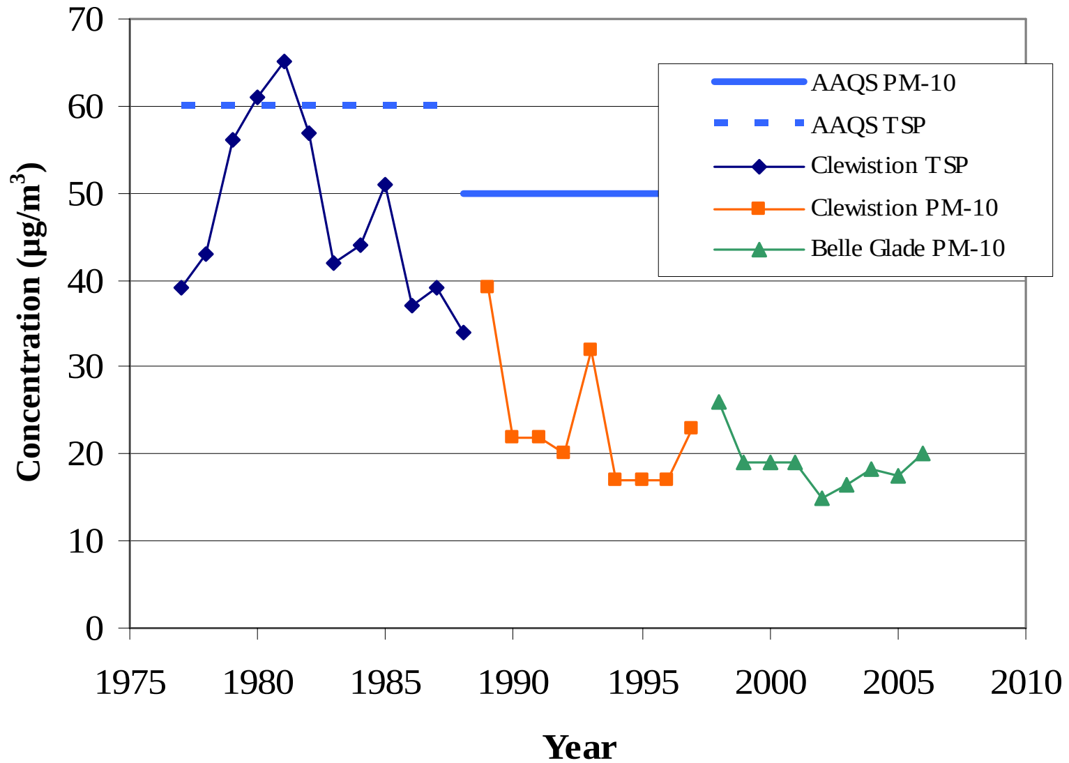
Figure 7-12 Annual Average \text{PM}_{10} and TSP Concentrations Measured from 1977 to 2006 - Hendry and Palm Beach Counties
