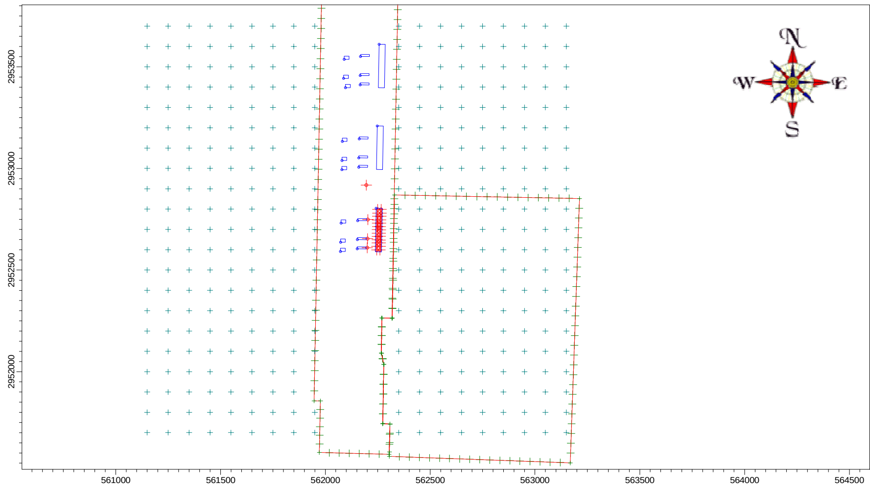
Figure E-4 FPL West County Unit 3 Project Receptor Grid Used in the AAQS and PSD Class II Increment Analyses for SO 2 For All Sources Excluding Hubbard Construction Company Source: Golder, 2007.
