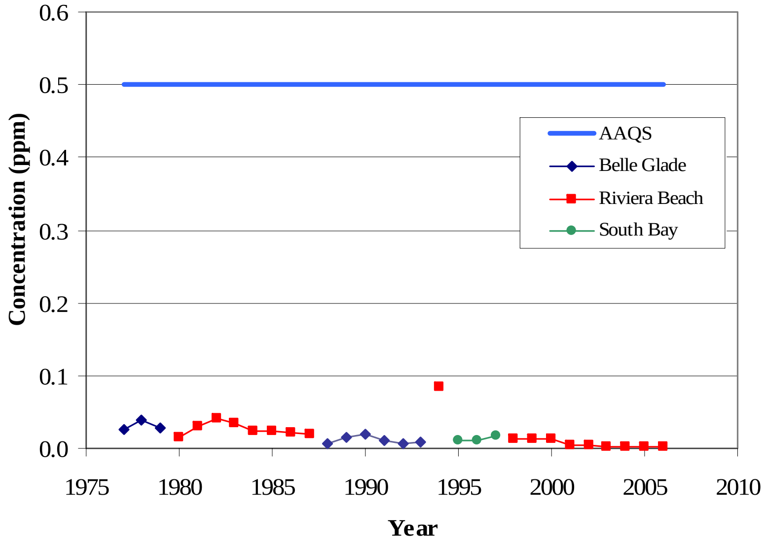
Figure 7-11 3-Hour Average Sulfur Dioxide Concentrations (2nd Highest Values) Measured from 1977 to 2006 - Palm Beach County
