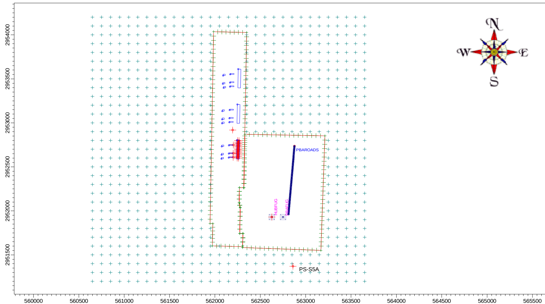
Figure E-7 FPL West County Unit 3 Project Receptor Grid Used in the AAQS and PSD Class II Increment Analyses for PM_{10} For All Sources Including Palm Beach Aggregates and Hubbard Construction Company Source: Golder, 2007.
