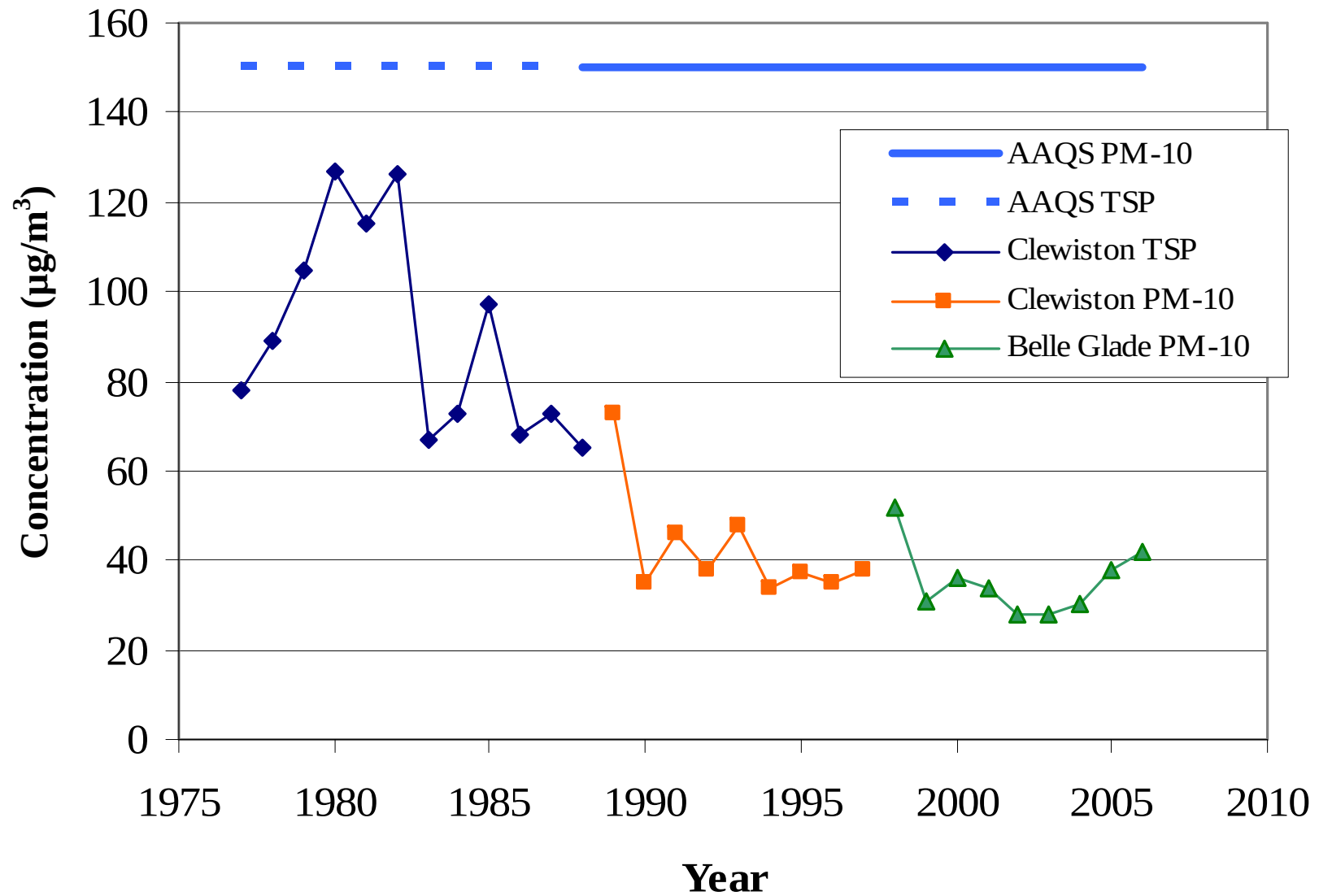
Figure 7-13 24-hour Average PM 10 and TSP Concentrations (2nd Highest Values) Measured from 1977 to 2006 - Hendry and Palm Beach Counties
