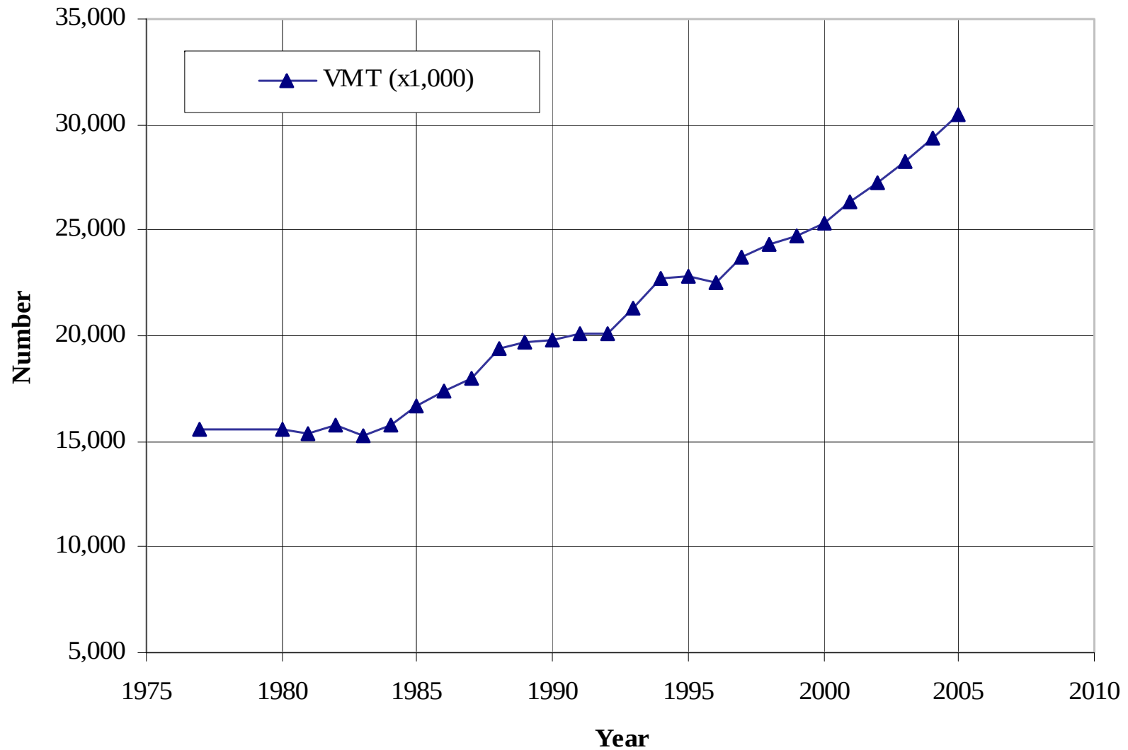
Figure 7-5 Vehicle Miles Traveled (VMT) Estimates for Motor Vehicles for Palm Beach County
