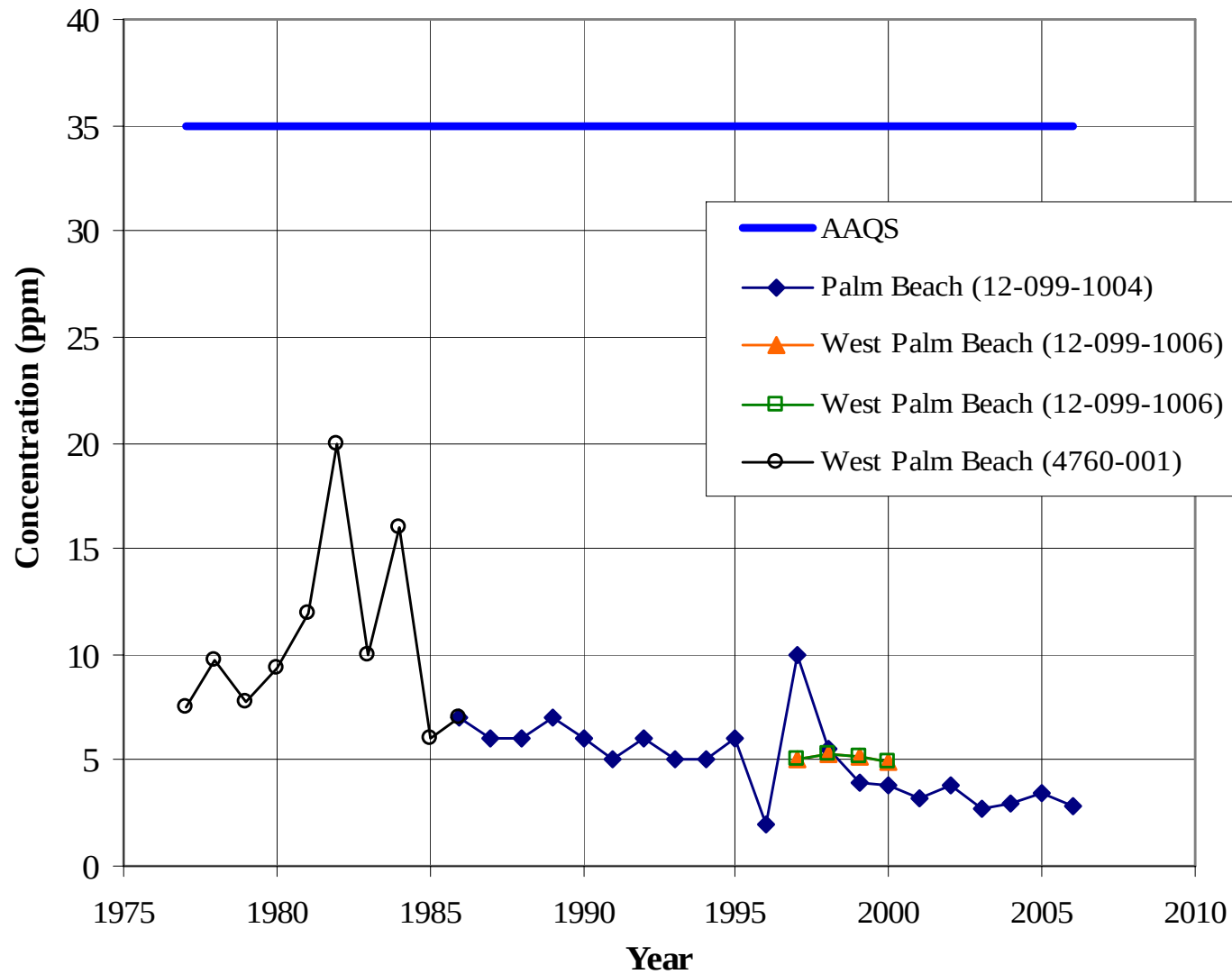
Figure 7-15 1-hour Average Carbon Monoxide Concentrations (2nd Highest Values) Measured from 1977 to 2006 - Palm Beach County
