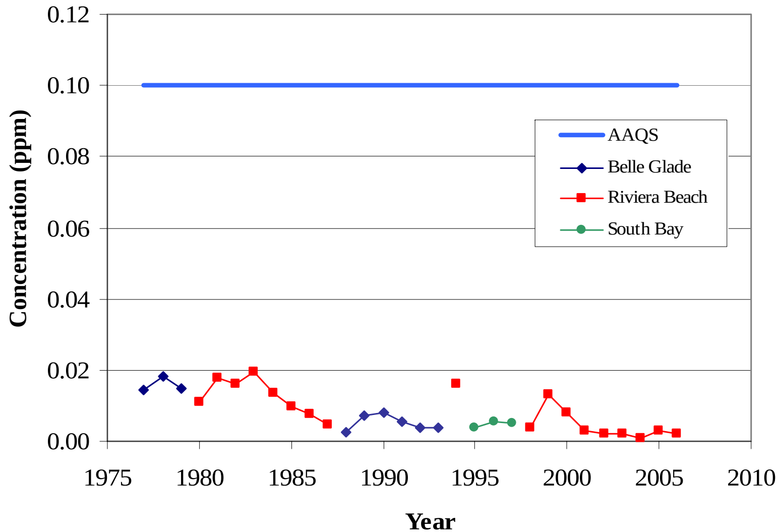
Figure 7-10 24-hour Average Sulfur Dioxide Concentrations (2nd Highest Values) Measured from 1977 to 2006 - Palm Beach County
