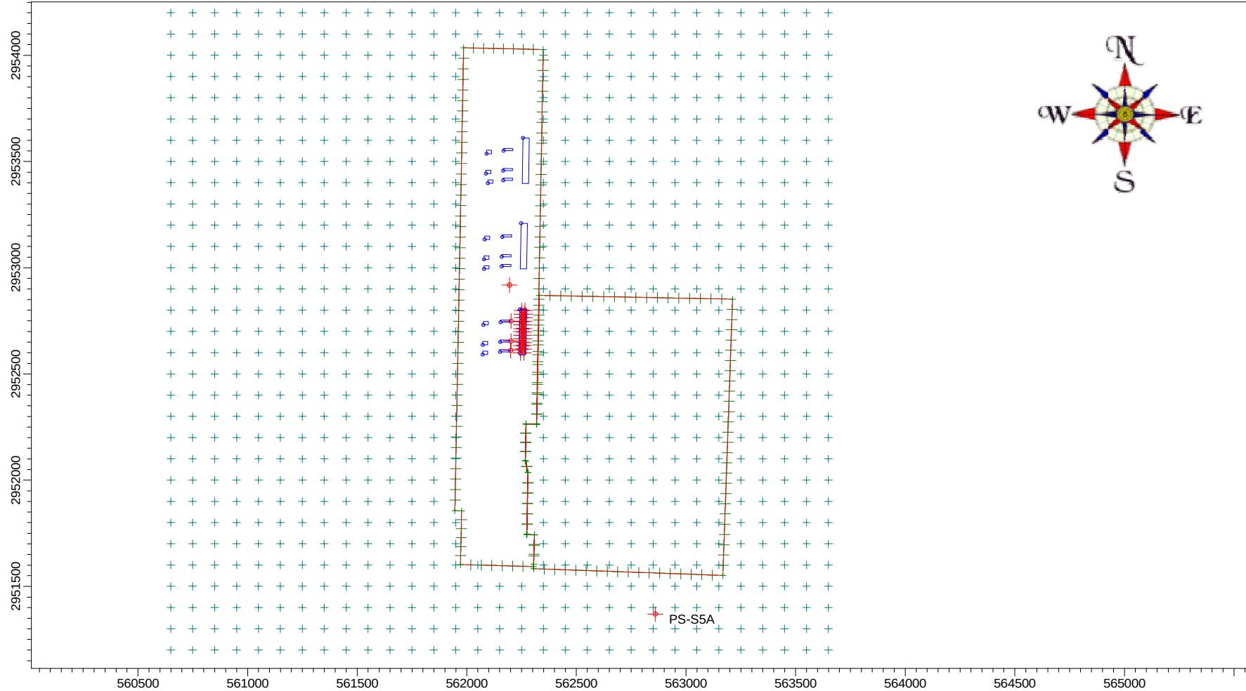
Figure E-6 FPL West County Unit 3 Project Receptor Grid Used in the AAQS and PSD Class II Increment Analyses for PM 10 For All Sources Excluding Palm Beach Aggregates and Hubbard Construction Company Source: Golder, 2007.
