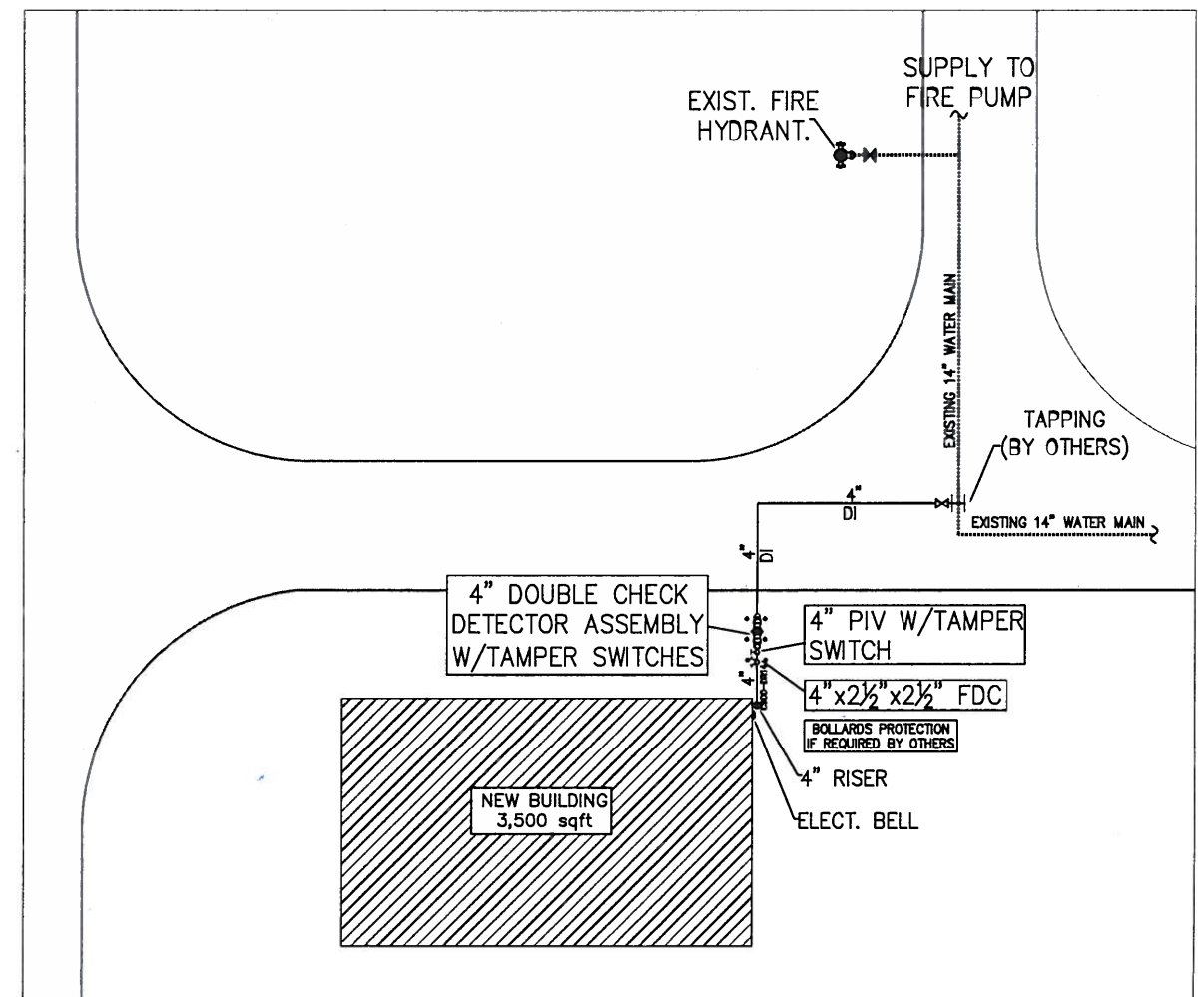
UNDERGROUND FIRE SPRINKLER PLAN NORTH N.T.S.
