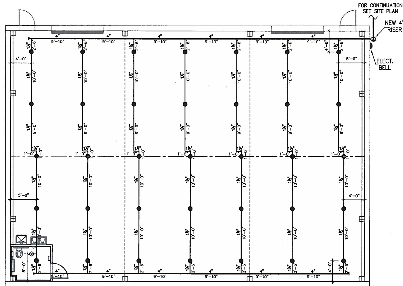
WAREHOUSE FIRE SPRINKLER PLAN SCALE 1/4"=1'-0" NORTH
