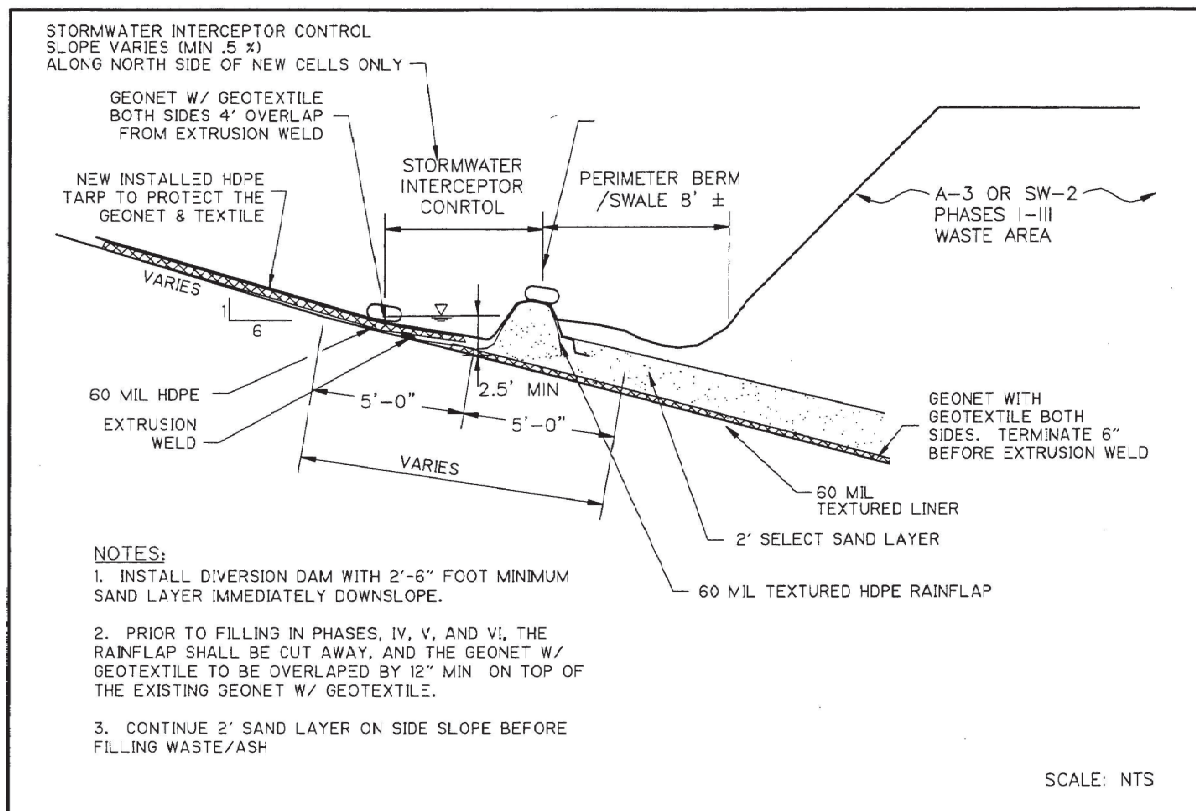
Figure No. 7 Stormwater Interceptor Control
