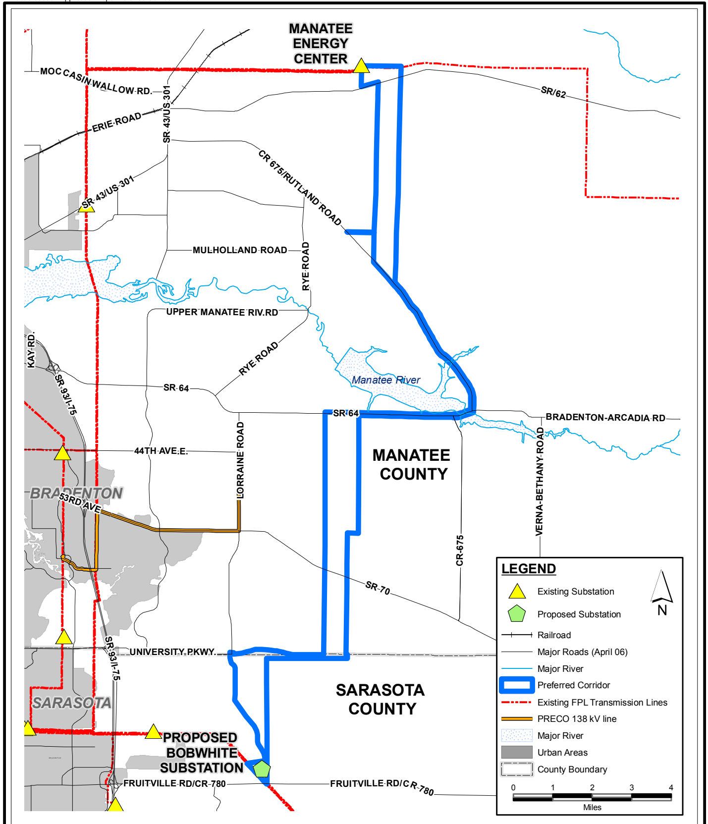
FIGURE 1.1-2. PREFERRED CORRIDOR ALIGNMENT
