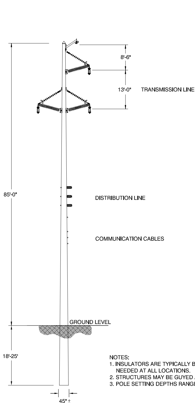
FIGURE 1.3-4. TYPICAL 85' TANGENT STRUCTURE TRIANGULAR CONFIGURATION WITH DISTRIBUTION / COMMUNICATION UNDERBUILD
