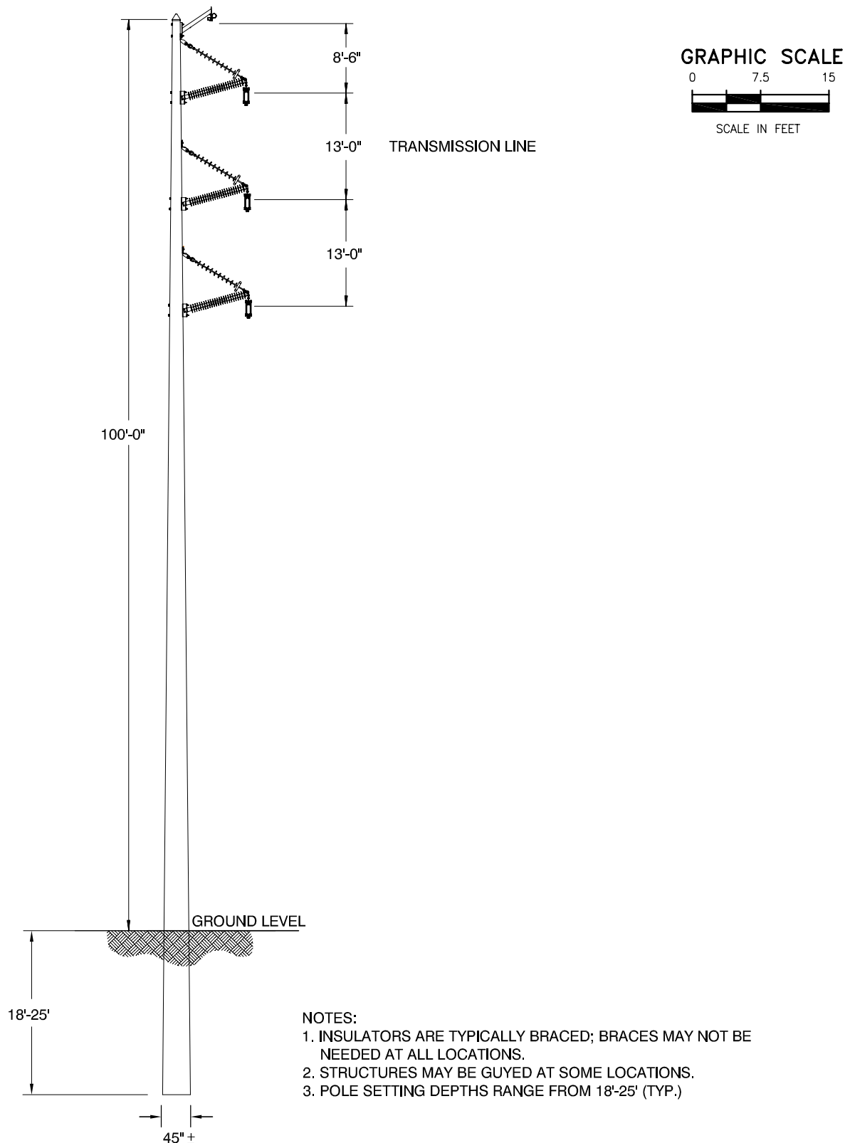
FIGURE 1.3-1. TYPICAL 100' TANGENT STRUCTURE VERTICAL CONFIGURATION WITHOUT DISTRIBUTION / COMMUNICATION UNDERBUILD
