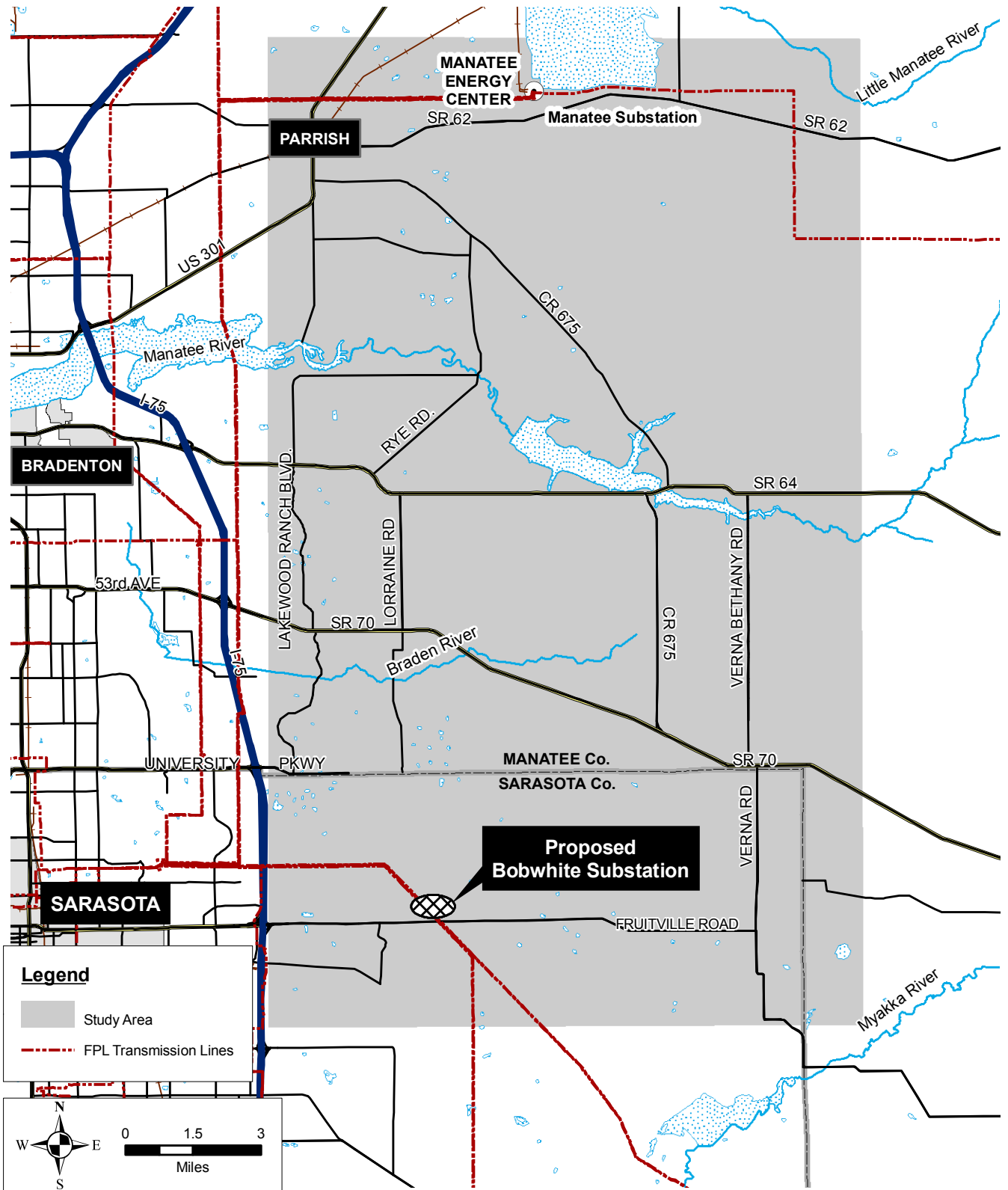
FIGURE 2.1-1. BOBWHITE-MANATEE 230-kV TRANSMISSION LINE PROJECT--STUDY AREA
