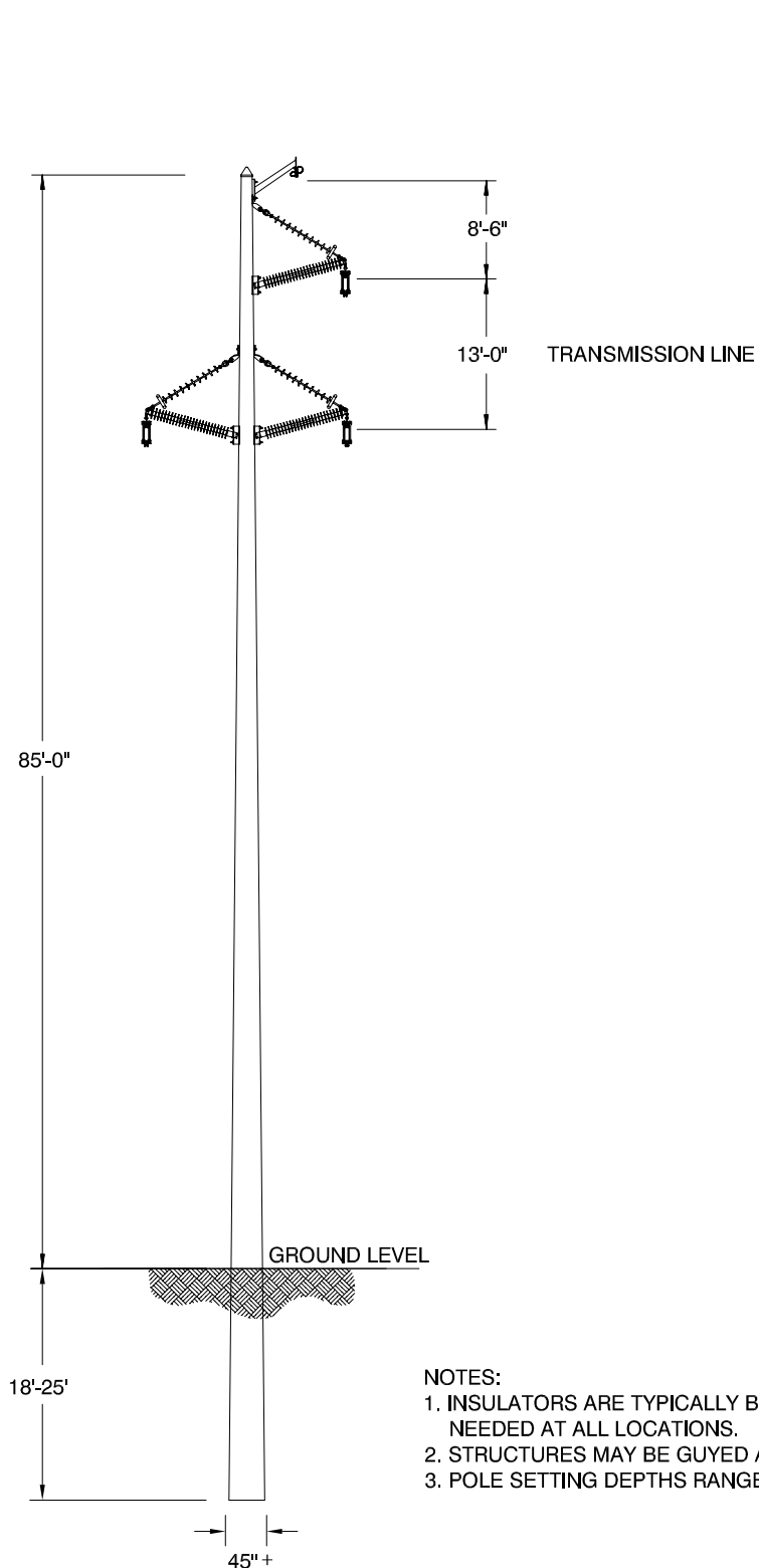
FIGURE 1.3-3. TYPICAL 85' TANGENT STRUCTURE TRIANGULAR CONFIGURATION WITHOUT DISTRIBUTION / COMMUNICATION UNDERBUILD
