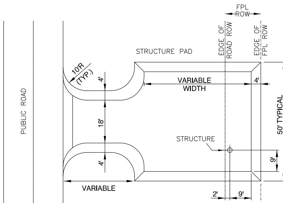
PLAN VIEW
