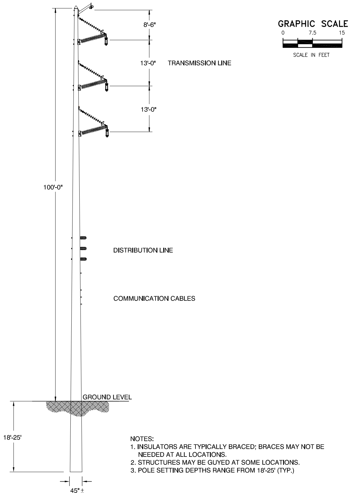
FIGURE 1.3-2. TYPICAL 100' TANGENT STRUCTURE VERTICAL CONFIGURATION WITH DISTRIBUTION / COMMUNICATION UNDERBUILD
