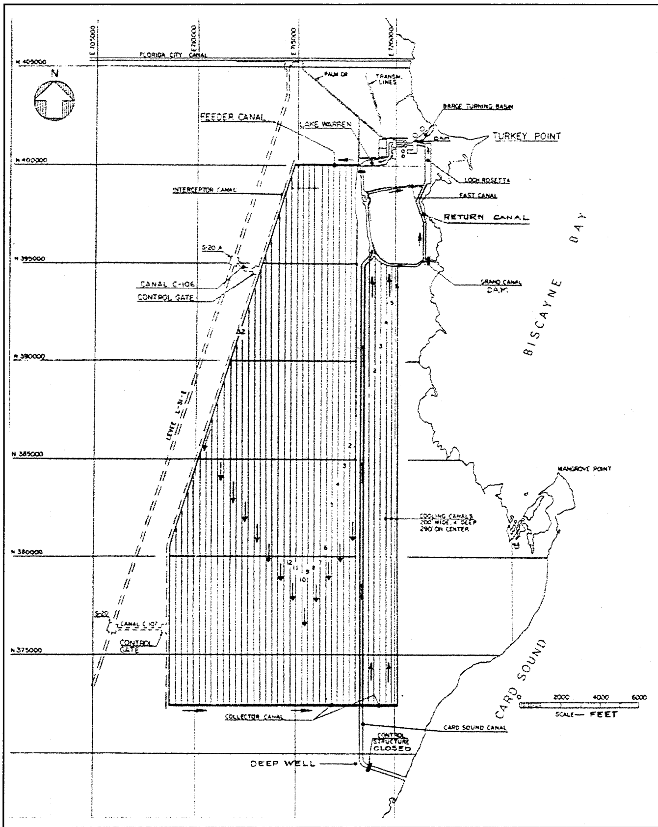
Figure 2.3-11. Turkey Point Cooling Canal System – Final Design
