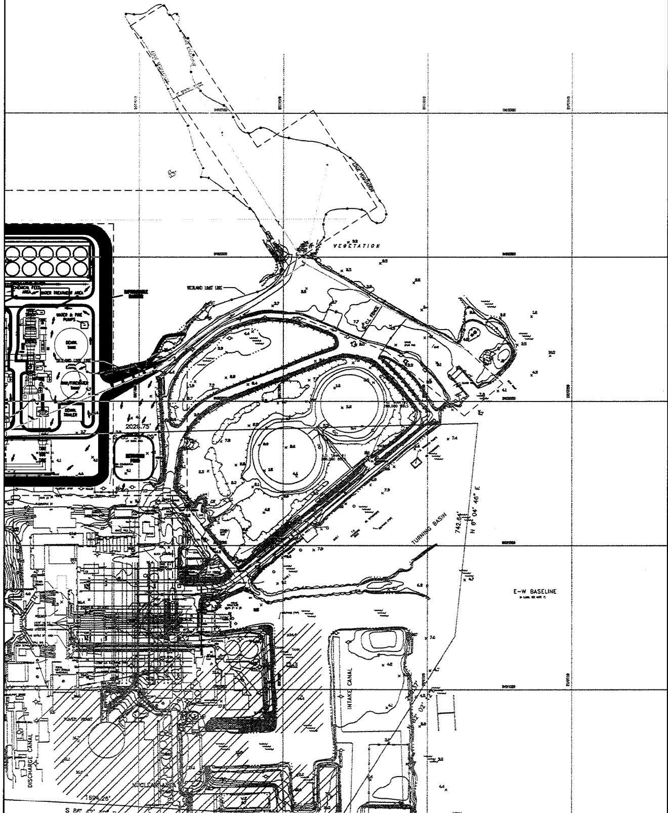
FIGURE 3.8-2 (Sheet 2 of 2) TURKEY POINT EXPANSION PROJECT - POST-CONSTRUCTION STORMWATER DRAINAGE
