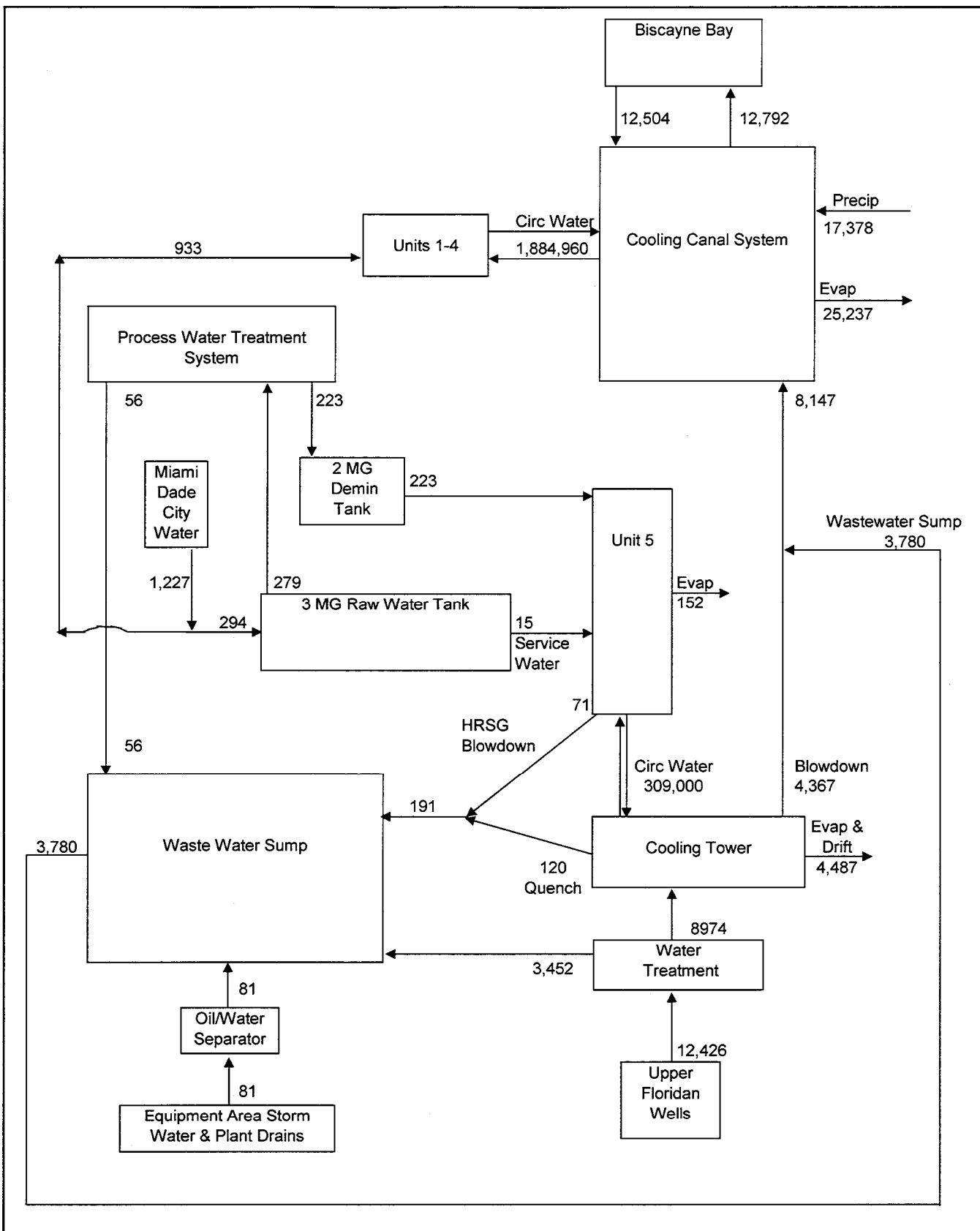
Figure 3.5-2 Special Water Use Diagram [flows in gpm]
