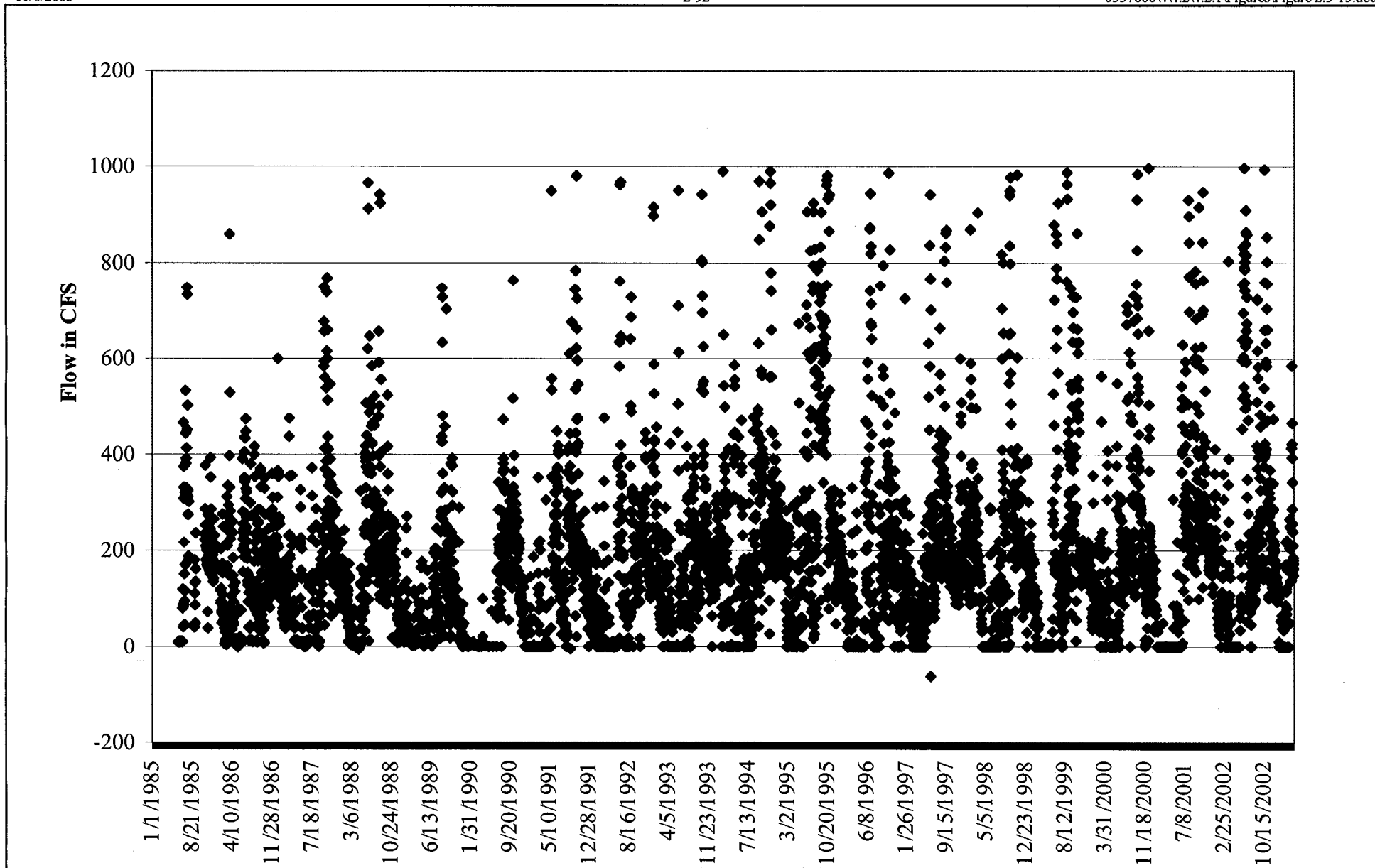
Figure 2.3-15. Flow at S-20F (1985-2002)
