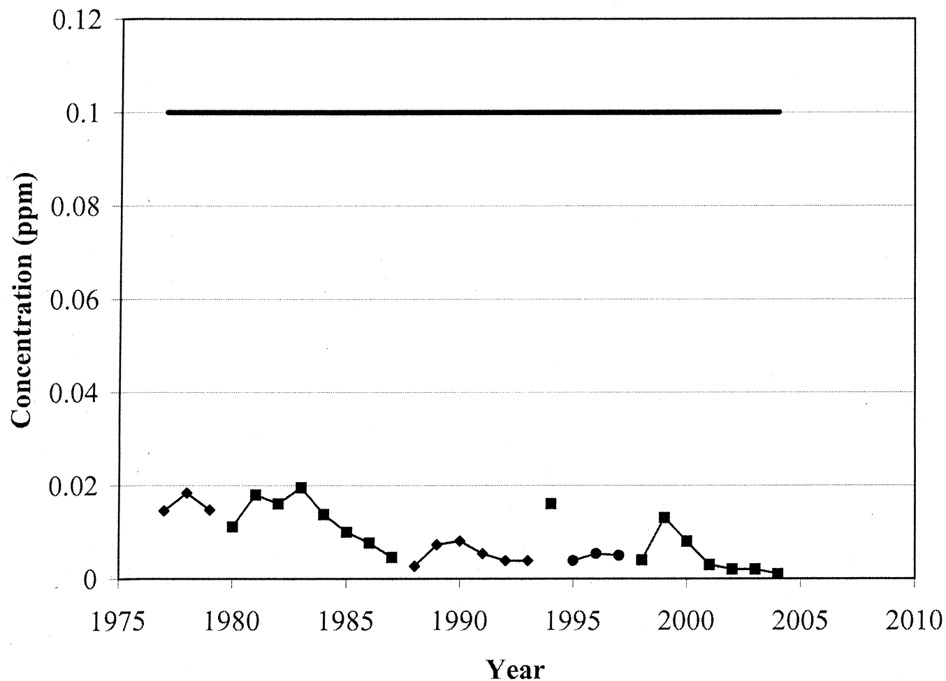
Figure 7-11. 24-hour Average Sulfur Dioxide Concentrations (2 nd Highest Values) Measured from 1977 to 2004- Palm Beach County
