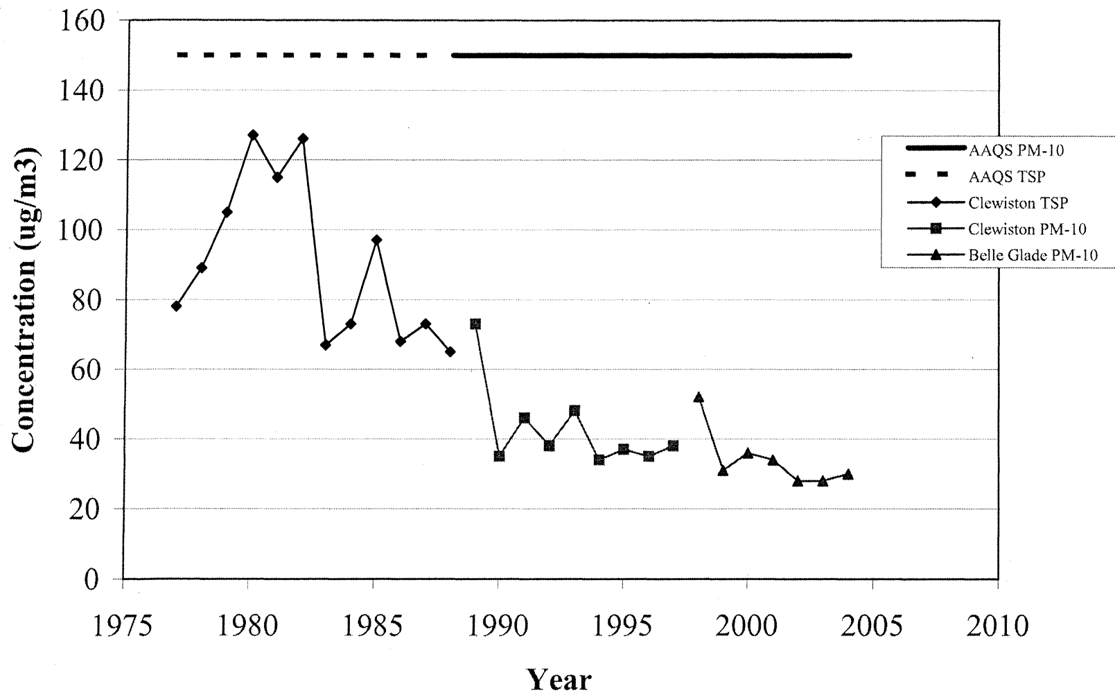
Figure 7-14. 24-hour Average PM 10 Concentrations and TSP Concentrations (2 nd Highest Values) Measured from 1977 to 2004- Hendry and Palm Beach Counties
