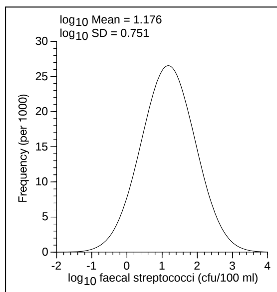
Figure C-1. A Probability Density Function of Fecal Indicator Distributions Measured at a Recreational Water Showing Probability of Exposure (Y Axis) versus Log 10 Faecal Streptococci Concentration (later termed enterococci).
