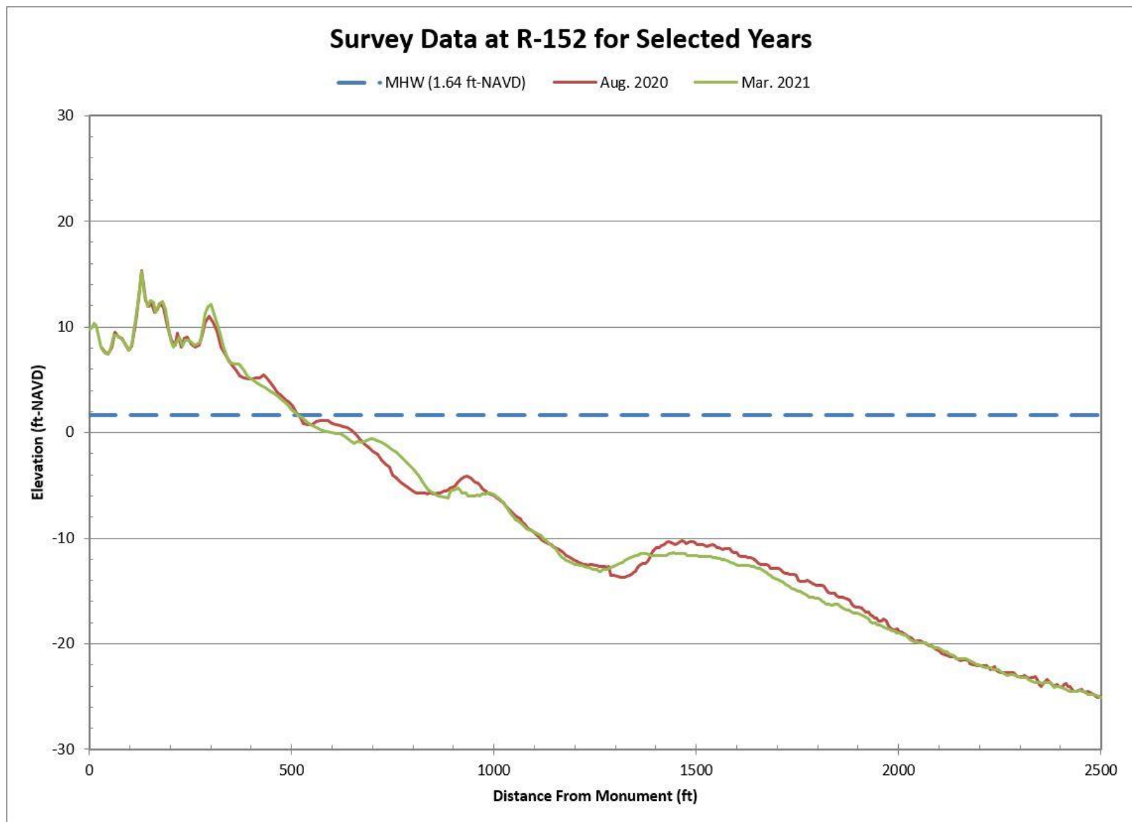
Figure B-76. Aug. 2020 Pre-Construction vs. Mar. 2021 Post-Construction Beach Profiles Along R-152
