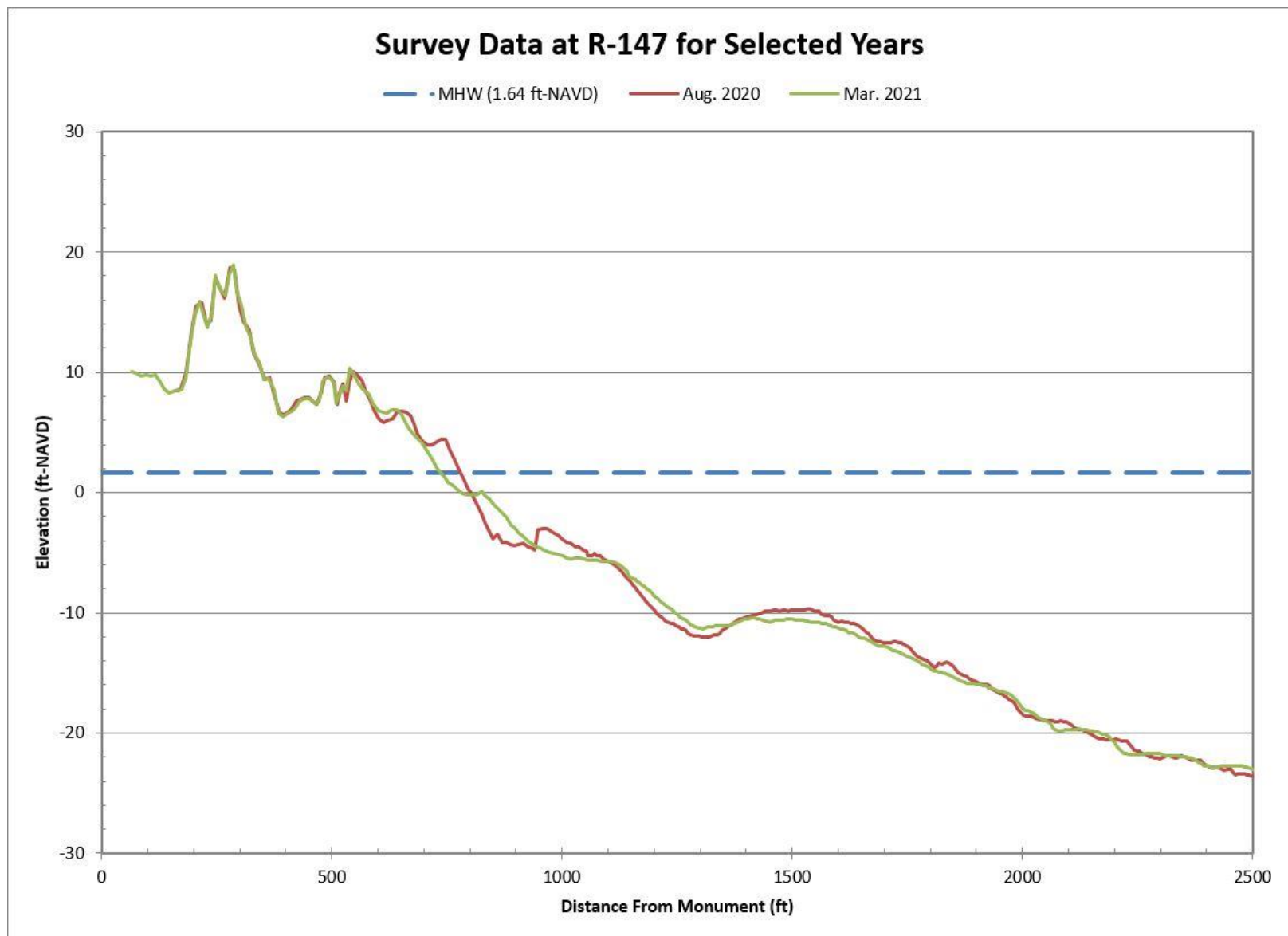
Figure B-71. Aug. 2020 Pre-Construction vs. Mar. 2021 Post-Construction Beach Profiles Along R-147
