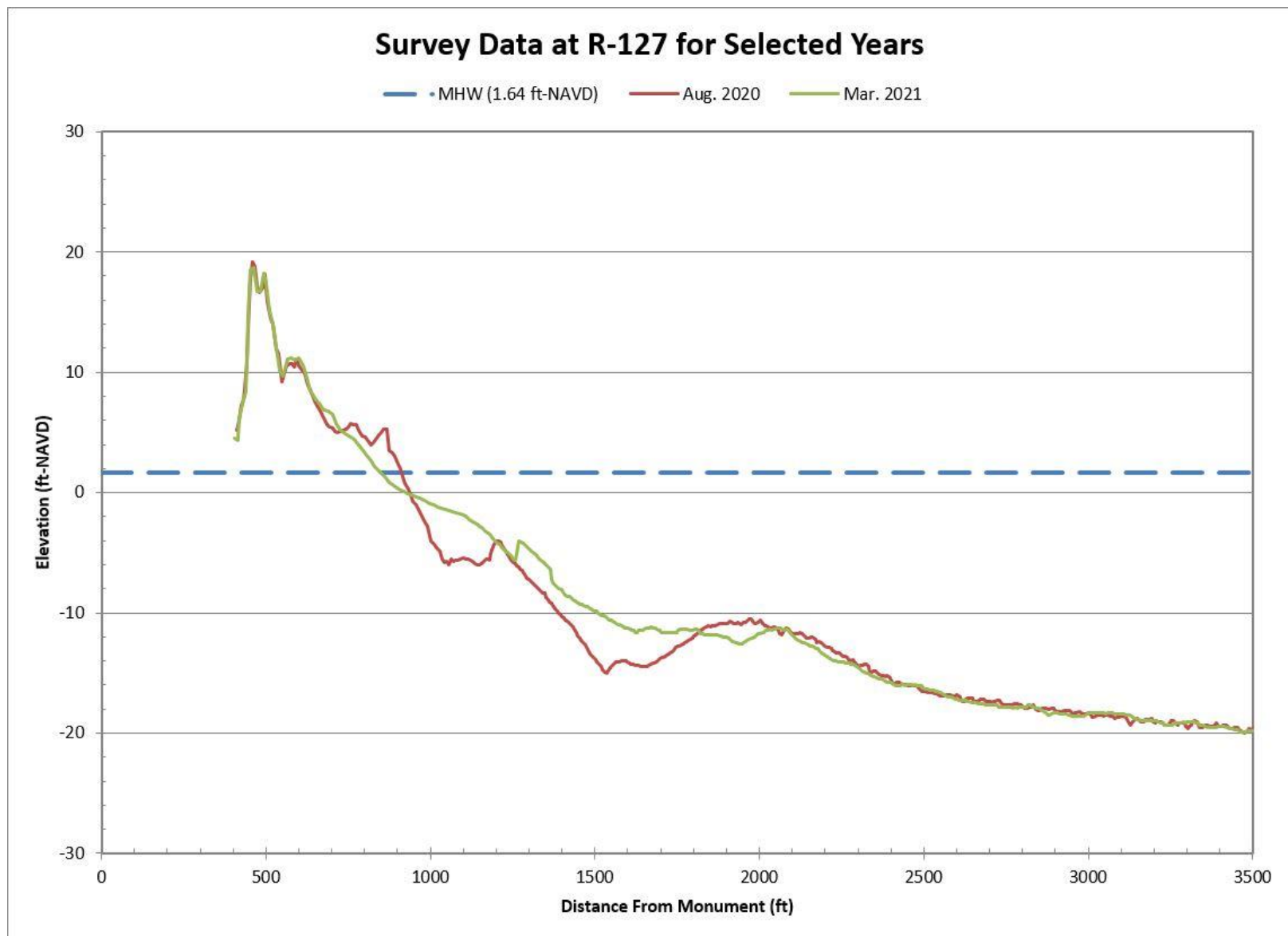
Figure B-51. Aug. 2020 Pre-Construction vs. Mar. 2021 Post-Construction Beach Profiles Along R-127
