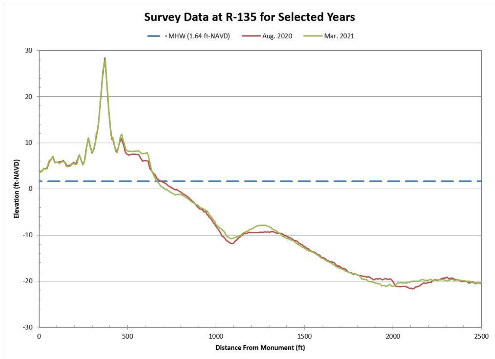
Figure B-59. Aug. 2020 Pre-Construction vs. Mar. 2021 Post-Construction Beach Profiles Along R-135
