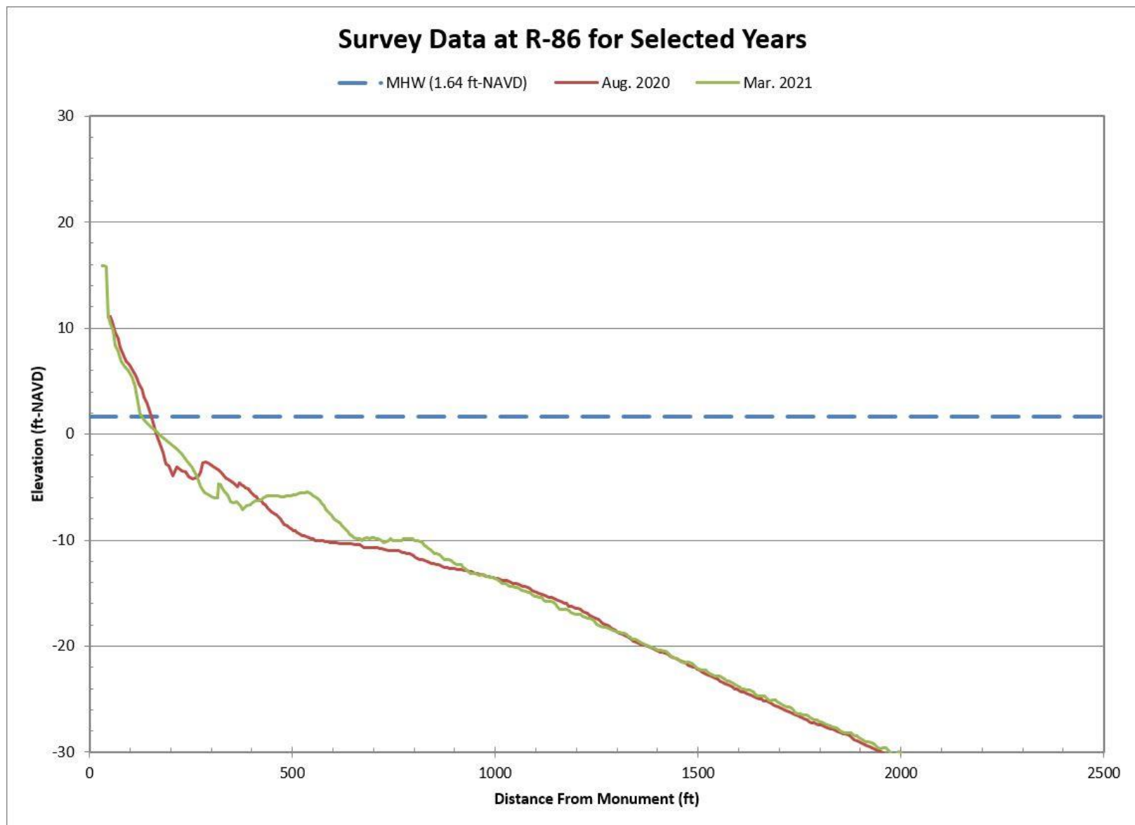
Figure B-7. Aug. 2020 Pre-Construction vs. Mar. 2021 Post-Construction Beach Profiles Along R-86
