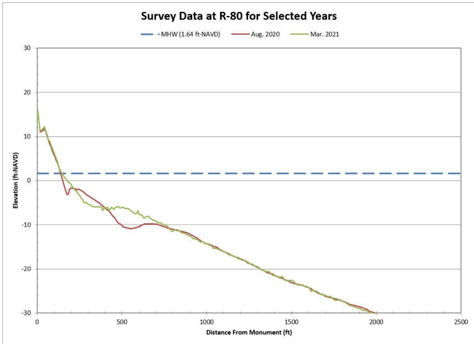
Figure B-1. Aug. 2020 Pre-Construction vs. Mar. 2021 Post-Construction Beach Profiles Along R-80
