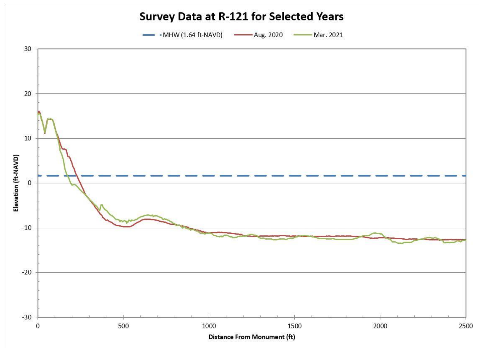
Figure B-42. Aug. 2020 Pre-Construction vs. Mar. 2021 Post-Construction Beach Profiles Along R-121
