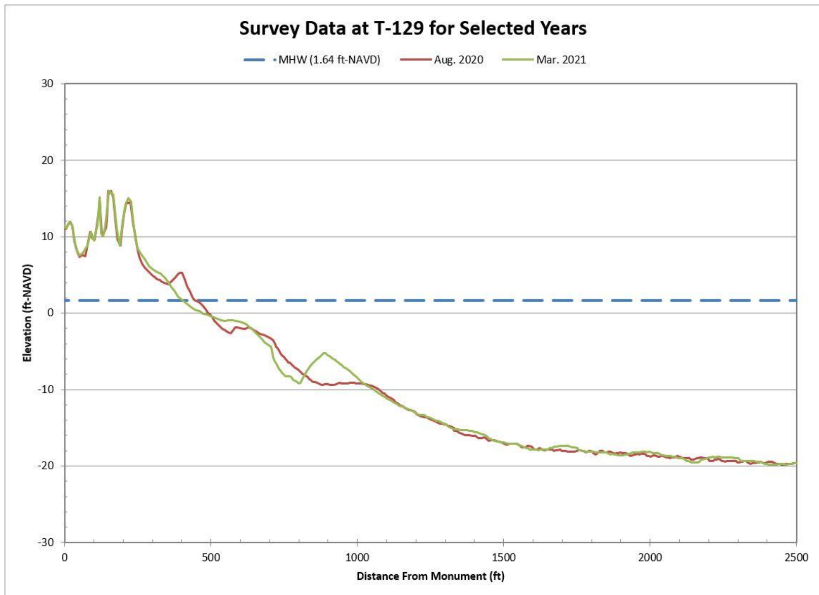
Figure B-53. Aug. 2020 Pre-Construction vs. Mar. 2021 Post-Construction Beach Profiles Along T-129
