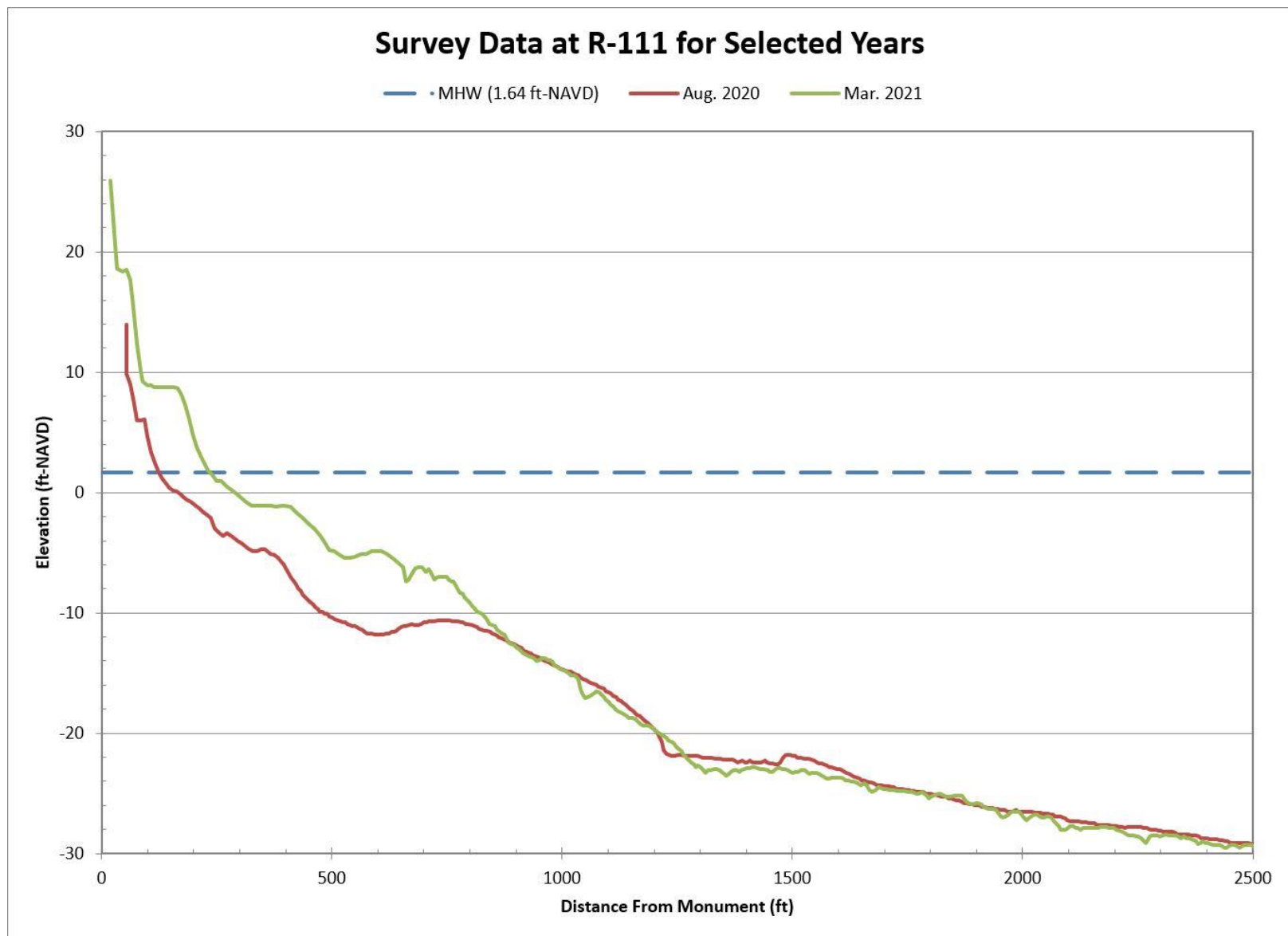
Figure B-32. Aug. 2020 Pre-Construction vs. Mar. 2021 Post-Construction Beach Profiles Along R-111
