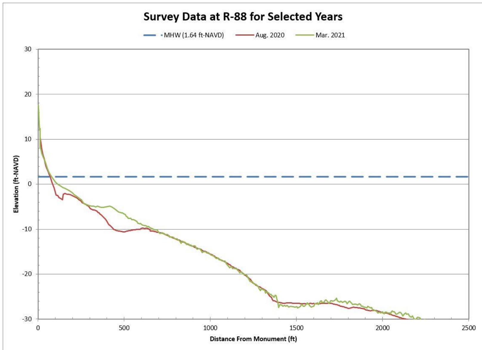
Figure B-9. Aug. 2020 Pre-Construction vs. Mar. 2021 Post-Construction Beach Profiles Along R-88
