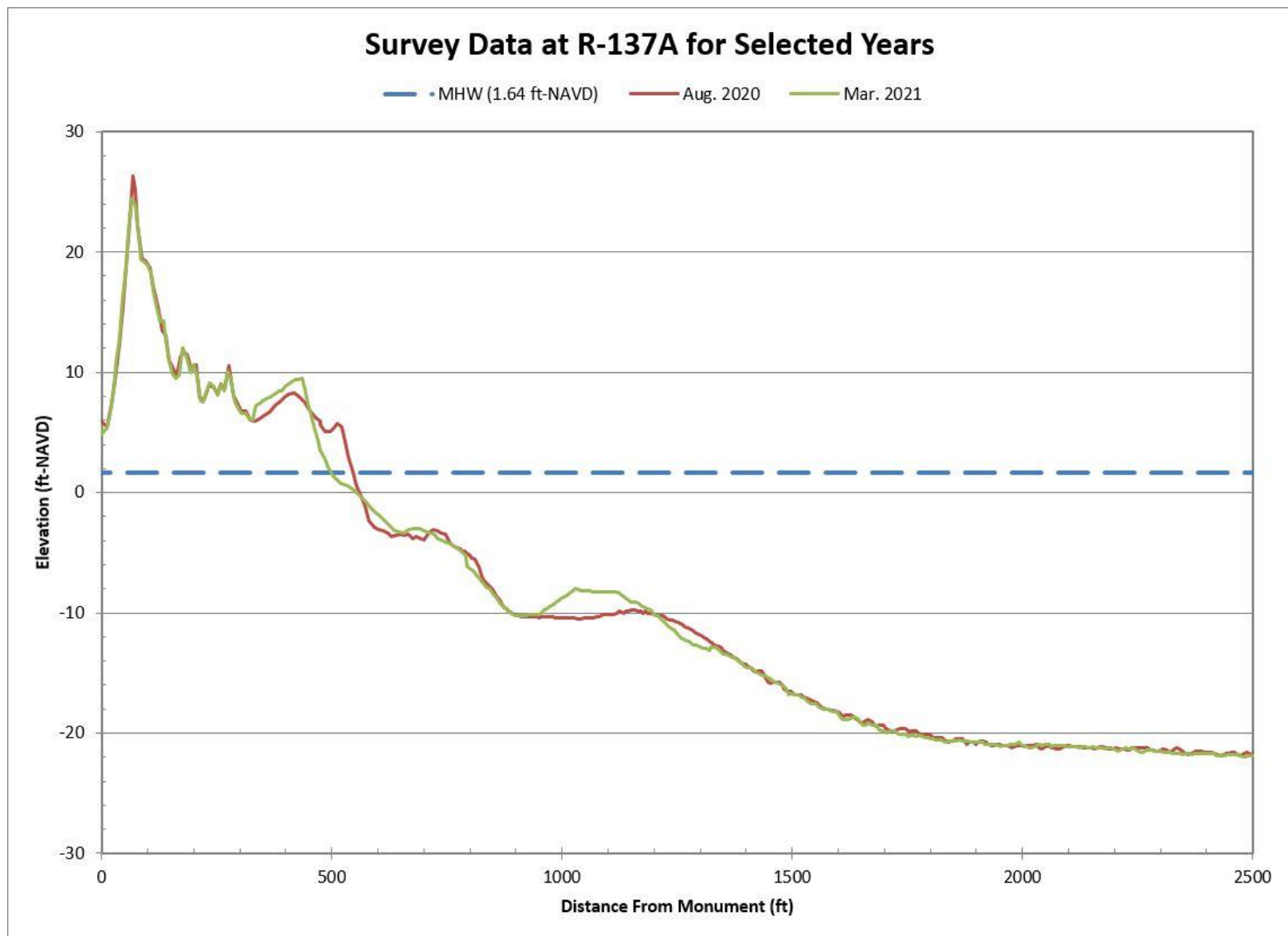
Figure B-61. Aug. 2020 Pre-Construction vs. Mar. 2021 Post-Construction Beach Profiles Along R-137A
