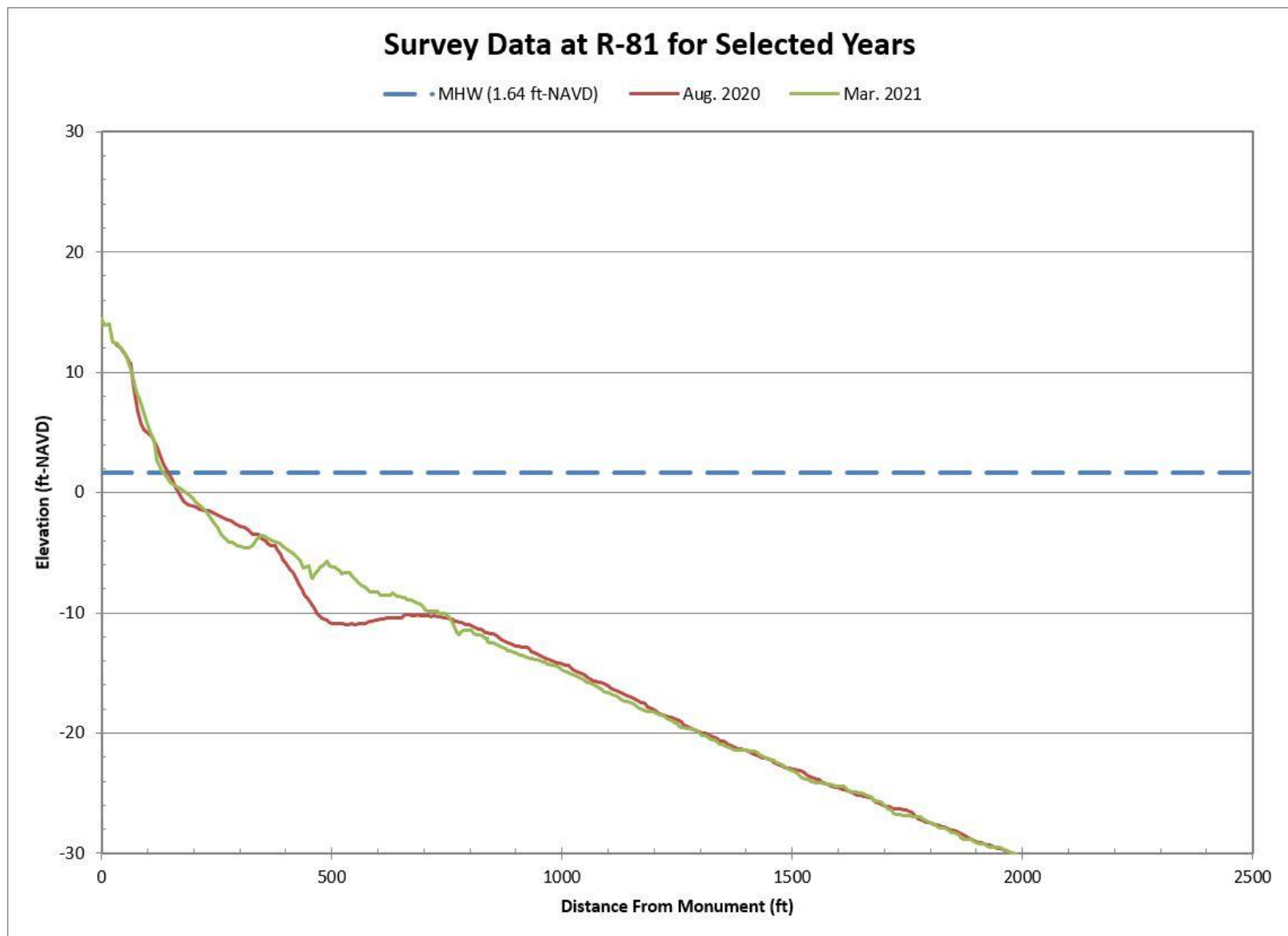
Figure B-2. Aug. 2020 Pre-Construction vs. Mar. 2021 Post-Construction Beach Profiles Along R-81
