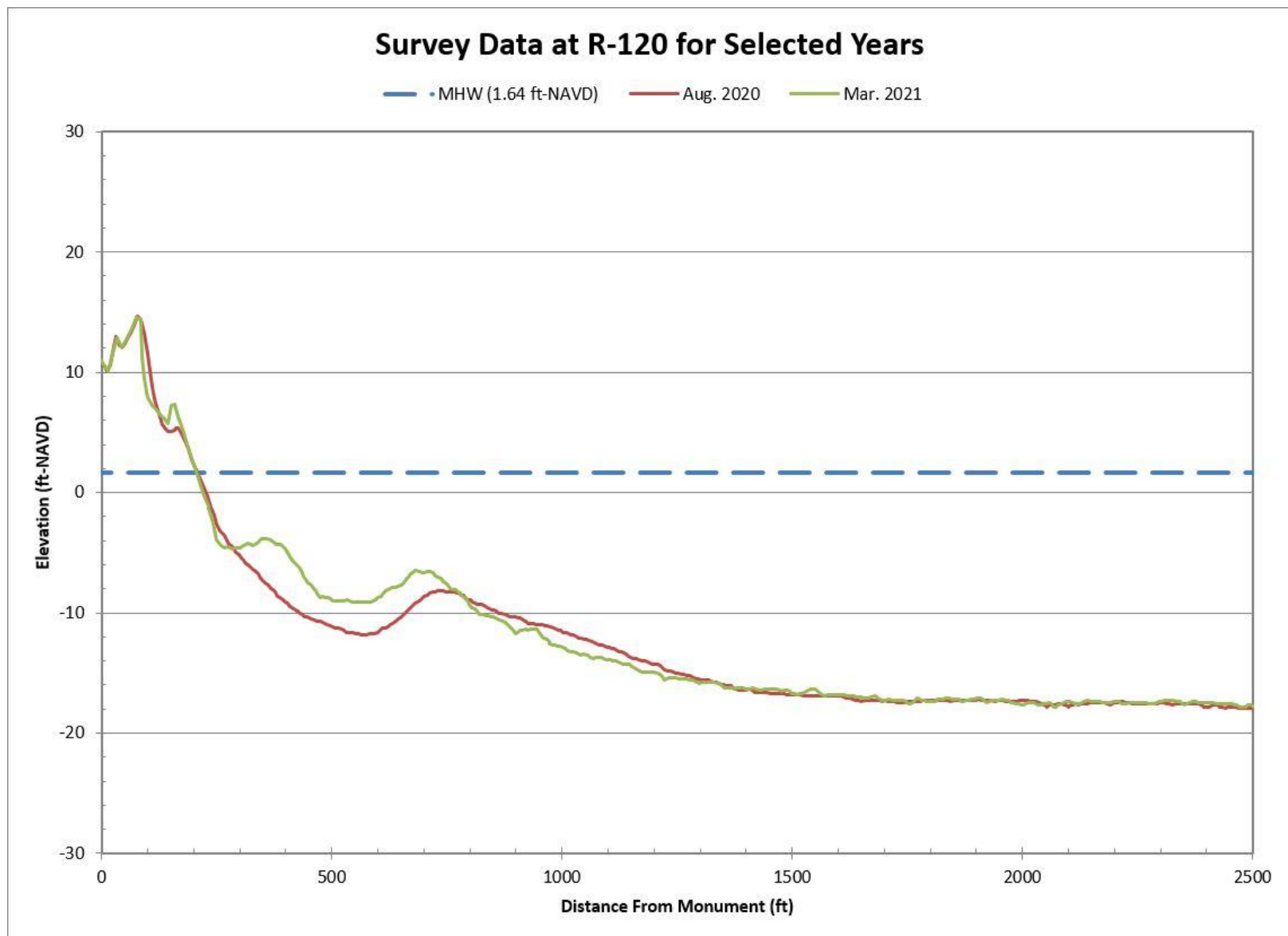
Figure B-41. Aug. 2020 Pre-Construction vs. Mar. 2021 Post-Construction Beach Profiles Along R-120
