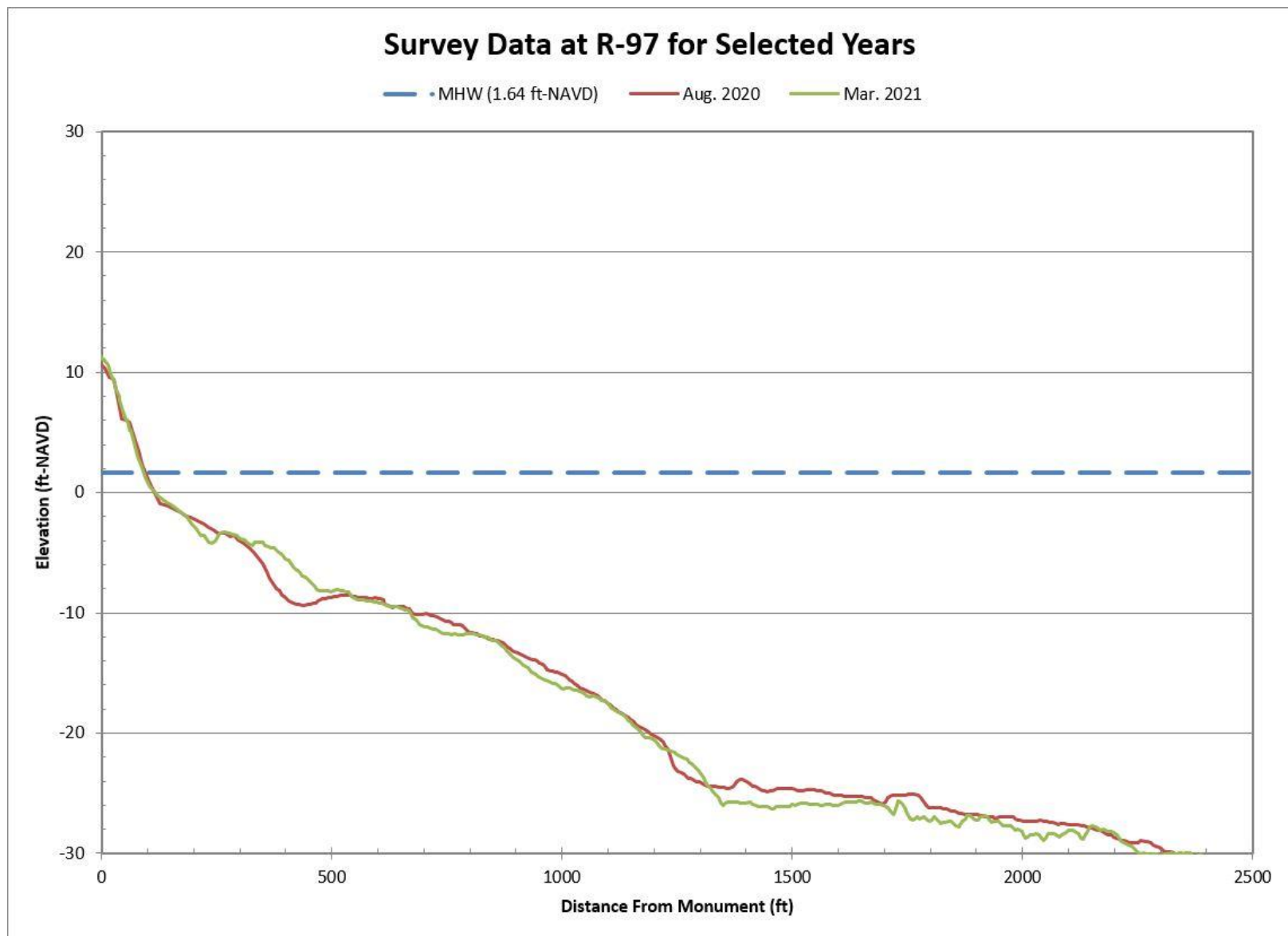
Figure B-18. Aug. 2020 Pre-Construction vs. Mar. 2021 Post-Construction Beach Profiles Along R-97
