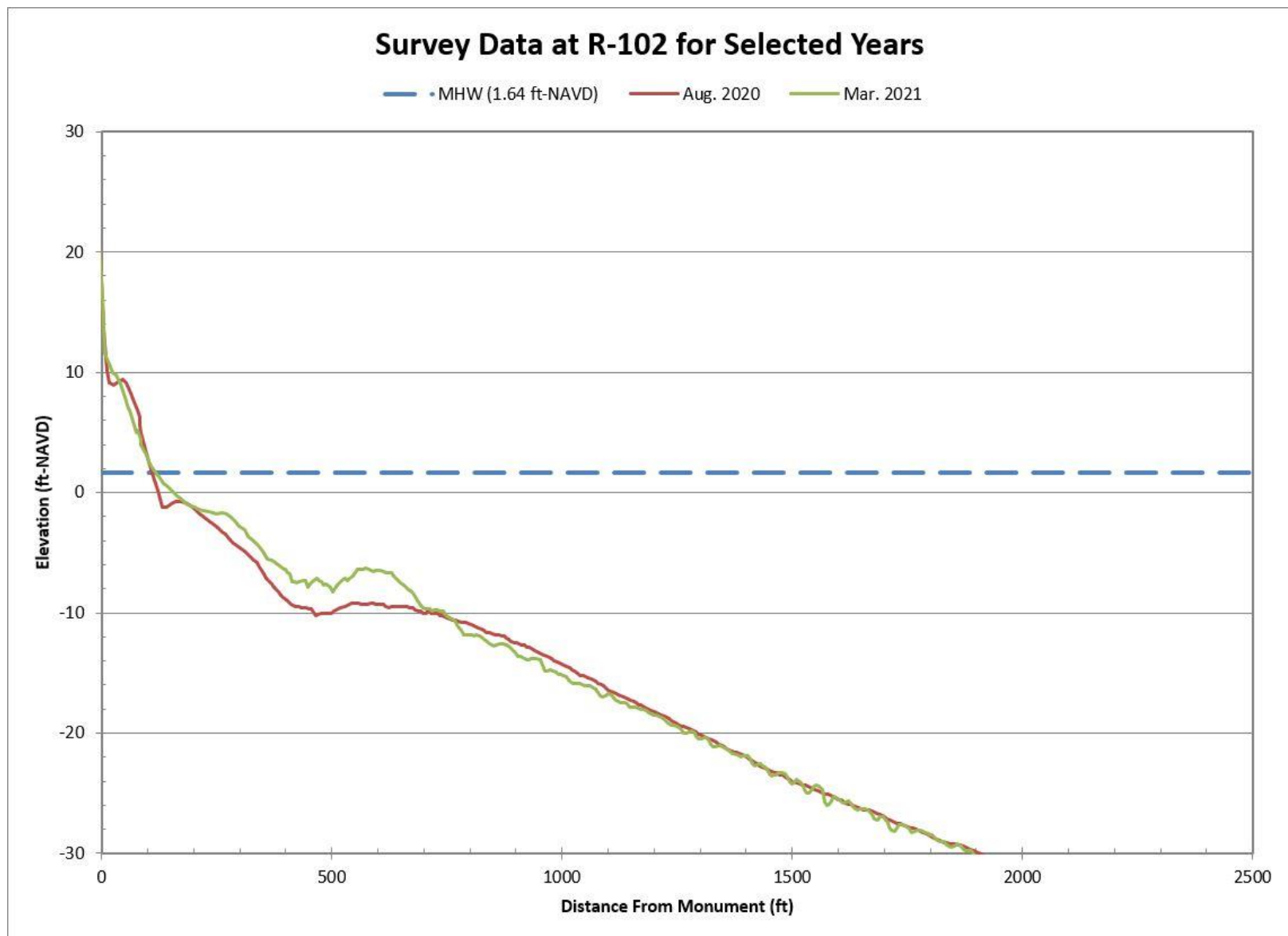
Figure B-23. Aug. 2020 Pre-Construction vs. Mar. 2021 Post-Construction Beach Profiles Along R-102
