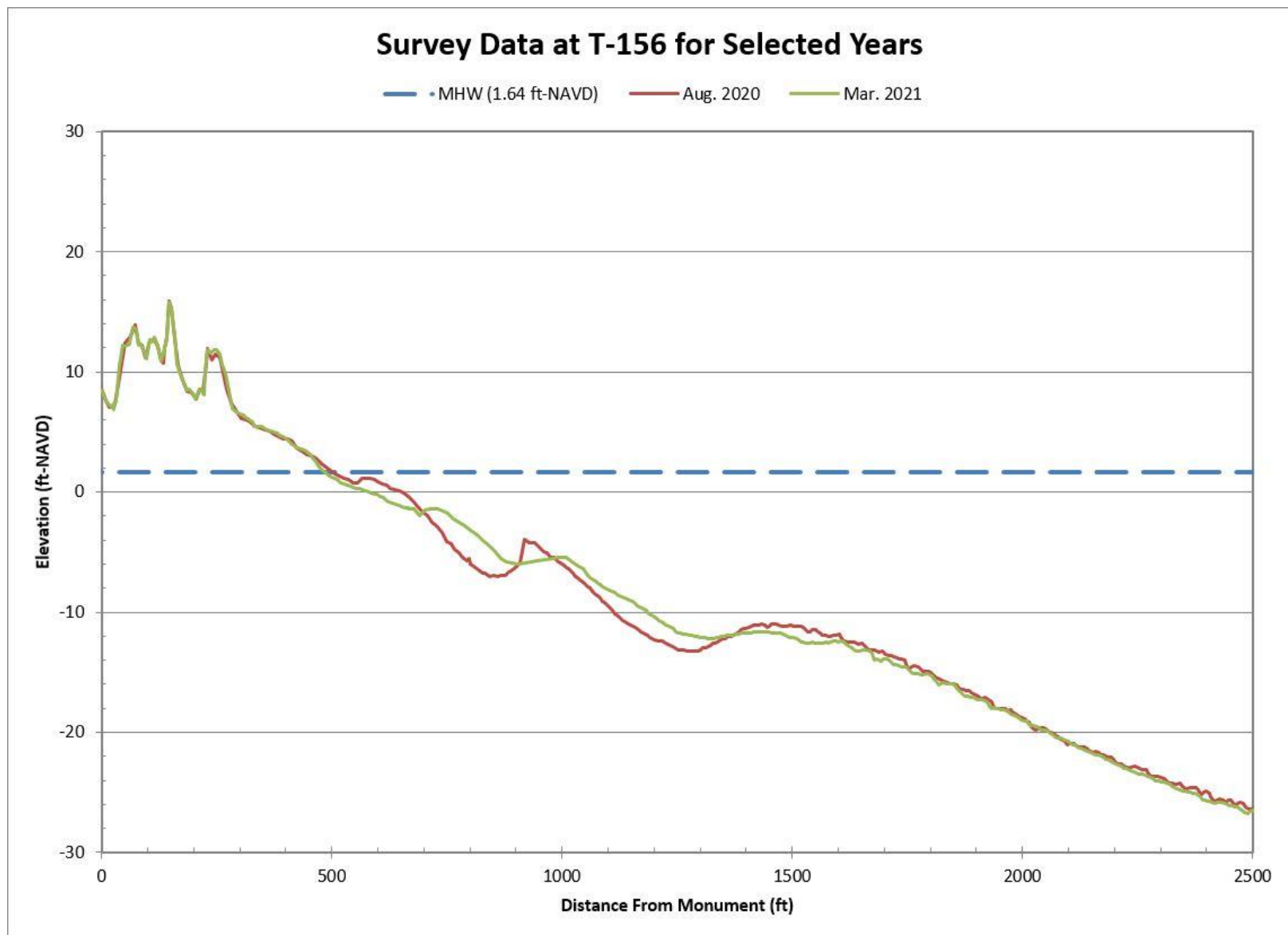
Figure B-80. Aug. 2020 Pre-Construction vs. Mar. 2021 Post-Construction Beach Profiles Along T-156
