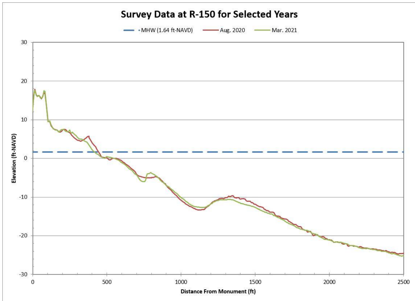
Figure B-74. Aug. 2020 Pre-Construction vs. Mar. 2021 Post-Construction Beach Profiles Along R-150
