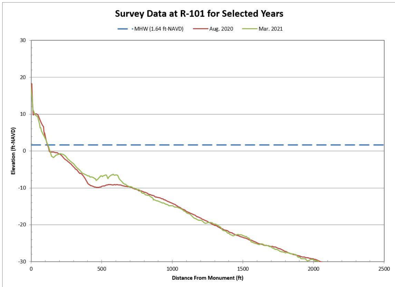
Figure B-22. Aug. 2020 Pre-Construction vs. Mar. 2021 Post-Construction Beach Profiles Along R-101
