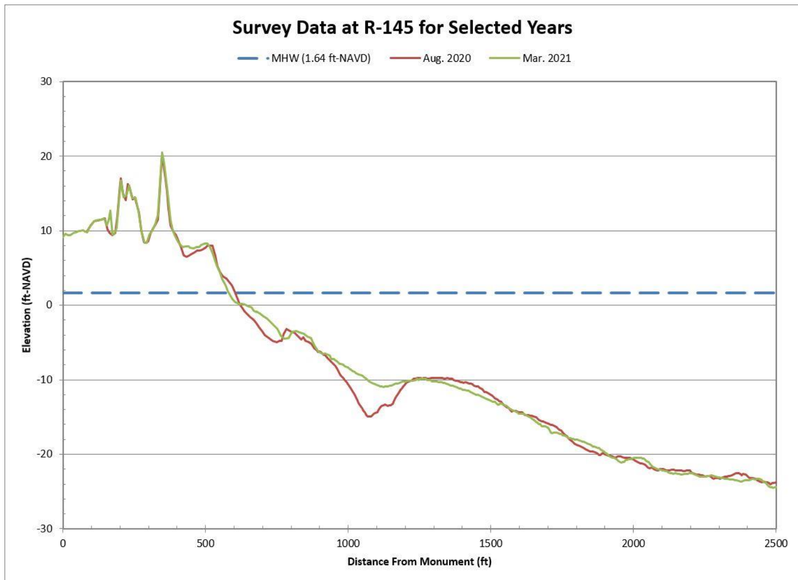
Figure B-69. Aug. 2020 Pre-Construction vs. Mar. 2021 Post-Construction Beach Profiles Along R-145
