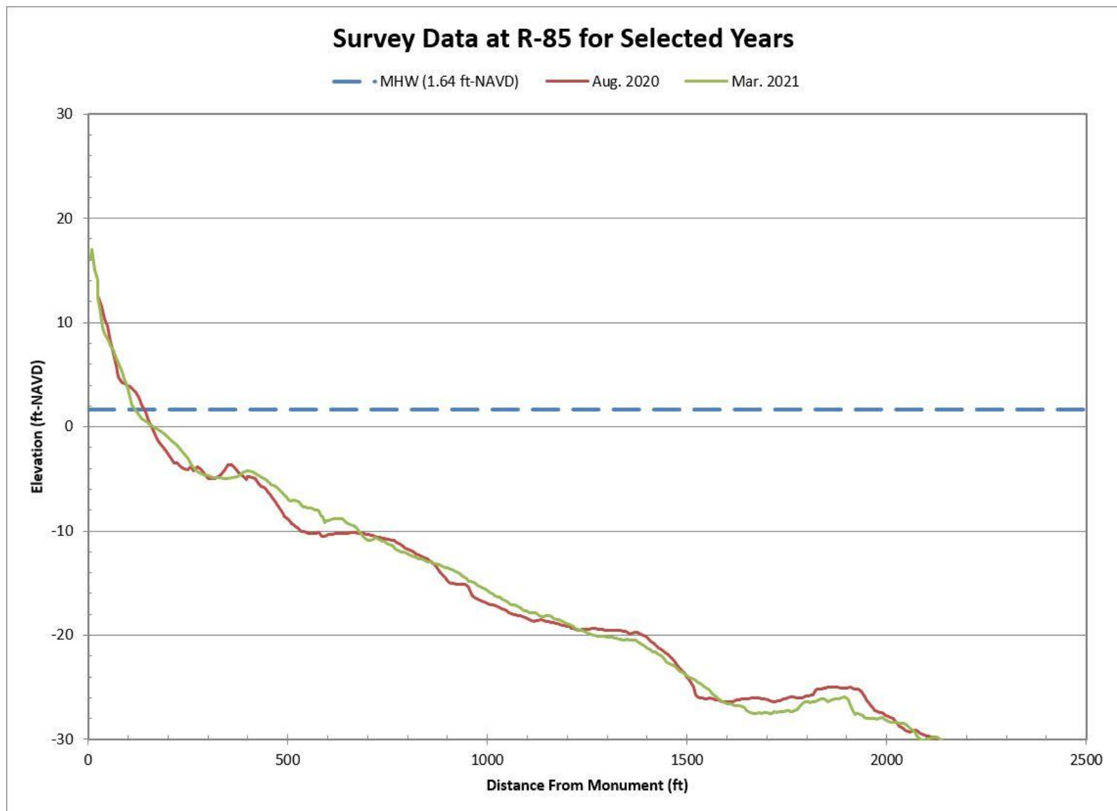
Figure B-6. Aug. 2020 Pre-Construction vs. Mar. 2021 Post-Construction Beach Profiles Along R-85
