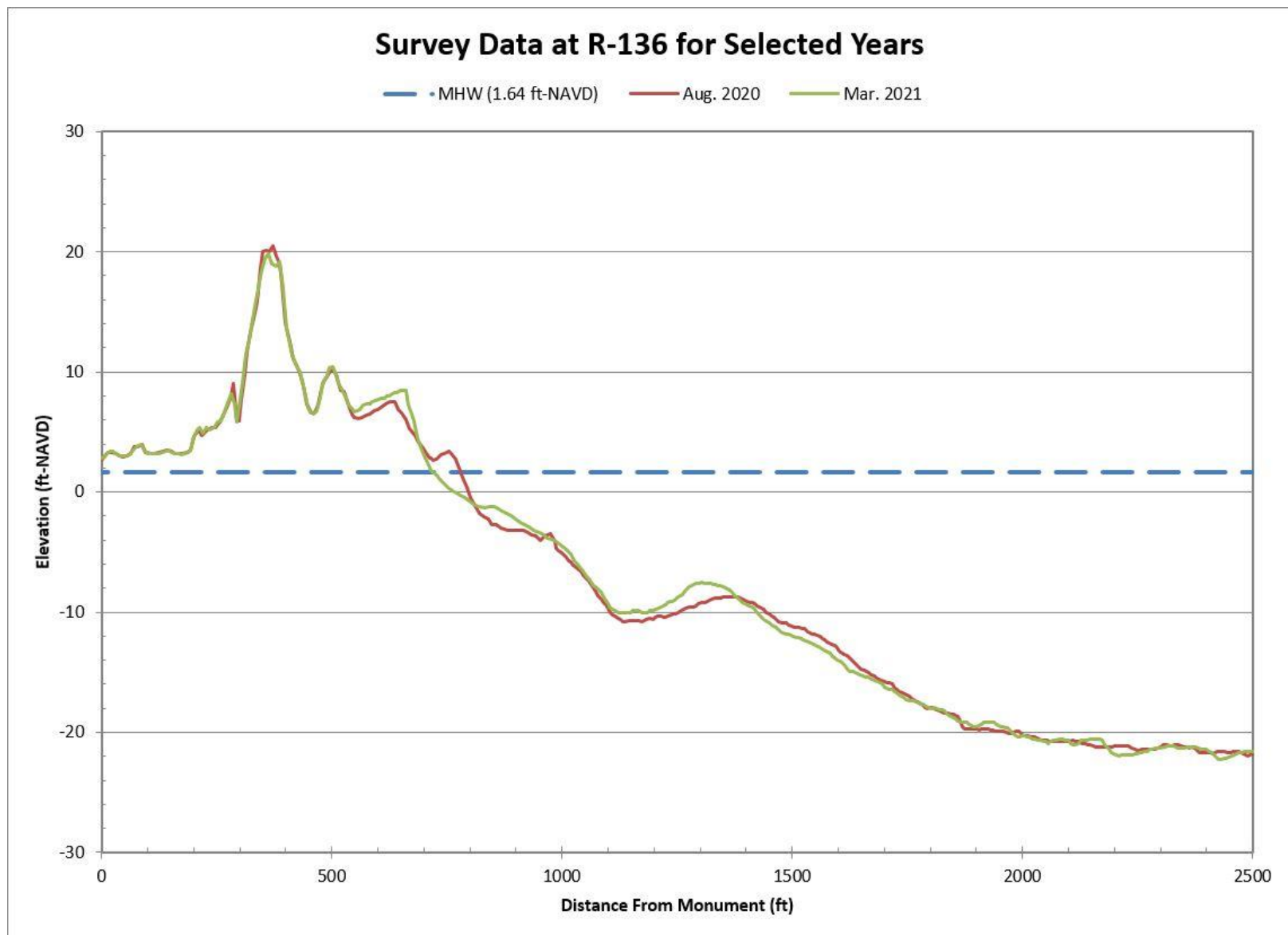
Figure B-60. Aug. 2020 Pre-Construction vs. Mar. 2021 Post-Construction Beach Profiles Along R-136
