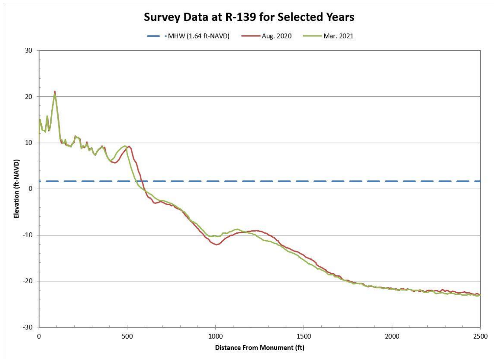
Figure B-63. Aug. 2020 Pre-Construction vs. Mar. 2021 Post-Construction Beach Profiles Along R-139
