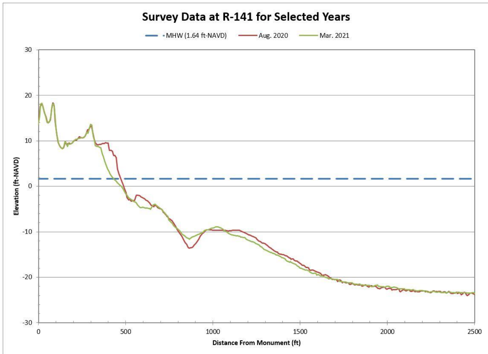
Figure B-65. Aug. 2020 Pre-Construction vs. Mar. 2021 Post-Construction Beach Profiles Along R-141
