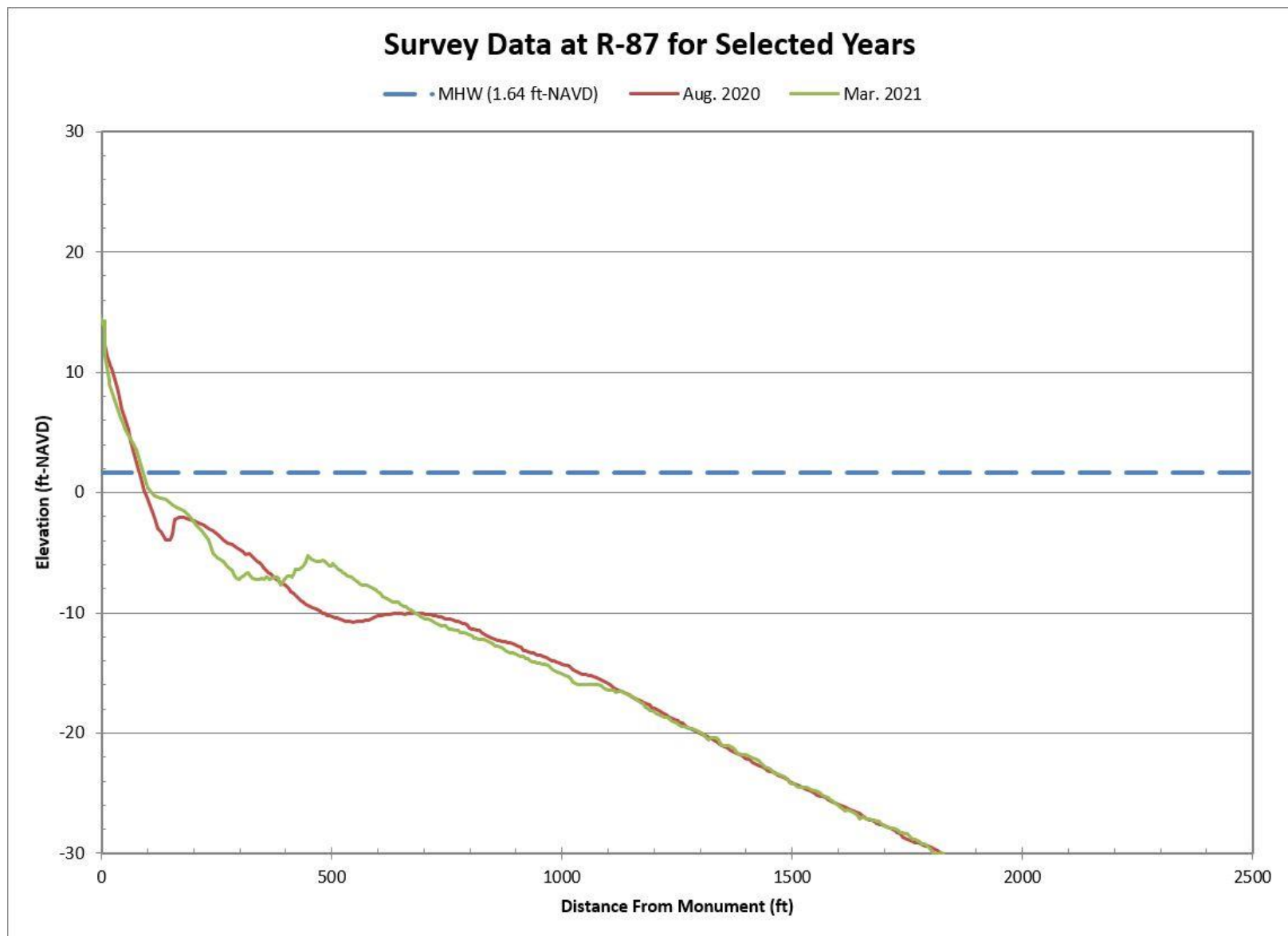
Figure B-8. Aug. 2020 Pre-Construction vs. Mar. 2021 Post-Construction Beach Profiles Along R-87
