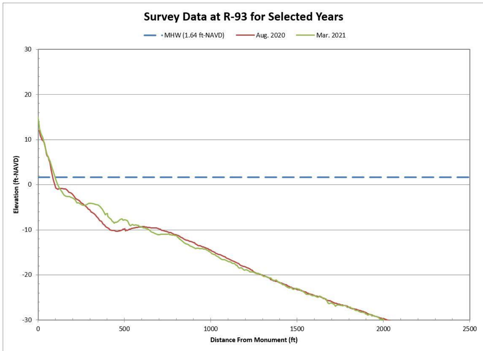
Figure B-14. Aug. 2020 Pre-Construction vs. Mar. 2021 Post-Construction Beach Profiles Along R-93
