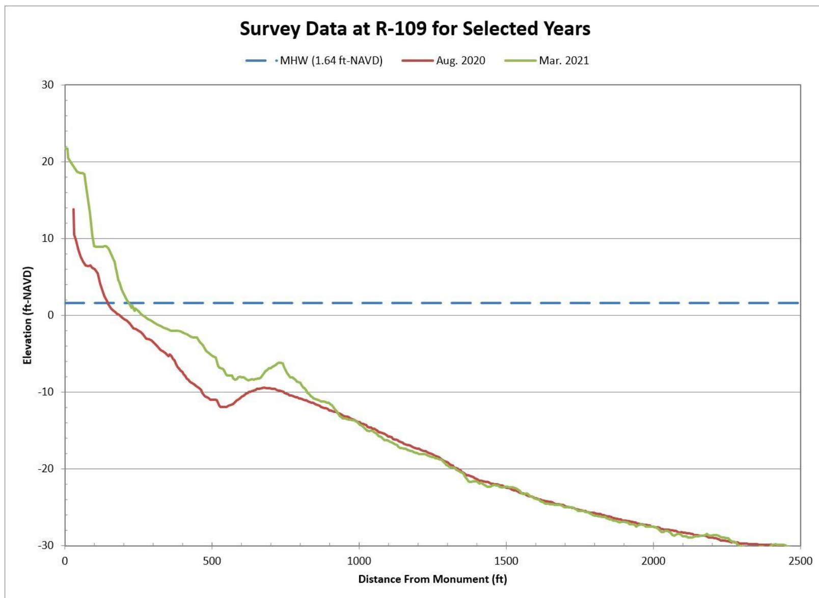
Figure B-30. Aug. 2020 Pre-Construction vs. Mar. 2021 Post-Construction Beach Profiles Along R-109
