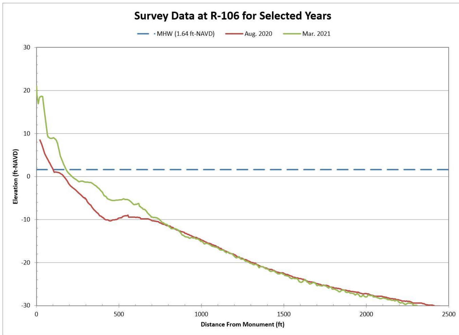
Figure B-27. Aug. 2020 Pre-Construction vs. Mar. 2021 Post-Construction Beach Profiles Along R-106
