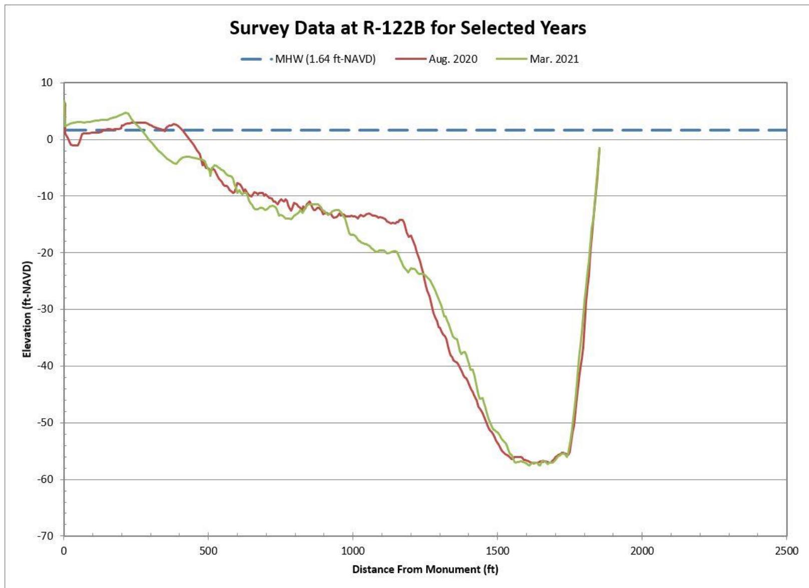
Figure B-45. Aug. 2020 Pre-Construction vs. Mar. 2021 Post-Construction Beach Profiles Along R-122B
