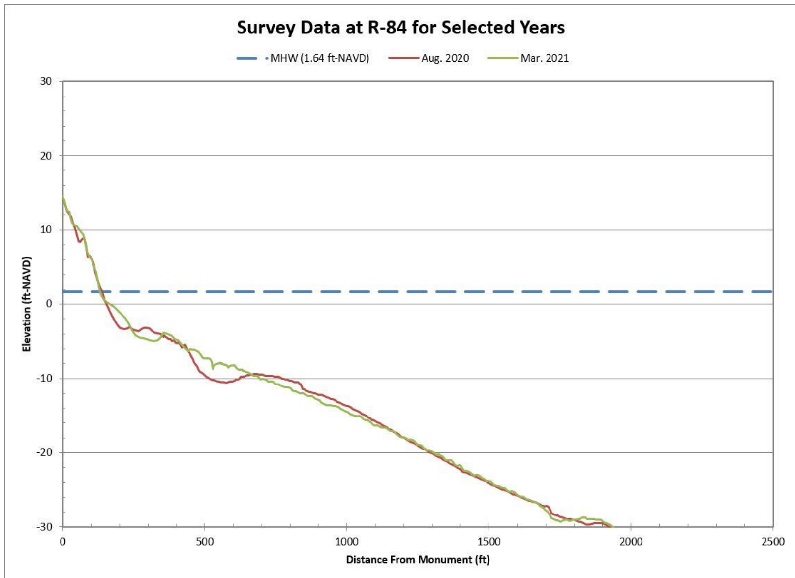
Figure B-5. Aug. 2020 Pre-Construction vs. Mar. 2021 Post-Construction Beach Profiles Along R-84
