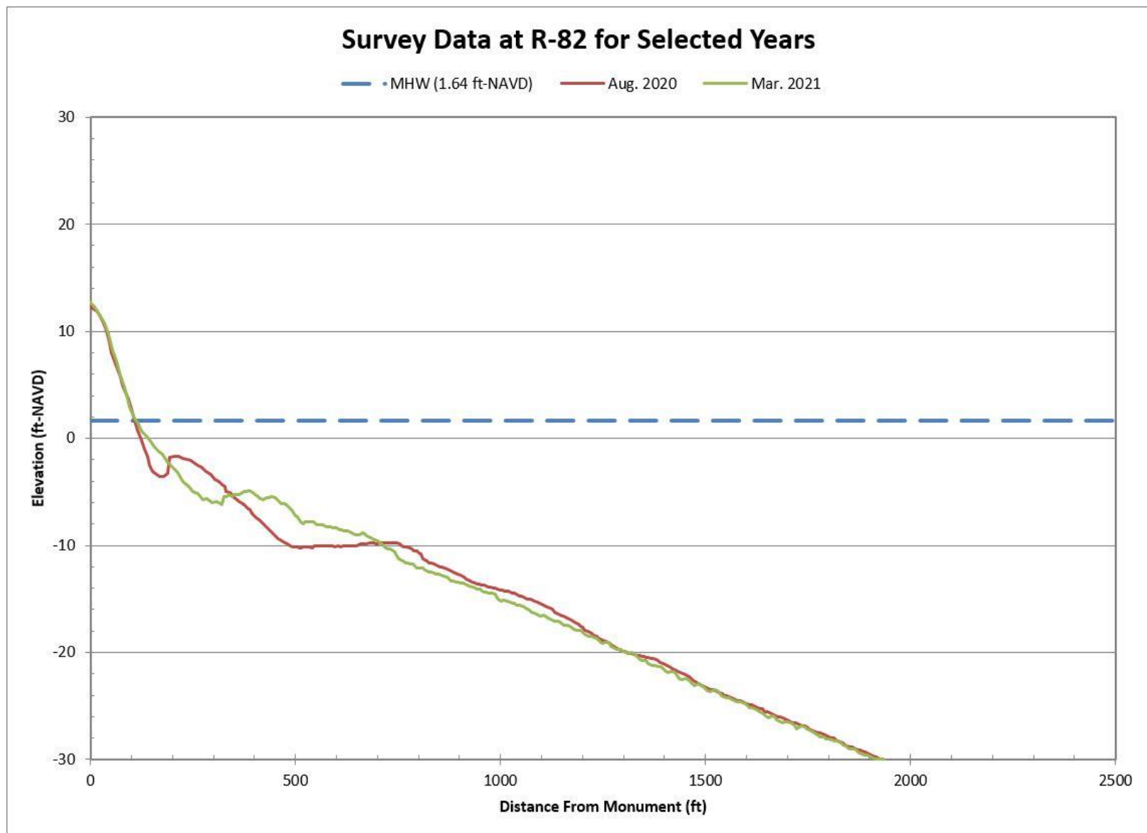
Figure B-3. Aug. 2020 Pre-Construction vs. Mar. 2021 Post-Construction Beach Profiles Along R-82
