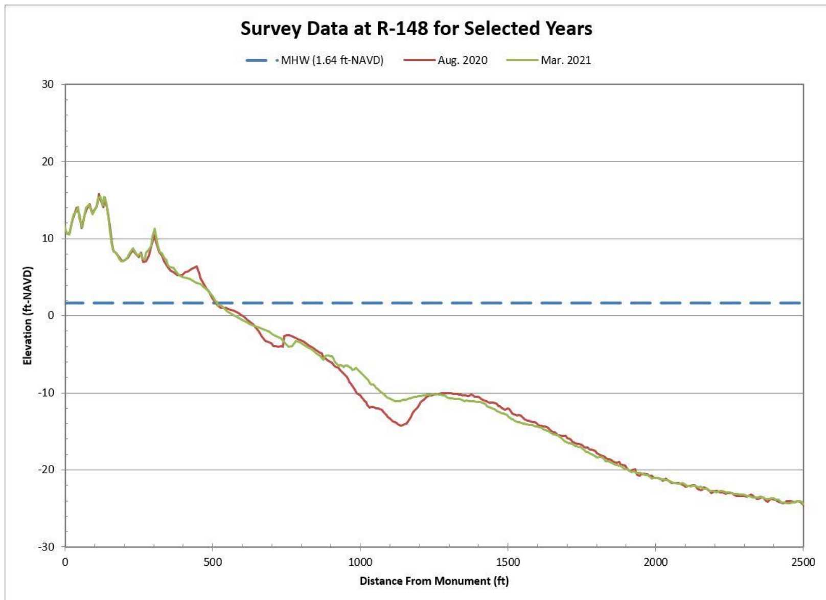
Figure B-72. Aug. 2020 Pre-Construction vs. Mar. 2021 Post-Construction Beach Profiles Along R-148
