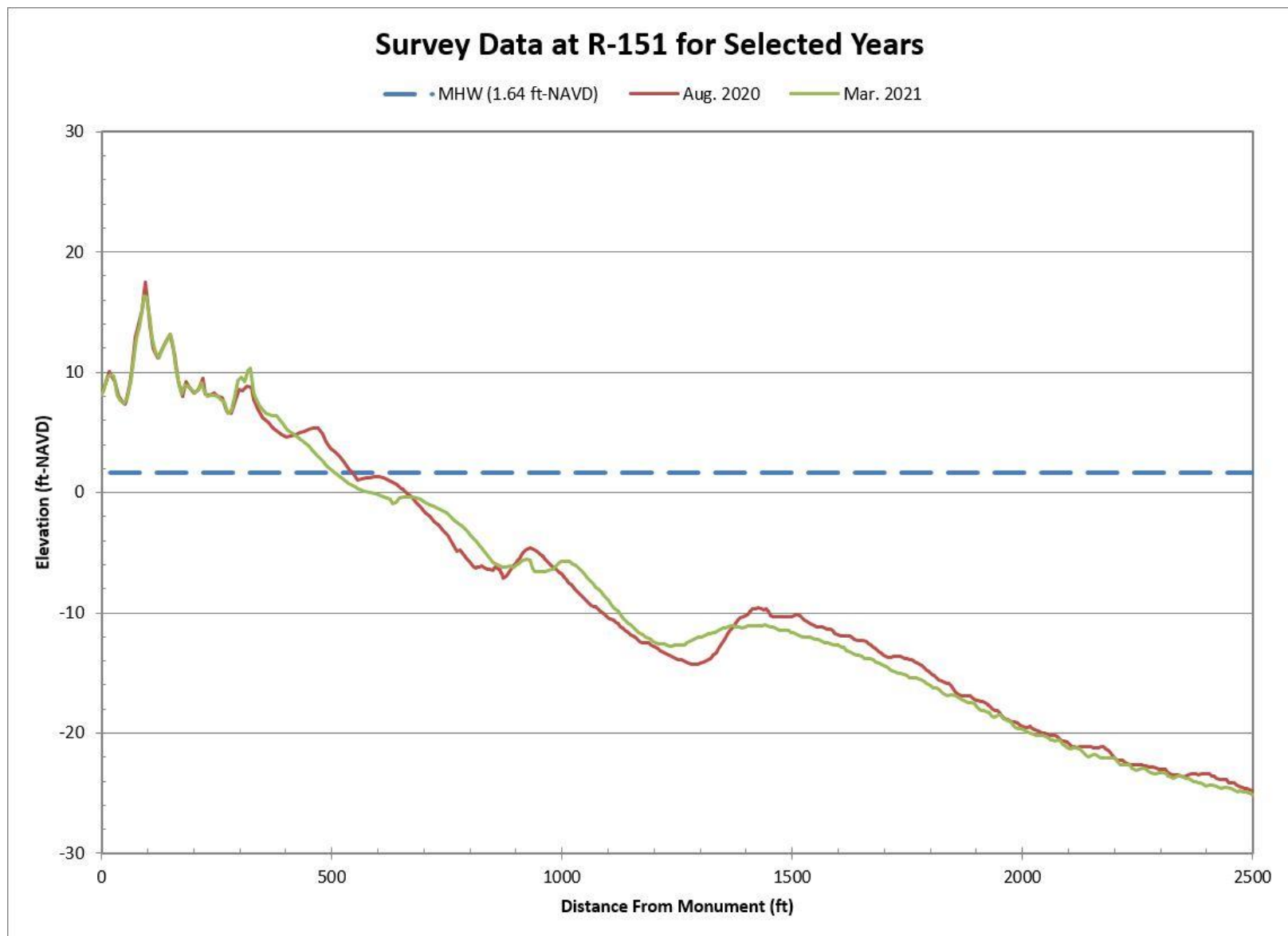
Figure B-75. Aug. 2020 Pre-Construction vs. Mar. 2021 Post-Construction Beach Profiles Along R-151
