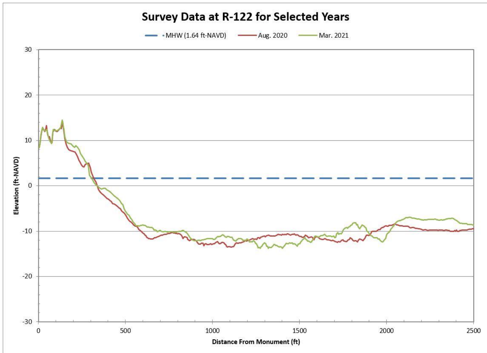
Figure B-43. Aug. 2020 Pre-Construction vs. Mar. 2021 Post-Construction Beach Profiles Along R-122
