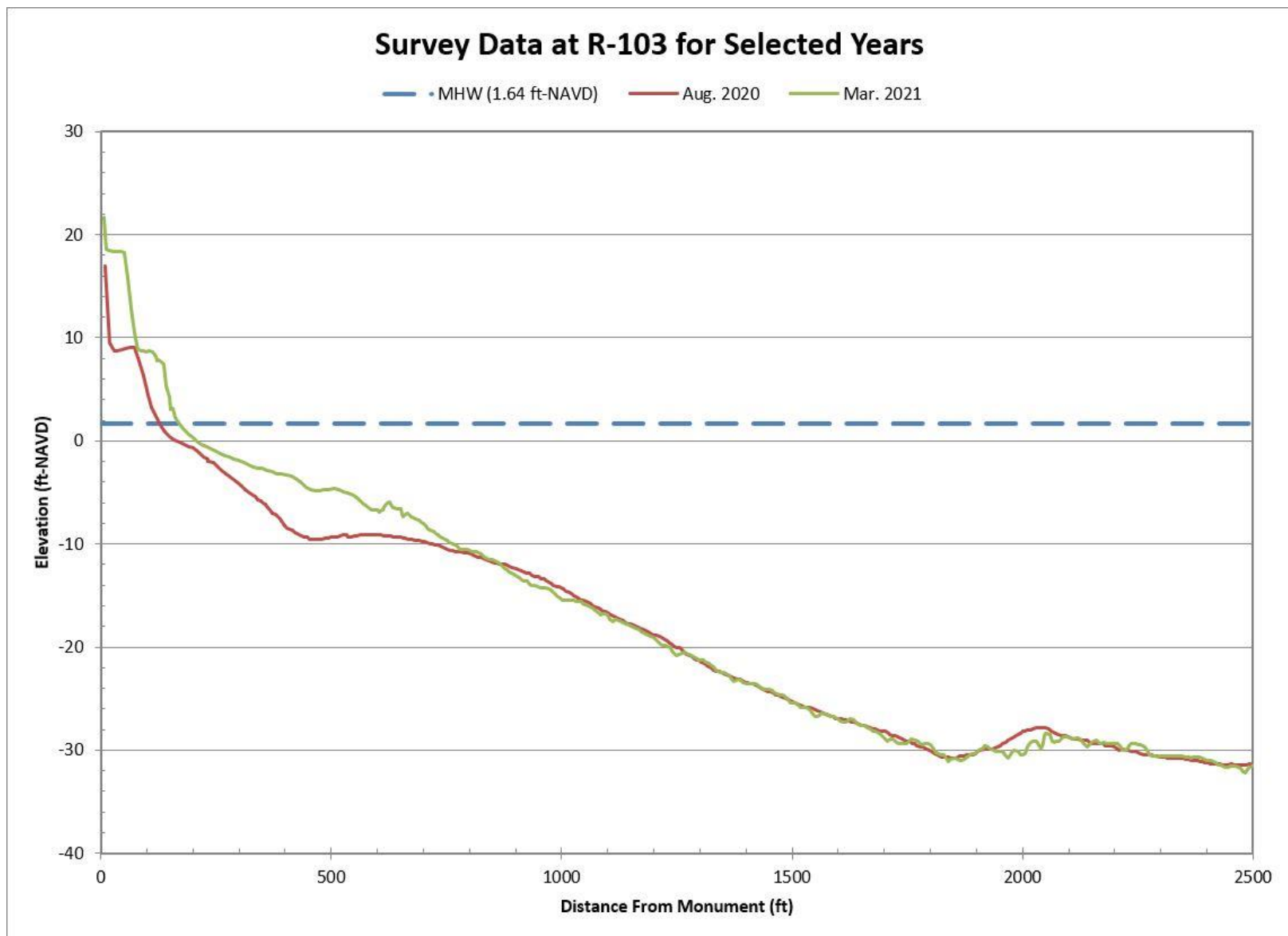
Figure B-24. Aug. 2020 Pre-Construction vs. Mar. 2021 Post-Construction Beach Profiles Along R-103
