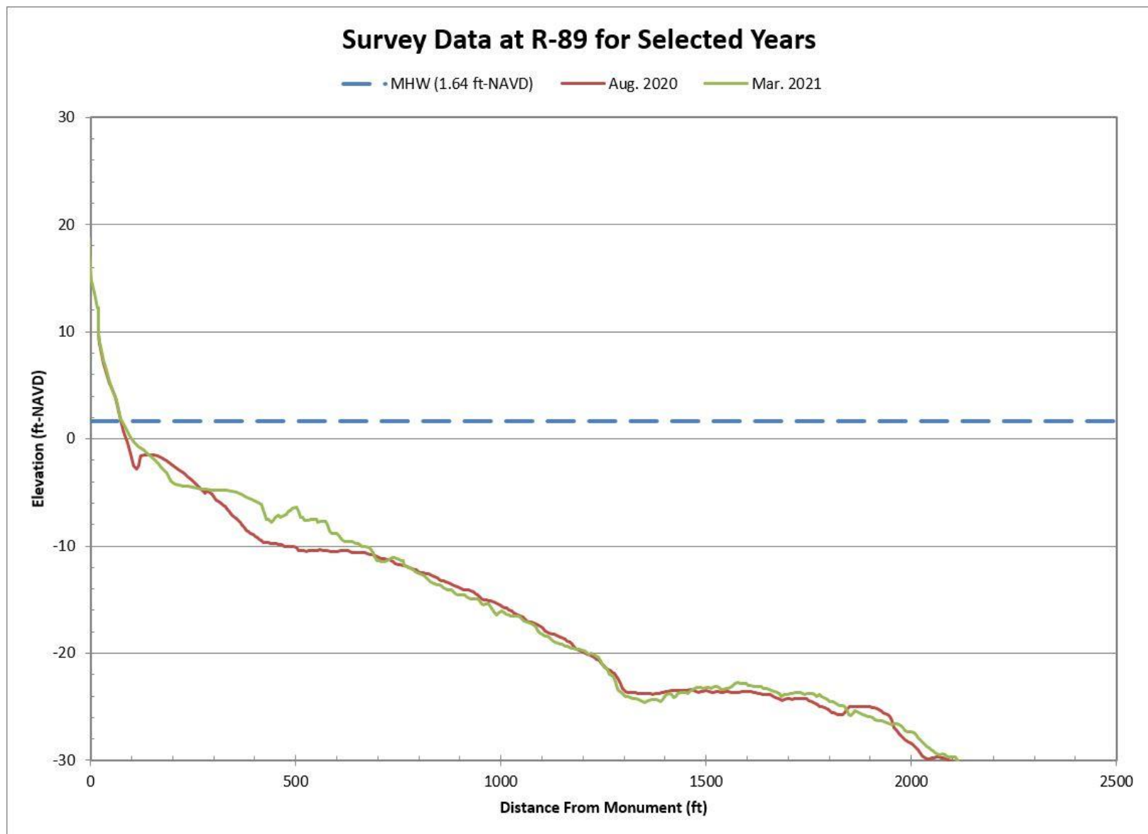
Figure B-10. Aug. 2020 Pre-Construction vs. Mar. 2021 Post-Construction Beach Profiles Along R-89
