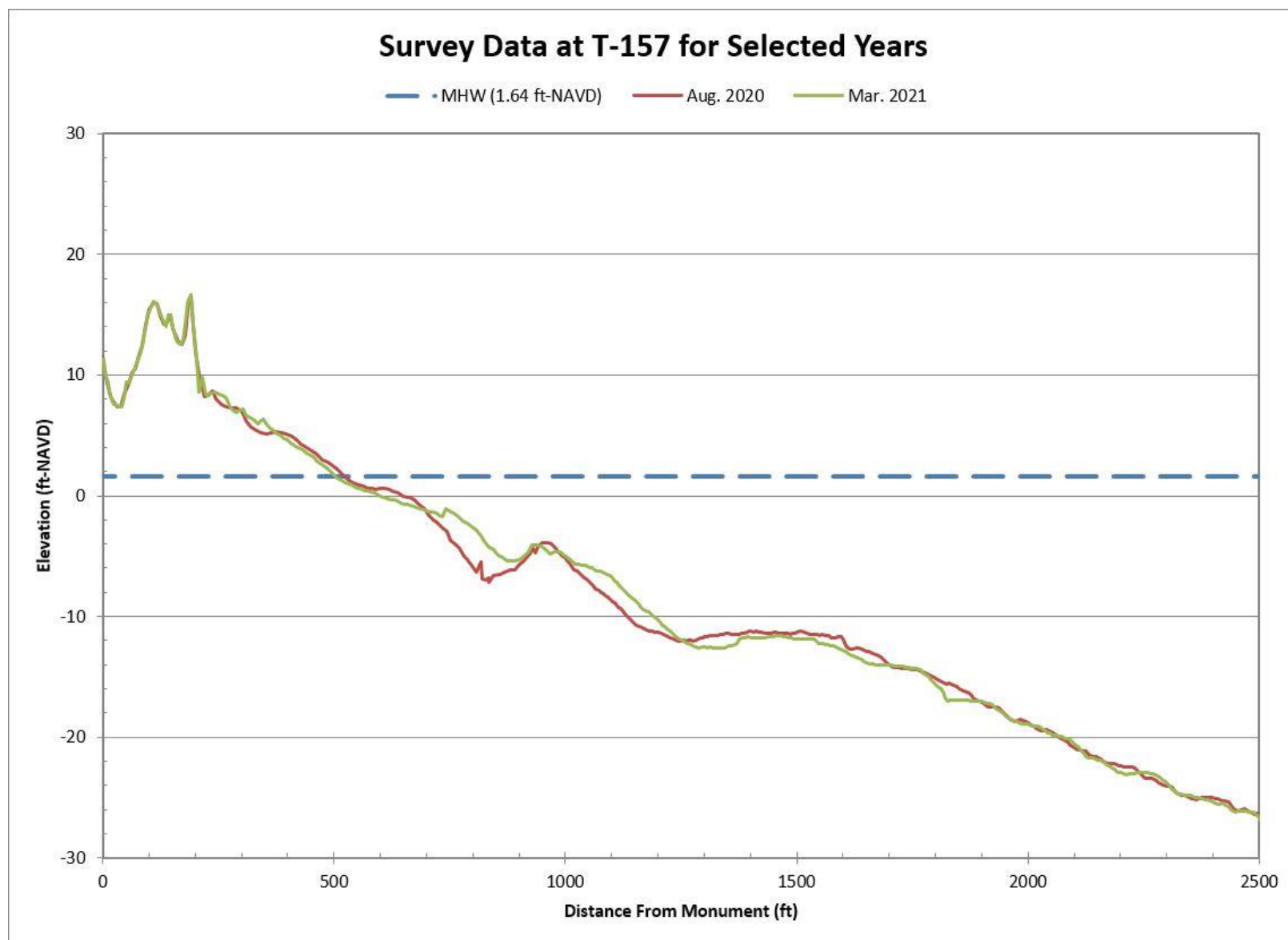
Figure B-81. Aug. 2020 Pre-Construction vs. Mar. 2021 Post-Construction Beach Profiles Along T-157
