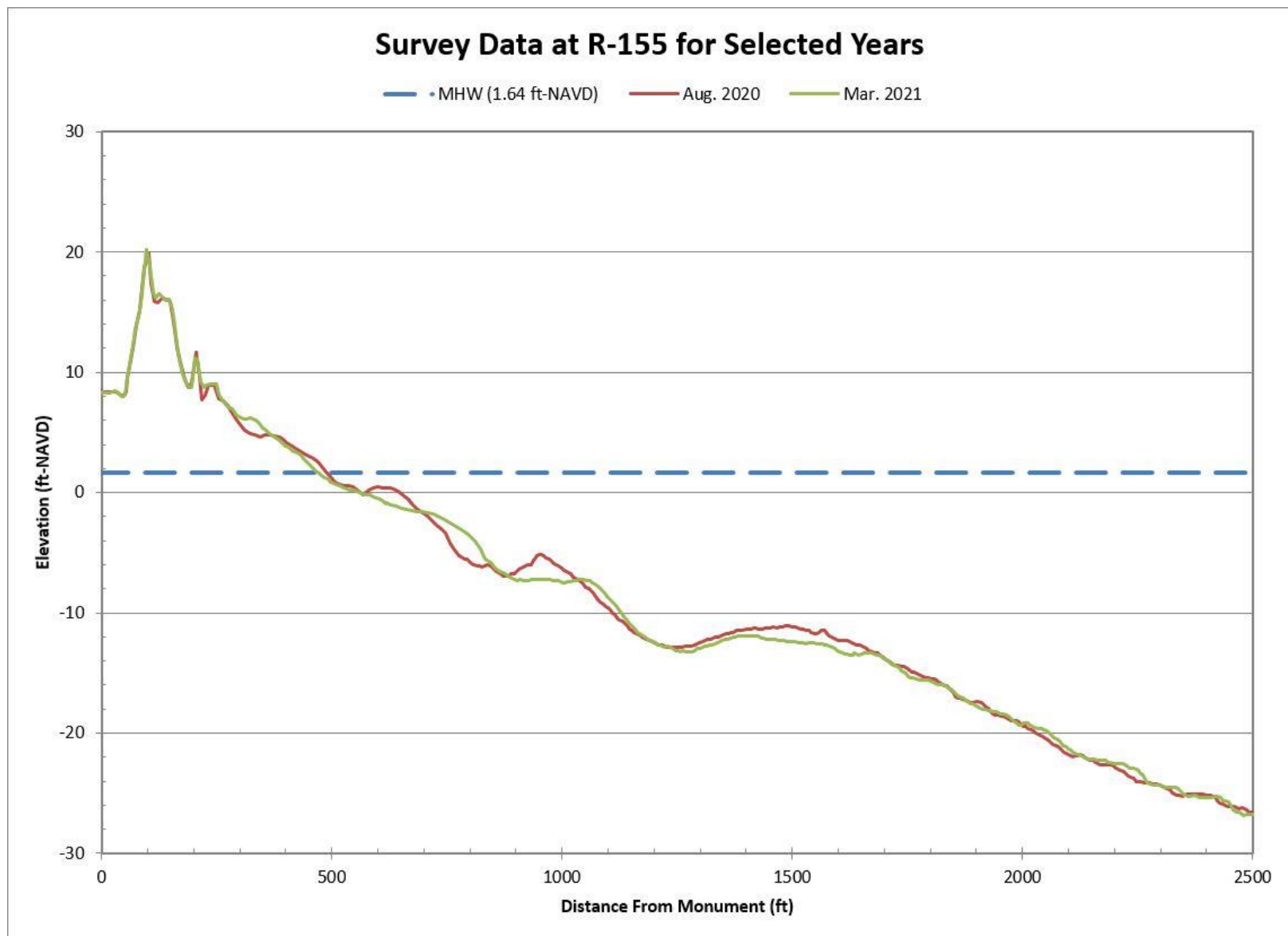
Figure B-79. Aug. 2020 Pre-Construction vs. Mar. 2021 Post-Construction Beach Profiles Along R-155
