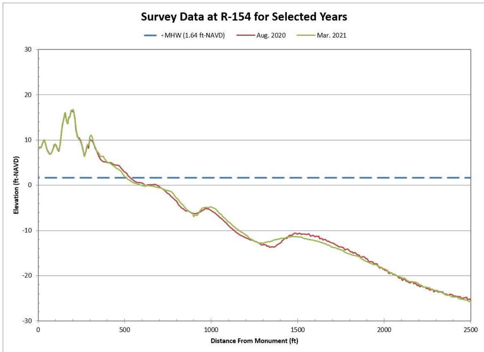
Figure B-78. Aug. 2020 Pre-Construction vs. Mar. 2021 Post-Construction Beach Profiles Along R-154
