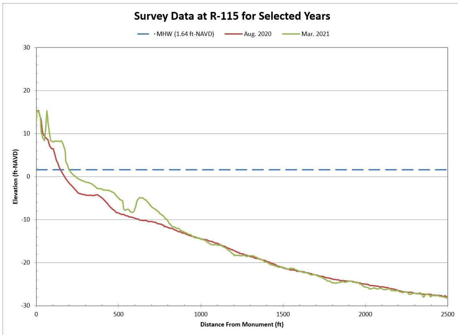
Figure B-36. Aug. 2020 Pre-Construction vs. Mar. 2021 Post-Construction Beach Profiles Along R-115
