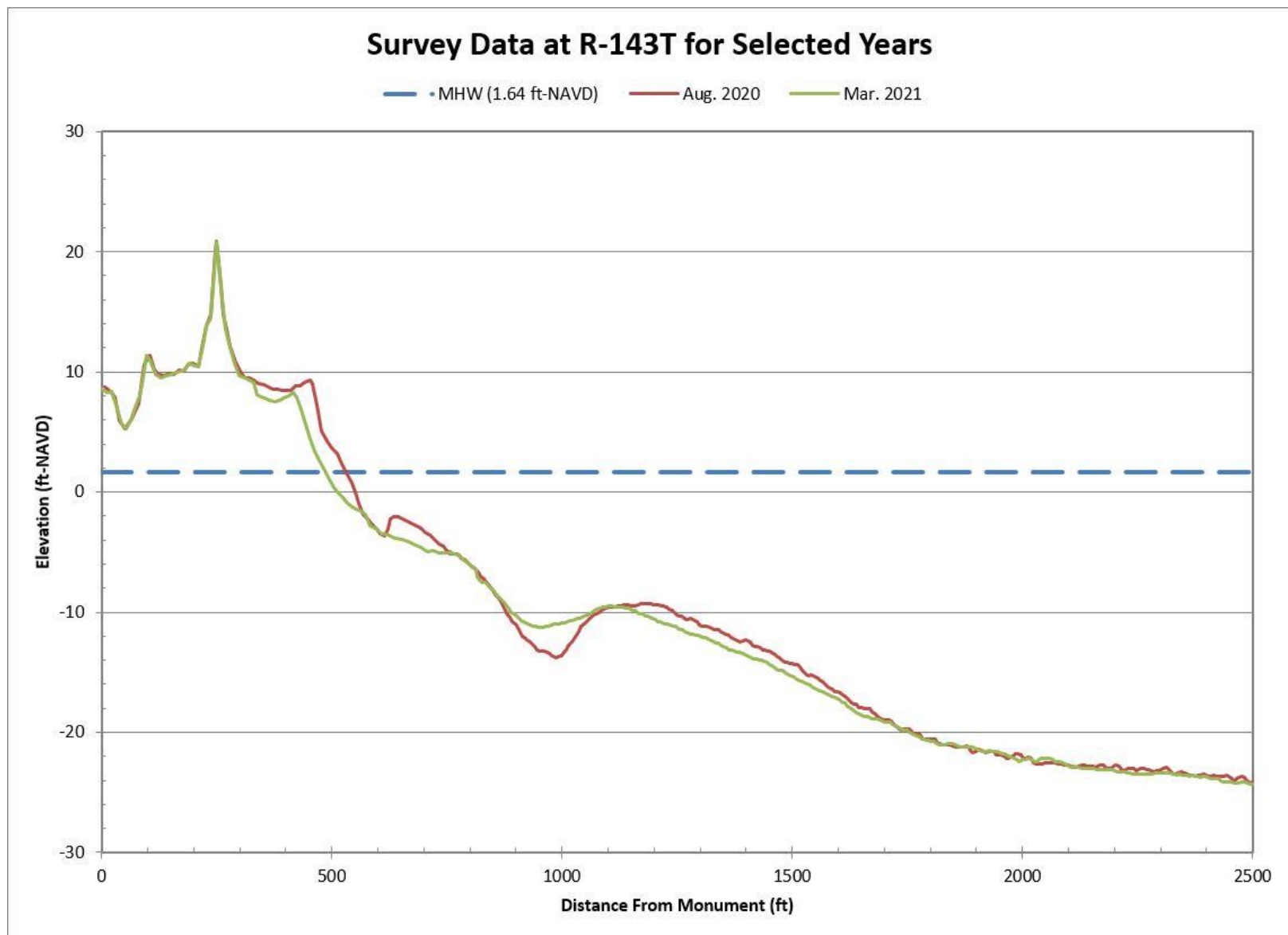
Figure B-67. Aug. 2020 Pre-Construction vs. Mar. 2021 Post-Construction Beach Profiles Along R-143T
