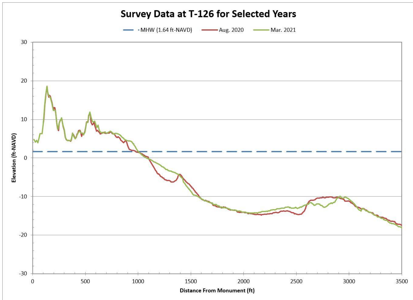
Figure B-50. Aug. 2020 Pre-Construction vs. Mar. 2021 Post-Construction Beach Profiles Along T-126
