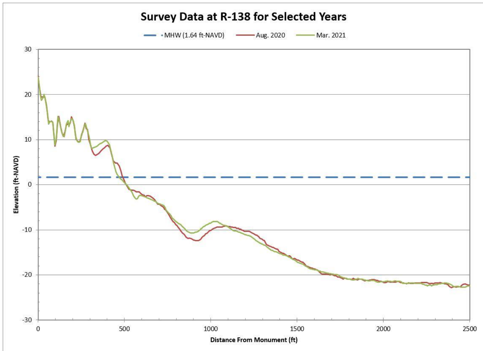
Figure B-62. Aug. 2020 Pre-Construction vs. Mar. 2021 Post-Construction Beach Profiles Along R-138
