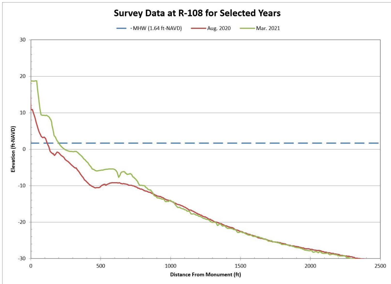
Figure B-29. Aug. 2020 Pre-Construction vs. Mar. 2021 Post-Construction Beach Profiles Along R-108
