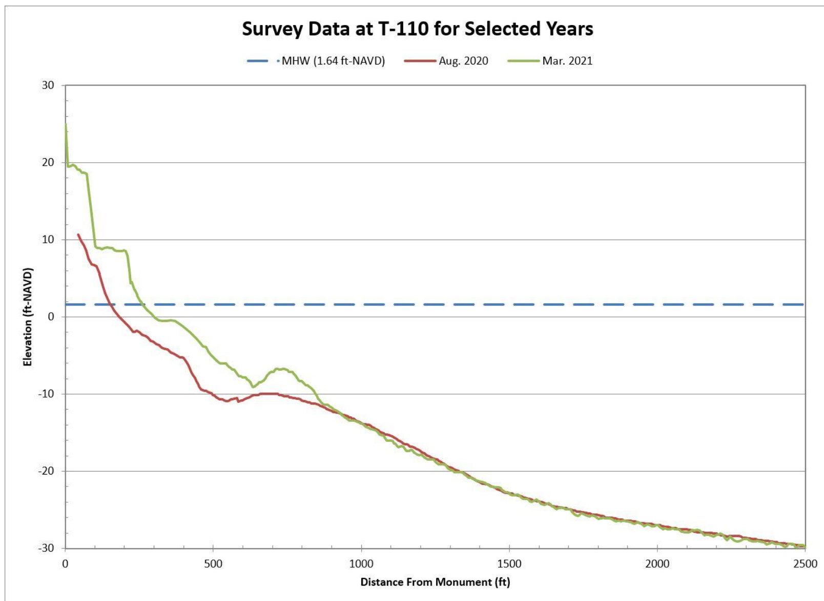
Figure B-31. Aug. 2020 Pre-Construction vs. Mar. 2021 Post-Construction Beach Profiles Along T-110
