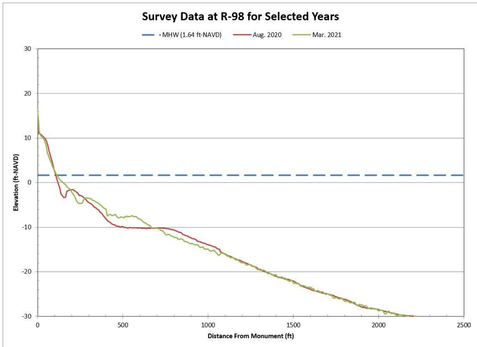
Figure B-19. Aug. 2020 Pre-Construction vs. Mar. 2021 Post-Construction Beach Profiles Along R-98
