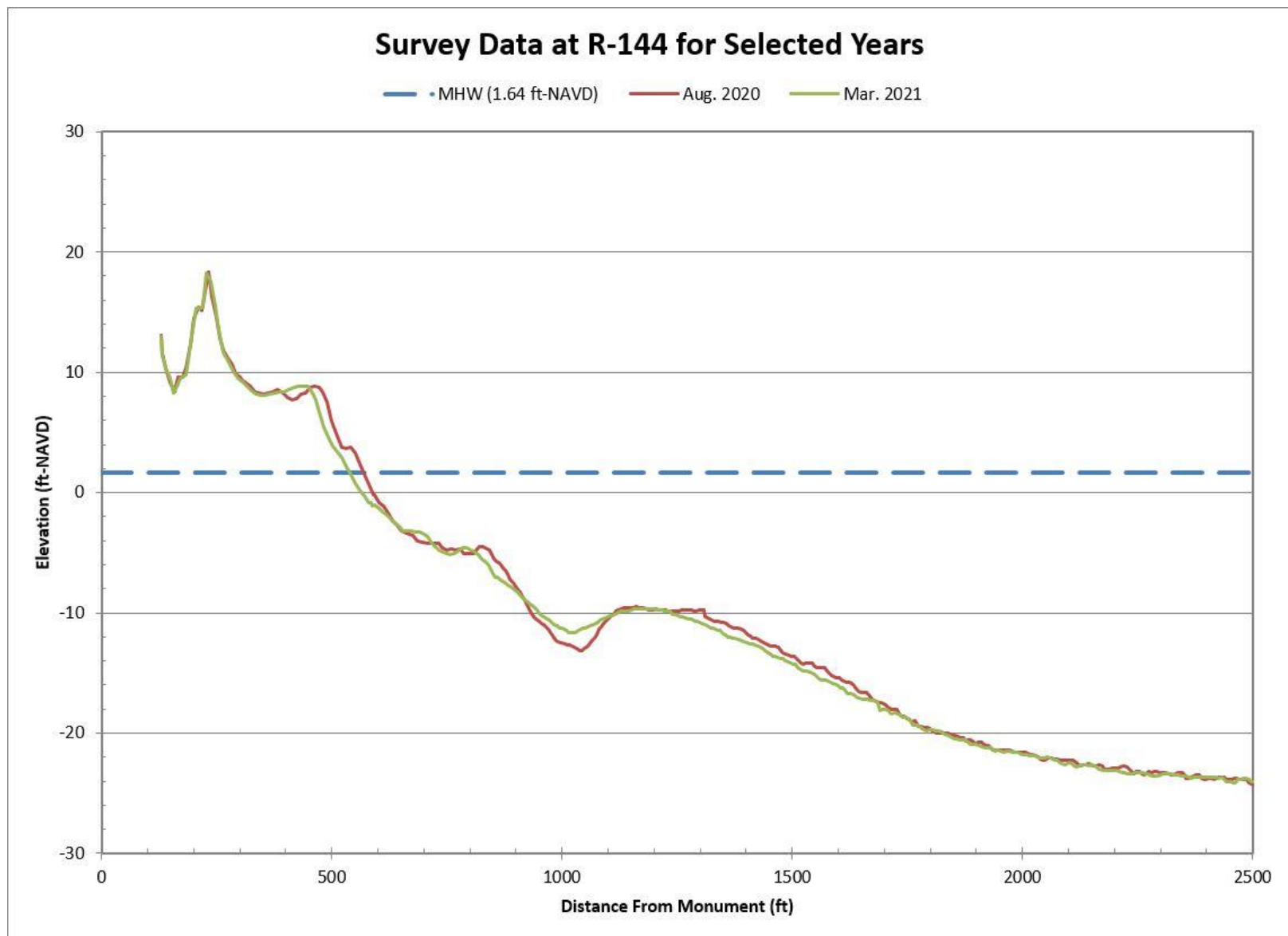
Figure B-68. Aug. 2020 Pre-Construction vs. Mar. 2021 Post-Construction Beach Profiles Along R-144
