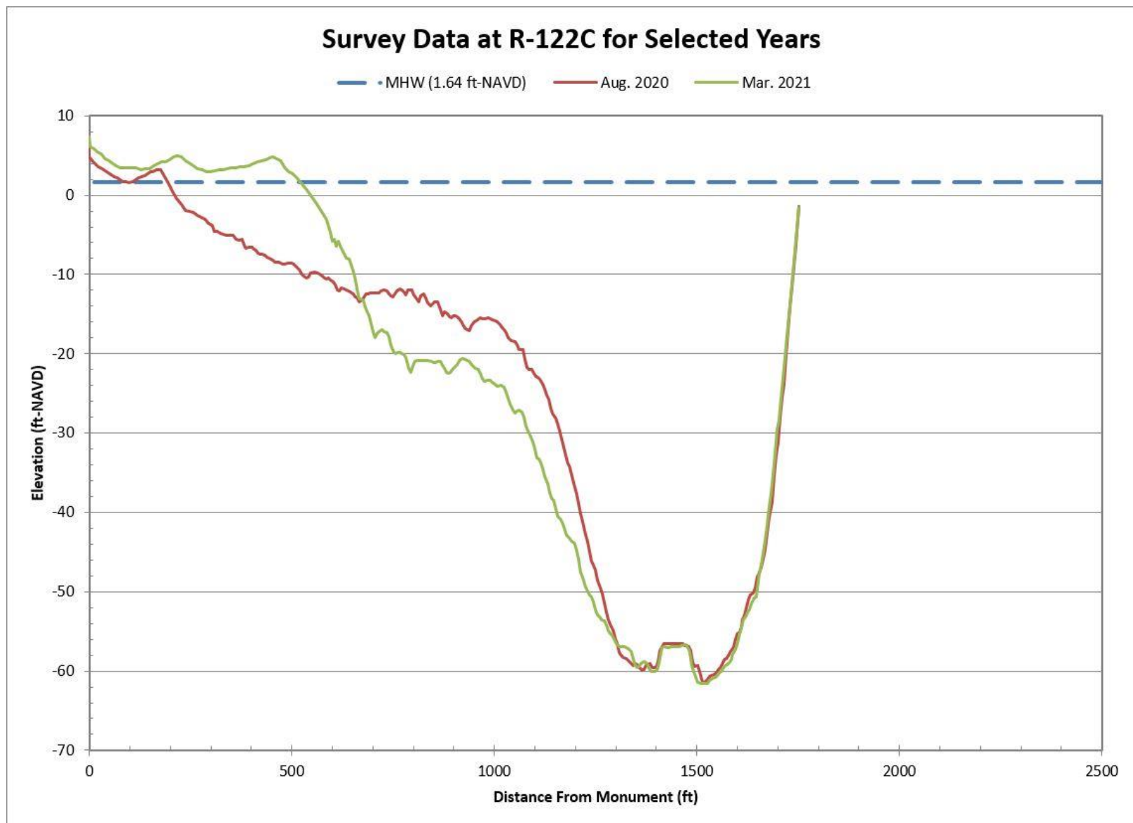
Figure B-46. Aug. 2020 Pre-Construction vs. Mar. 2021 Post-Construction Beach Profiles Along R-122C
