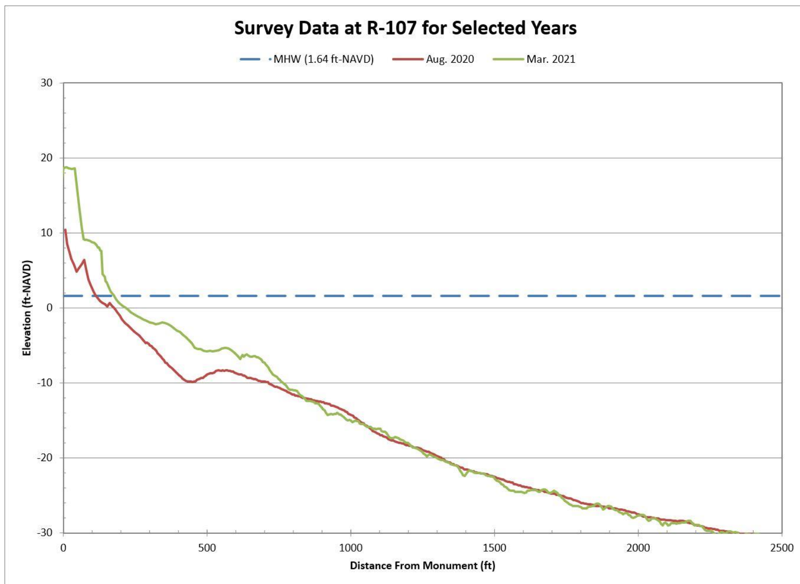
Figure B-28. Aug. 2020 Pre-Construction vs. Mar. 2021 Post-Construction Beach Profiles Along R-107
