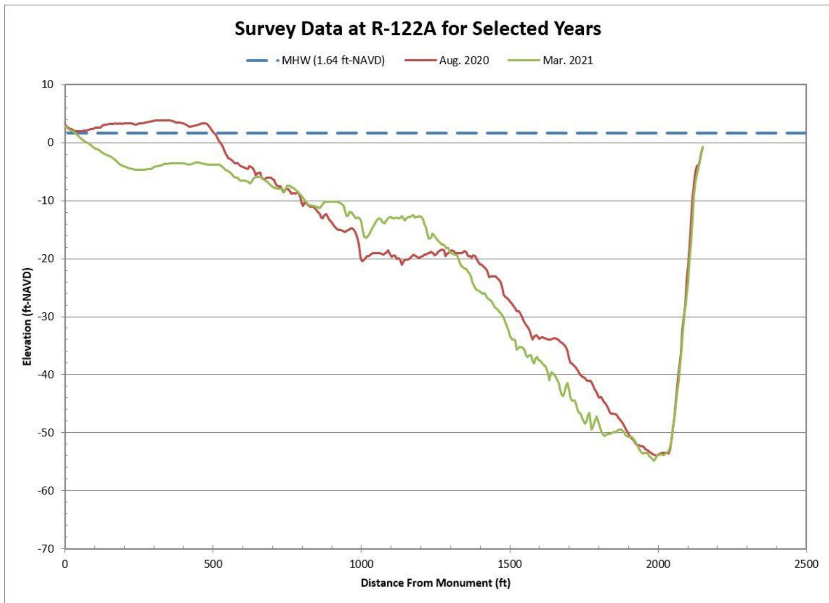
Figure B-44. Aug. 2020 Pre-Construction vs. Mar. 2021 Post-Construction Beach Profiles Along R-122A
