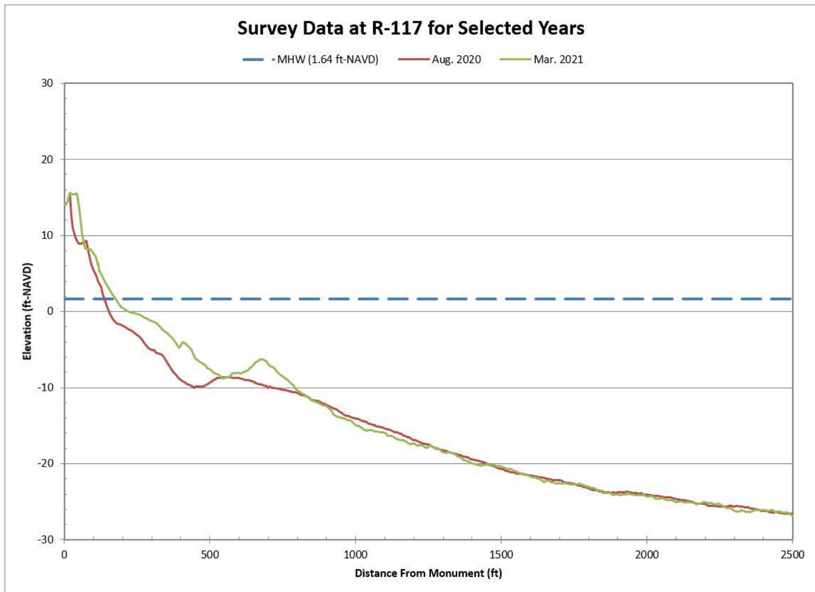
Figure B-38. Aug. 2020 Pre-Construction vs. Mar. 2021 Post-Construction Beach Profiles Along R-117
