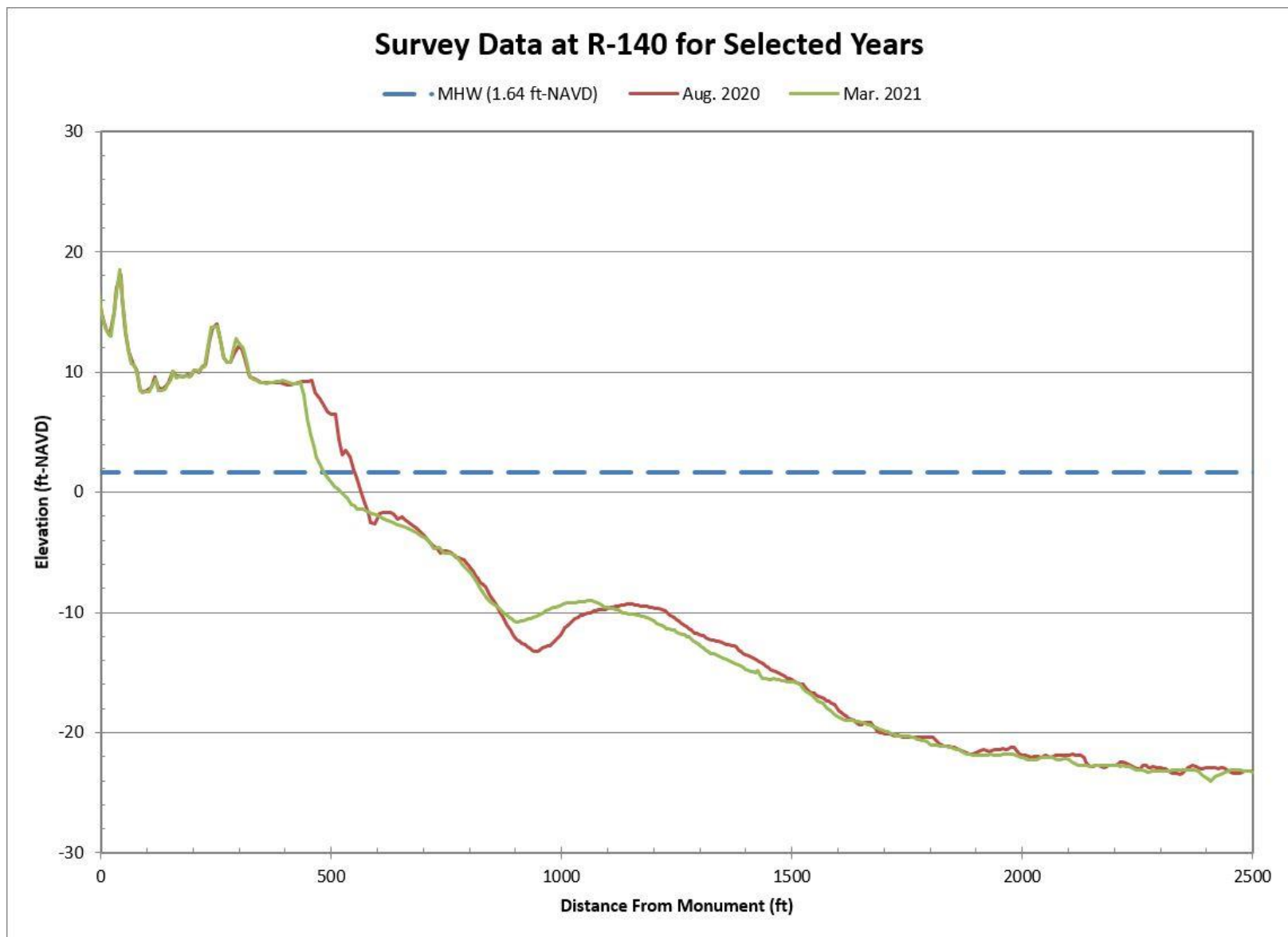
Figure B-64. Aug. 2020 Pre-Construction vs. Mar. 2021 Post-Construction Beach Profiles Along R-140
