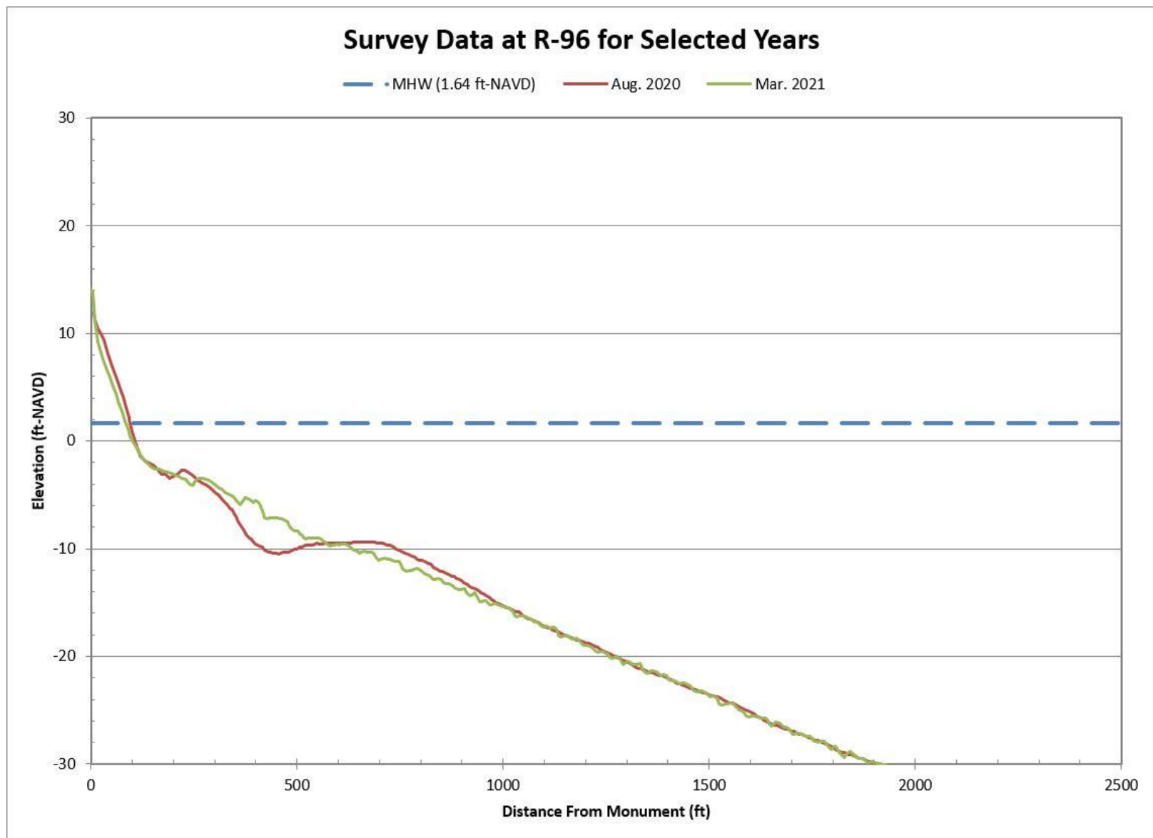
Figure B-17. Aug. 2020 Pre-Construction vs. Mar. 2021 Post-Construction Beach Profiles Along R-96
