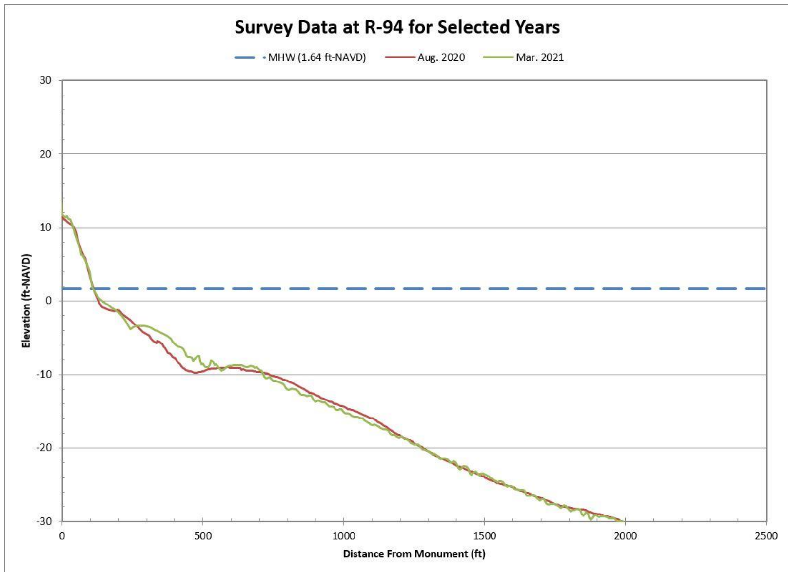
Figure B-15. Aug. 2020 Pre-Construction vs. Mar. 2021 Post-Construction Beach Profiles Along R-94
