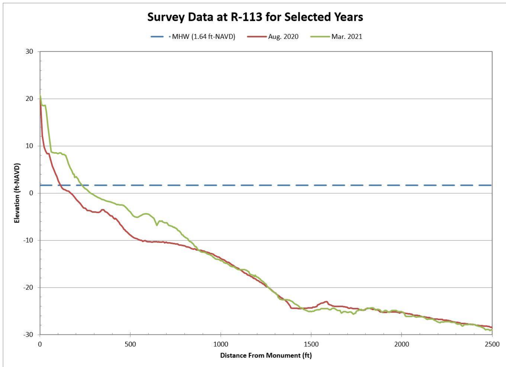
Figure B-34. Aug. 2020 Pre-Construction vs. Mar. 2021 Post-Construction Beach Profiles Along R-113
