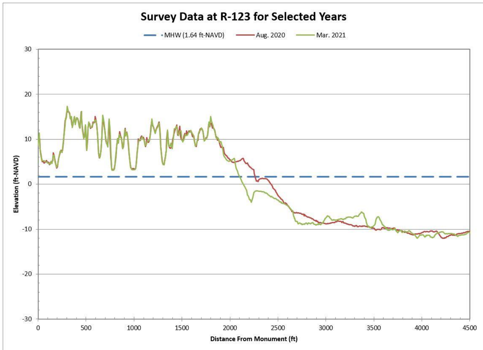
Figure B-47. Aug. 2020 Pre-Construction vs. Mar. 2021 Post-Construction Beach Profiles Along R-123
