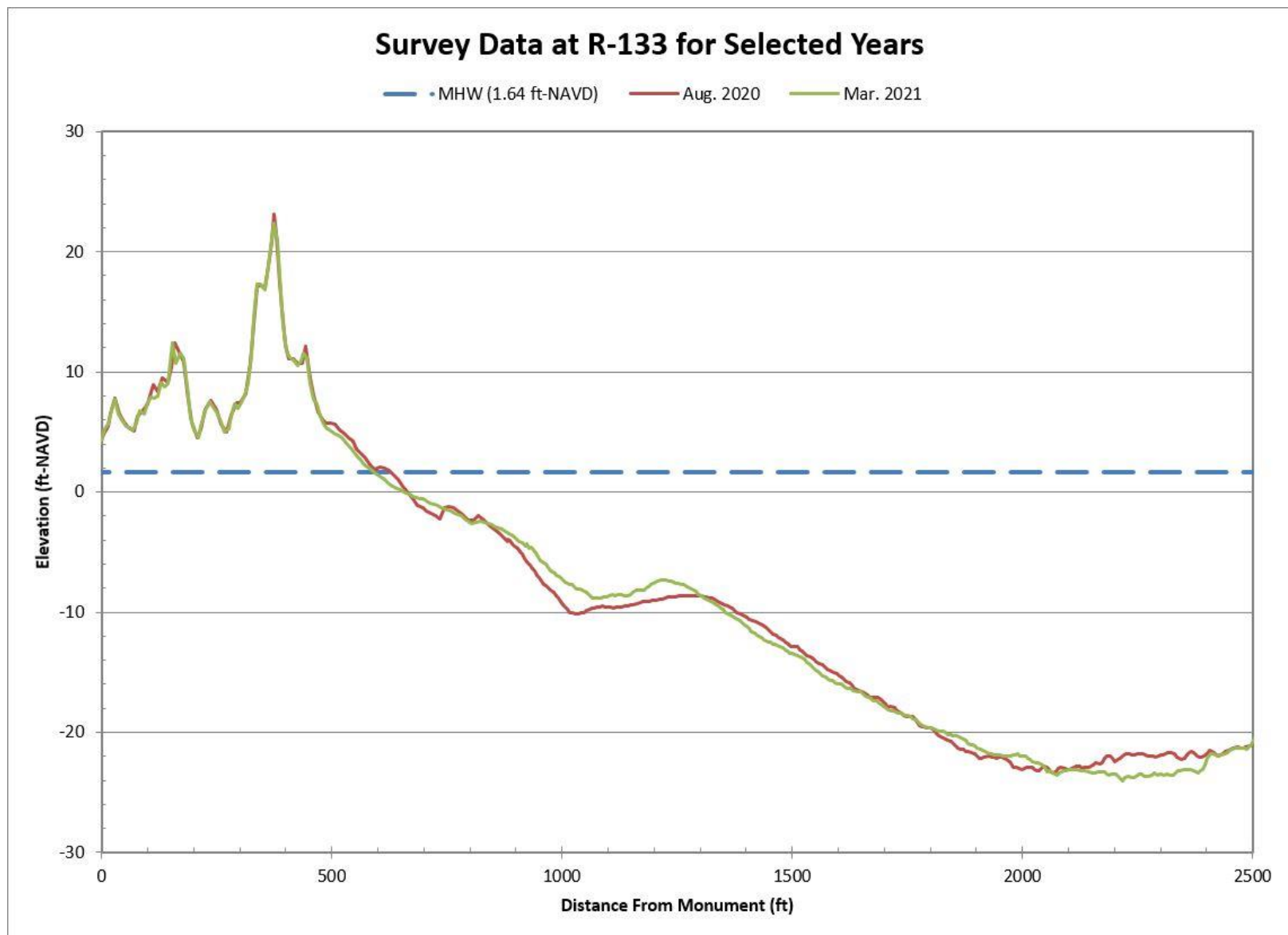
Figure B-57. Aug. 2020 Pre-Construction vs. Mar. 2021 Post-Construction Beach Profiles Along R-133
