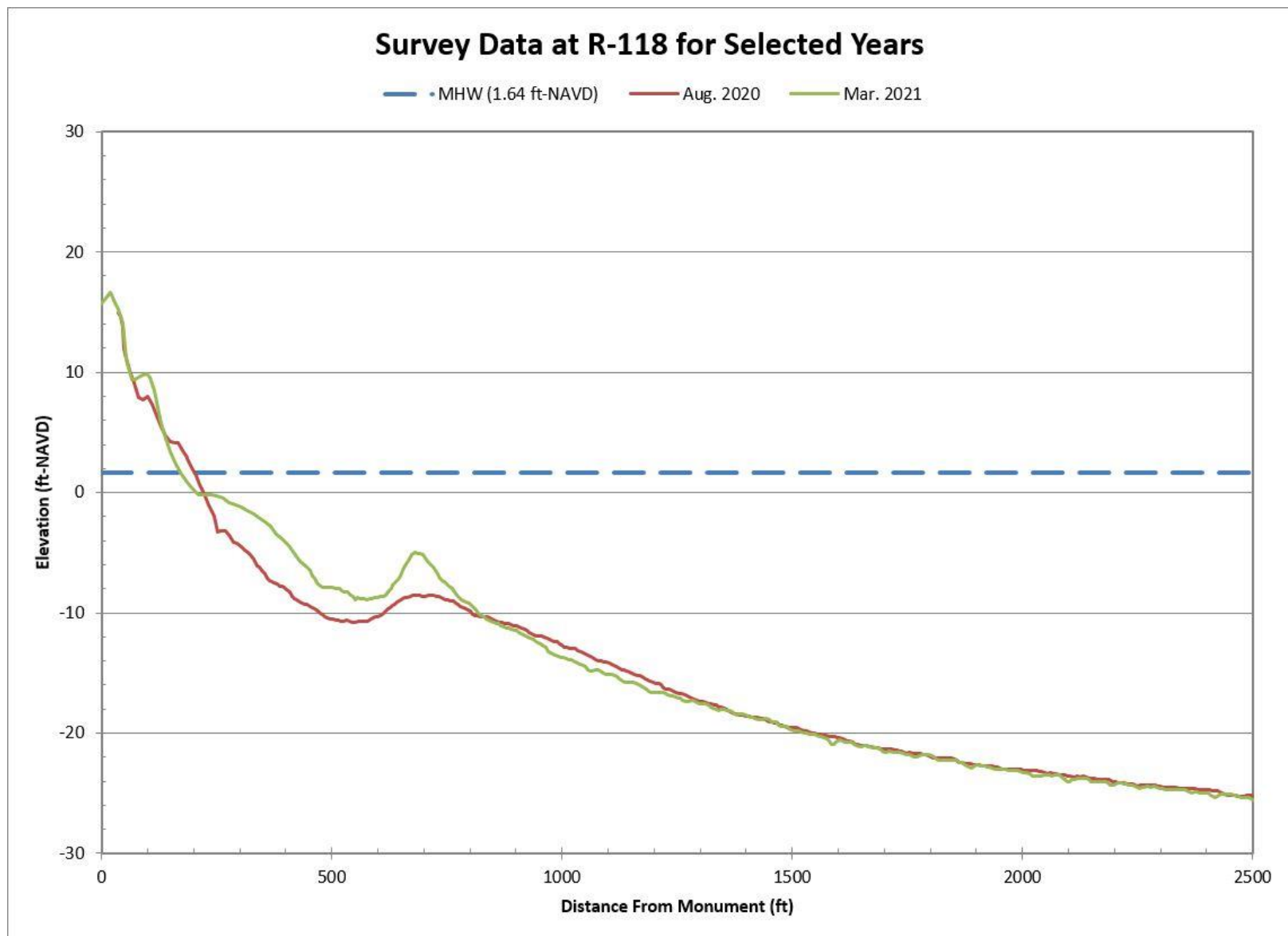
Figure B-39. Aug. 2020 Pre-Construction vs. Mar. 2021 Post-Construction Beach Profiles Along R-118
