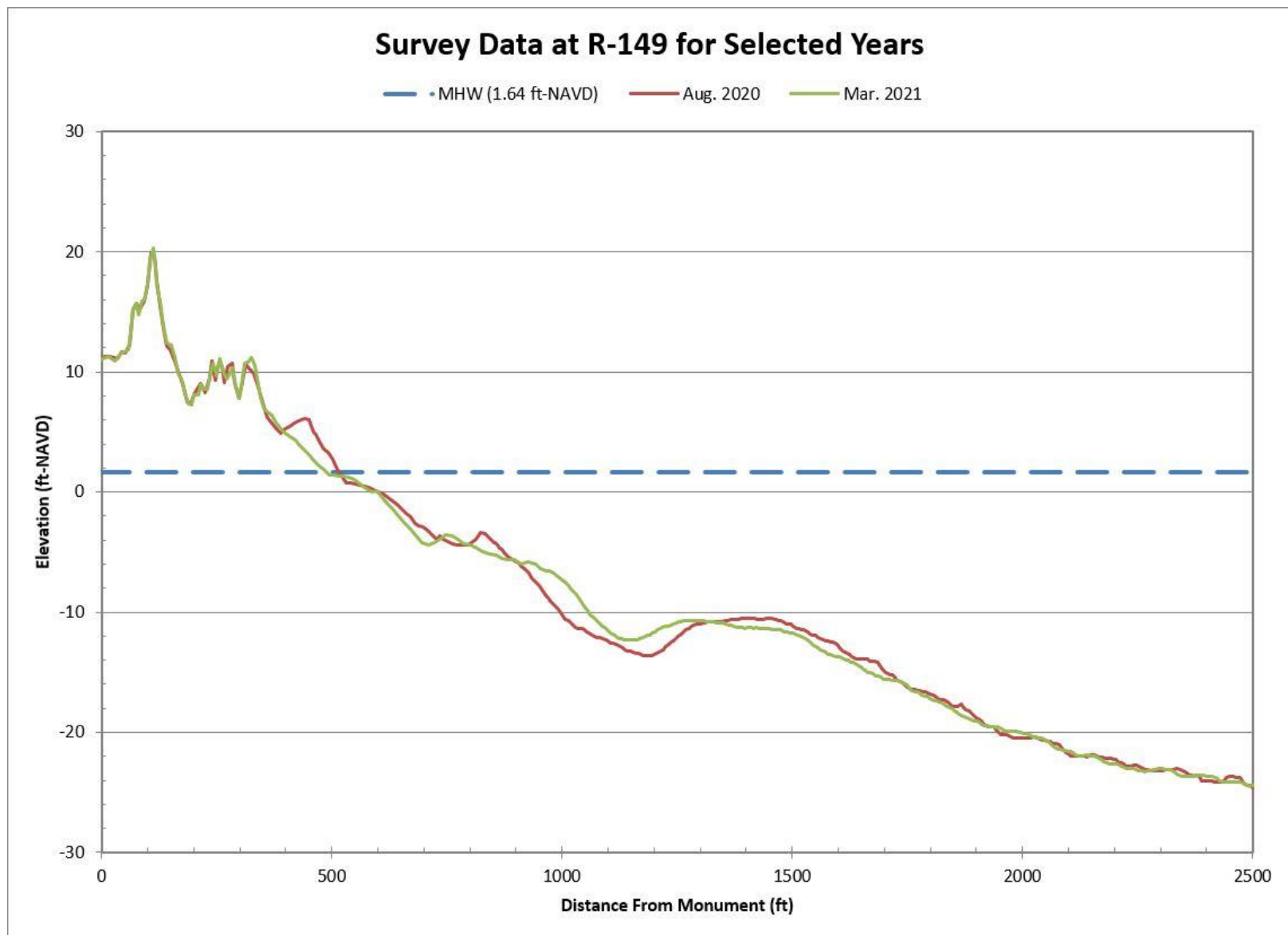
Figure B-73. Aug. 2020 Pre-Construction vs. Mar. 2021 Post-Construction Beach Profiles Along R-149
