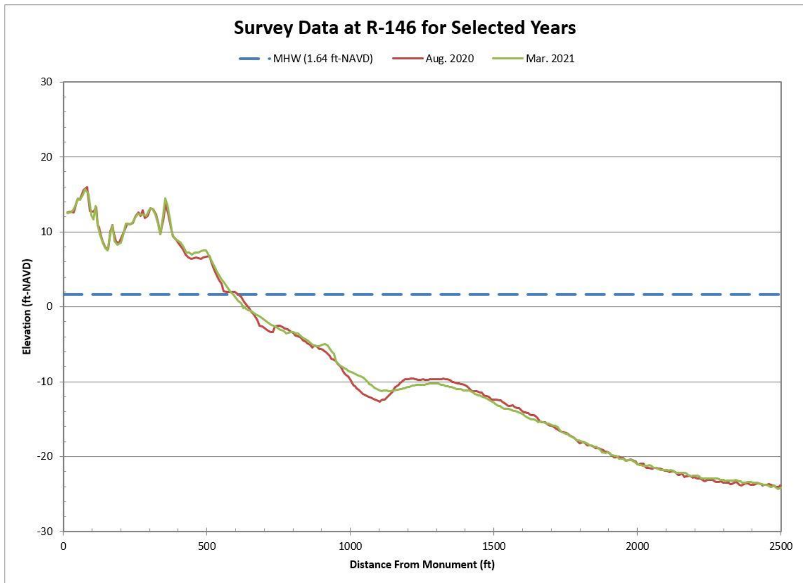
Figure B-70. Aug. 2020 Pre-Construction vs. Mar. 2021 Post-Construction Beach Profiles Along R-146
