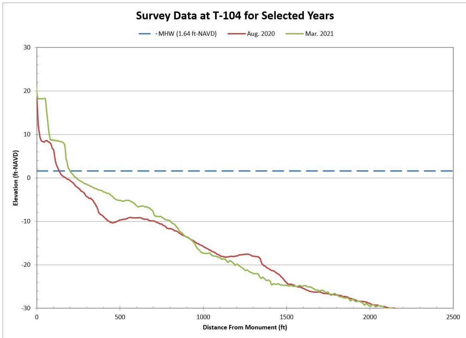
Figure B-25. Aug. 2020 Pre-Construction vs. Mar. 2021 Post-Construction Beach Profiles Along T-104
