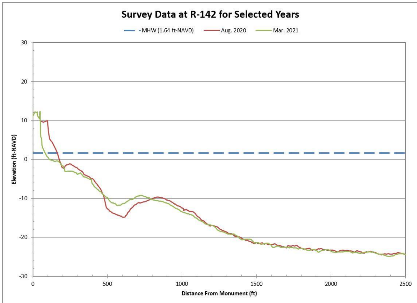
Figure B-66. Aug. 2020 Pre-Construction vs. Mar. 2021 Post-Construction Beach Profiles Along R-142
