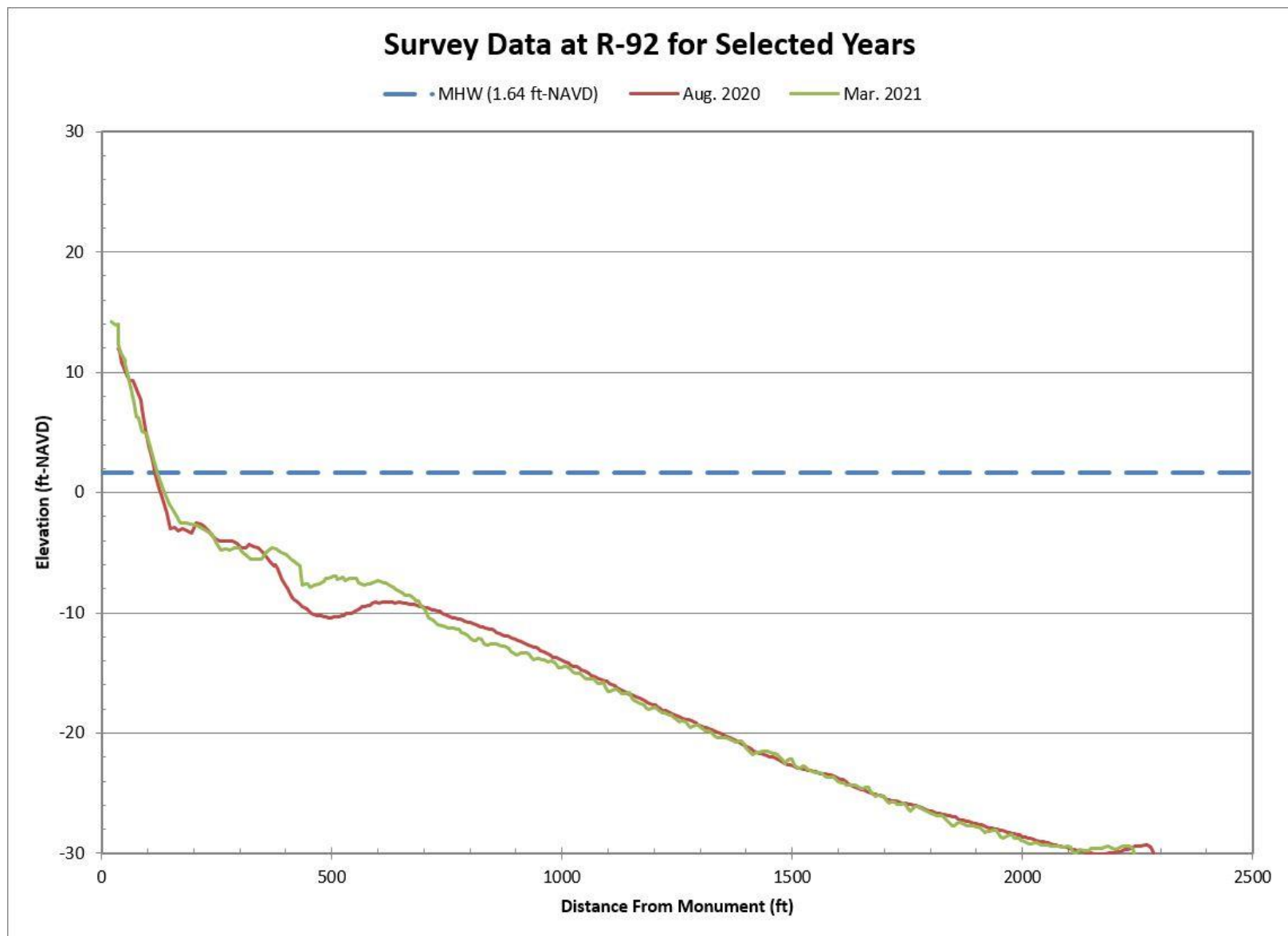
Figure B-13. Aug. 2020 Pre-Construction vs. Mar. 2021 Post-Construction Beach Profiles Along R-92
