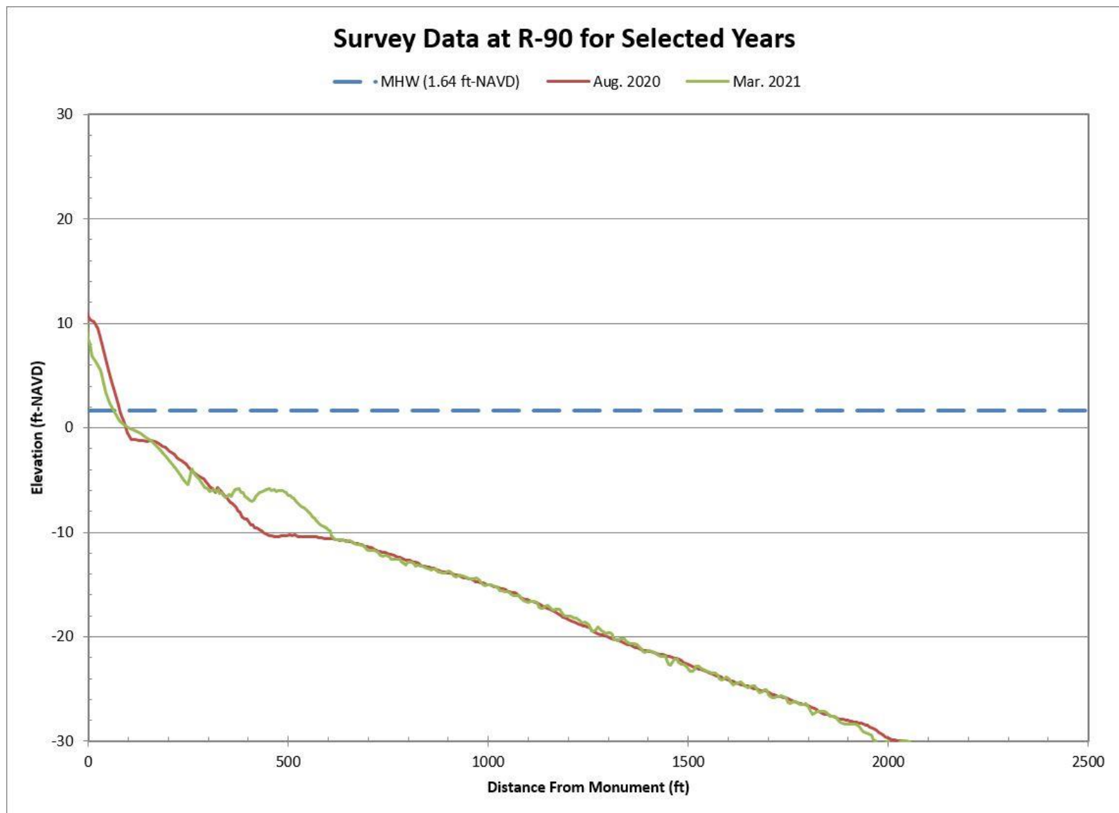
Figure B-11. Aug. 2020 Pre-Construction vs. Mar. 2021 Post-Construction Beach Profiles Along R-90
