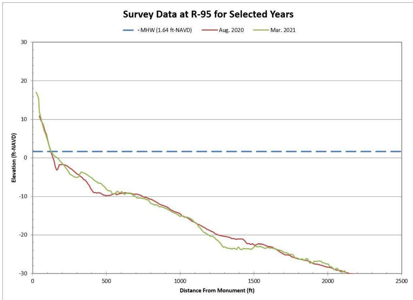
Figure B-16. Aug. 2020 Pre-Construction vs. Mar. 2021 Post-Construction Beach Profiles Along R-95
