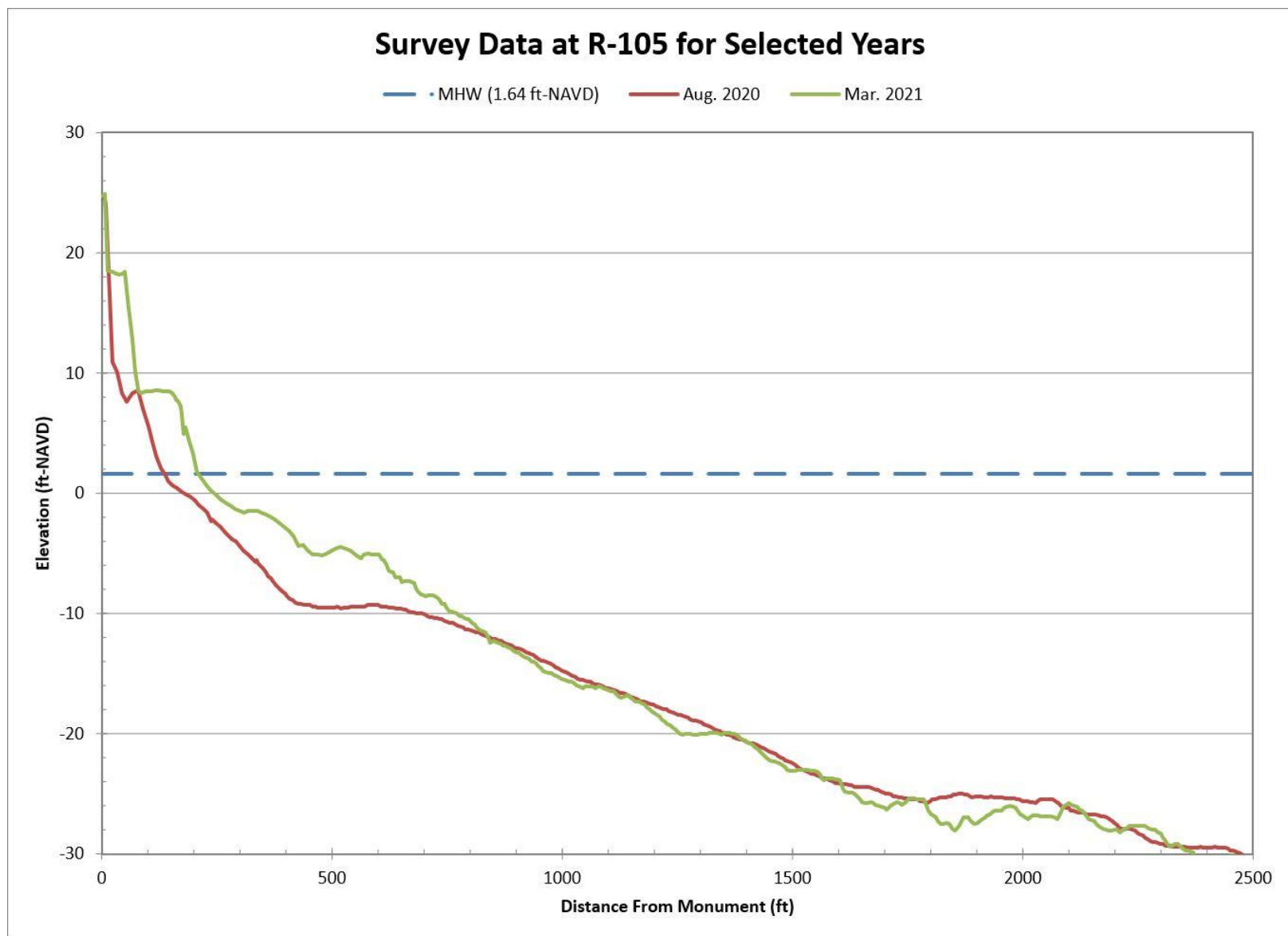
Figure B-26. Aug. 2020 Pre-Construction vs. Mar. 2021 Post-Construction Beach Profiles Along R-105
