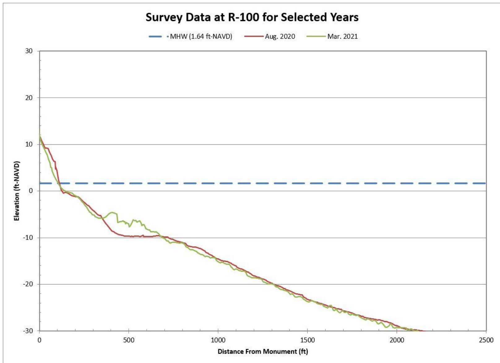
Figure B-21. Aug. 2020 Pre-Construction vs. Mar. 2021 Post-Construction Beach Profiles Along R-100
