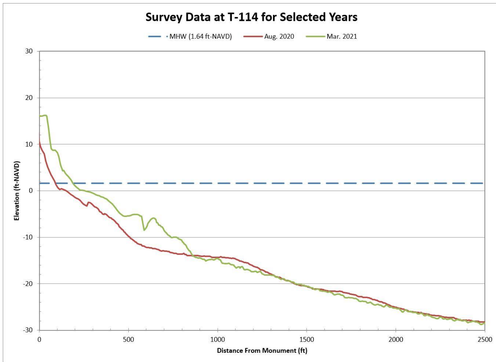
Figure B-35. Aug. 2020 Pre-Construction vs. Mar. 2021 Post-Construction Beach Profiles Along T-114
