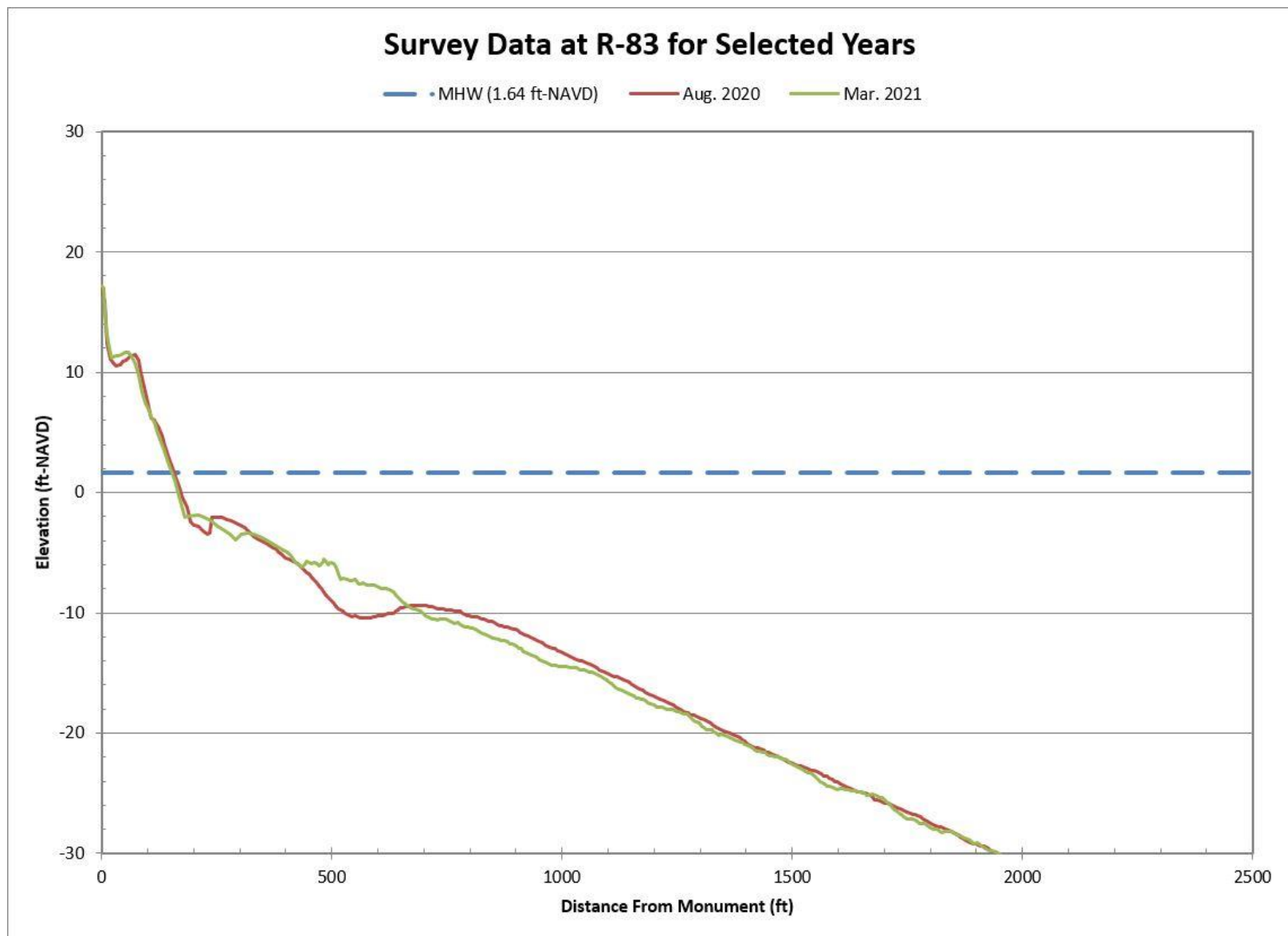
Figure B-4. Aug. 2020 Pre-Construction vs. Mar. 2021 Post-Construction Beach Profiles Along R-83
