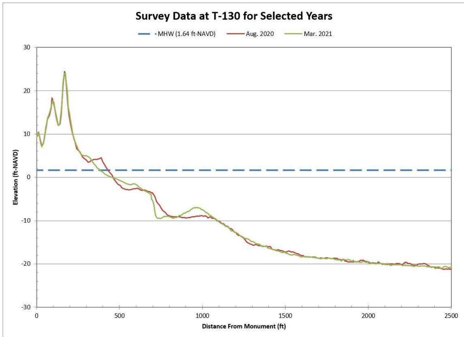
Figure B-54. Aug. 2020 Pre-Construction vs. Mar. 2021 Post-Construction Beach Profiles Along T-130
