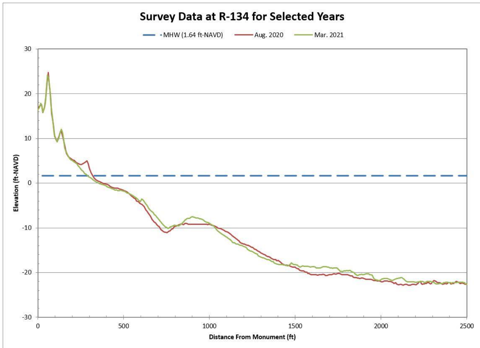
Figure B-58. Aug. 2020 Pre-Construction vs. Mar. 2021 Post-Construction Beach Profiles Along R-134
