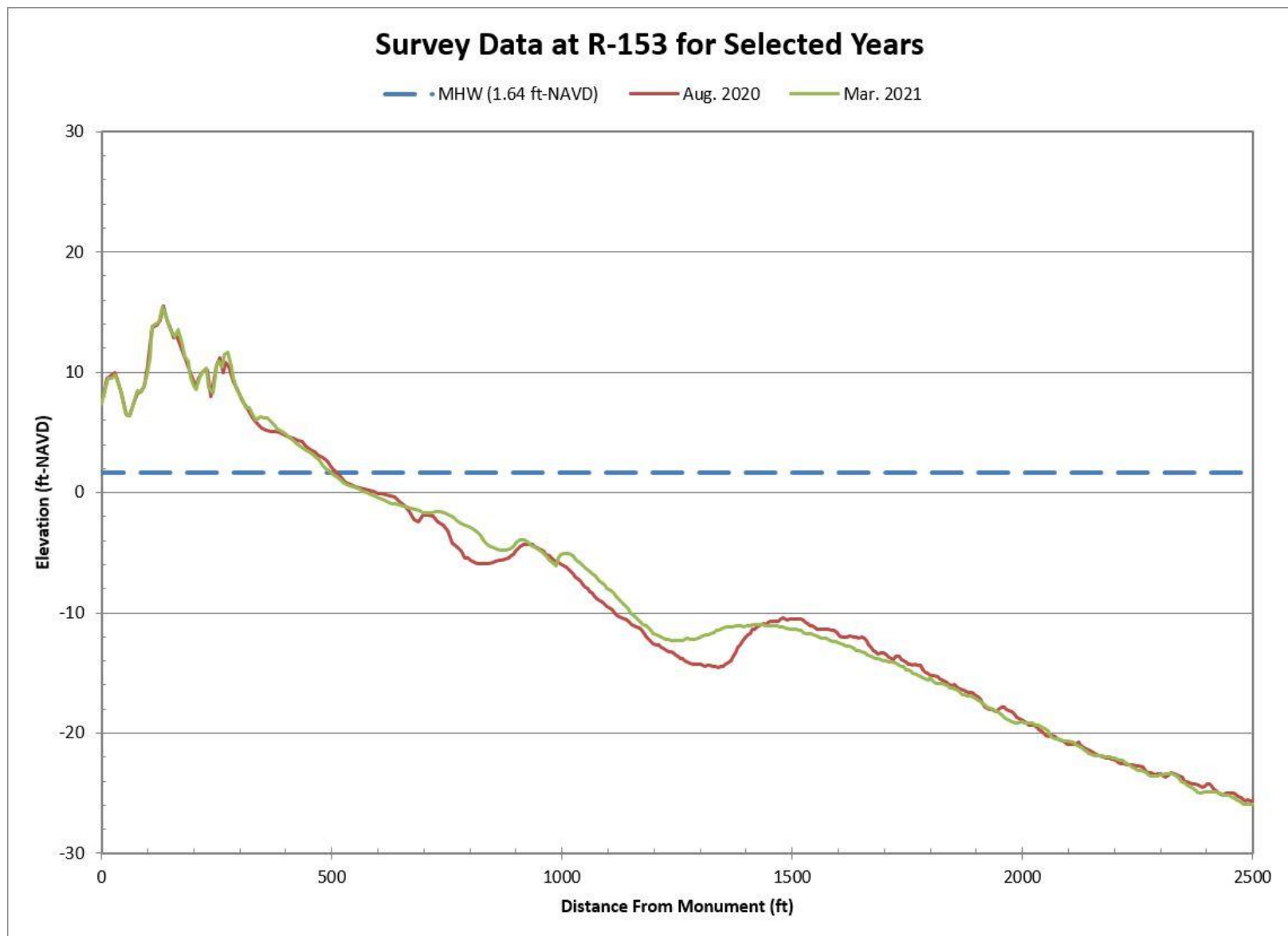
Figure B-77. Aug. 2020 Pre-Construction vs. Mar. 2021 Post-Construction Beach Profiles Along R-153
