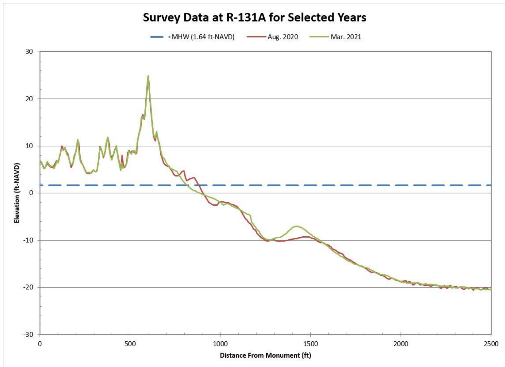
Figure B-55. Aug. 2020 Pre-Construction vs. Mar. 2021 Post-Construction Beach Profiles Along R-131A
