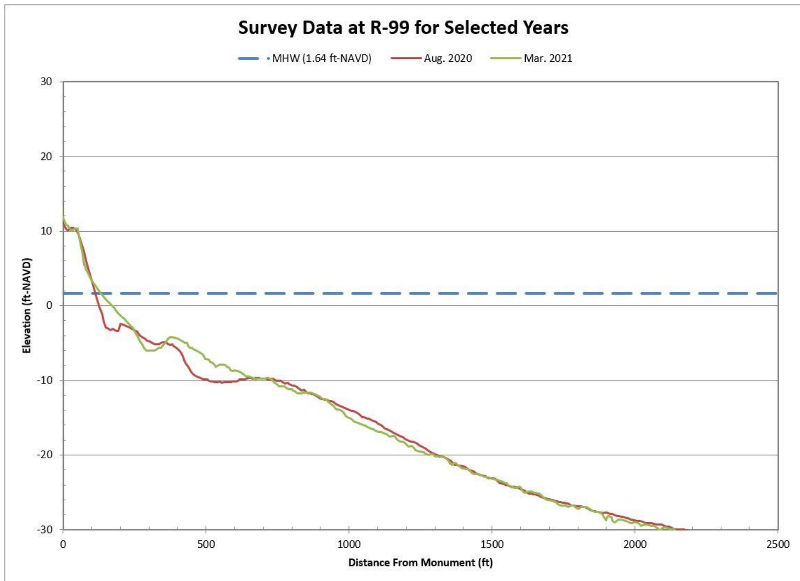
Figure B-20. Aug. 2020 Pre-Construction vs. Mar. 2021 Post-Construction Beach Profiles Along R-99
