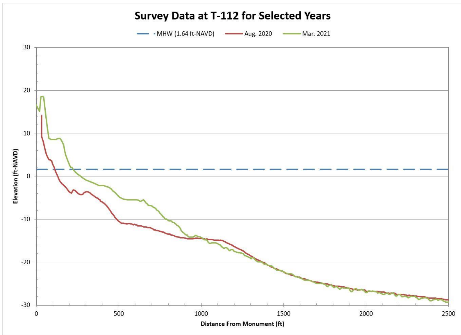
Figure B-33. Aug. 2020 Pre-Construction vs. Mar. 2021 Post-Construction Beach Profiles Along T-112
