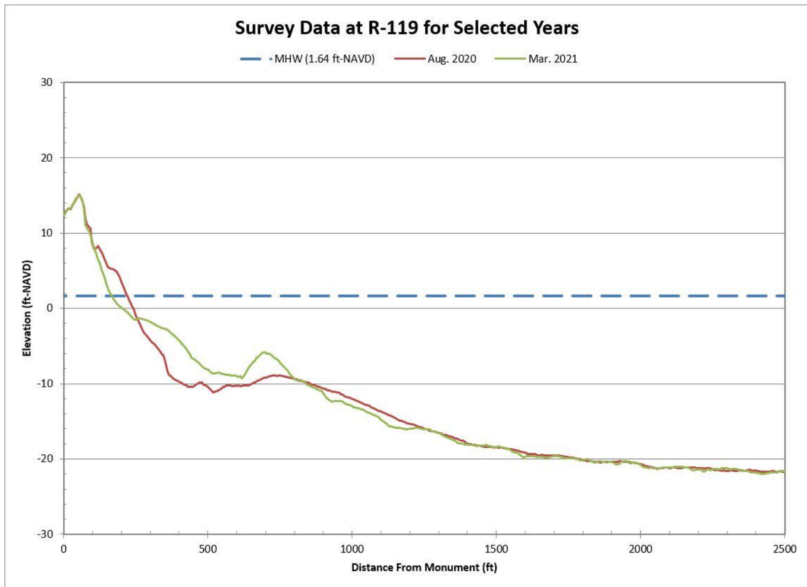
Figure B-40. Aug. 2020 Pre-Construction vs. Mar. 2021 Post-Construction Beach Profiles Along R-119
