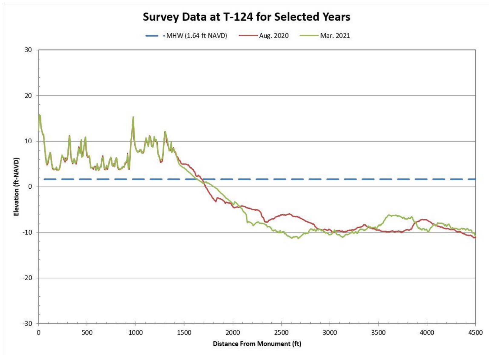
Figure B-48. Aug. 2020 Pre-Construction vs. Mar. 2021 Post-Construction Beach Profiles Along T-124
