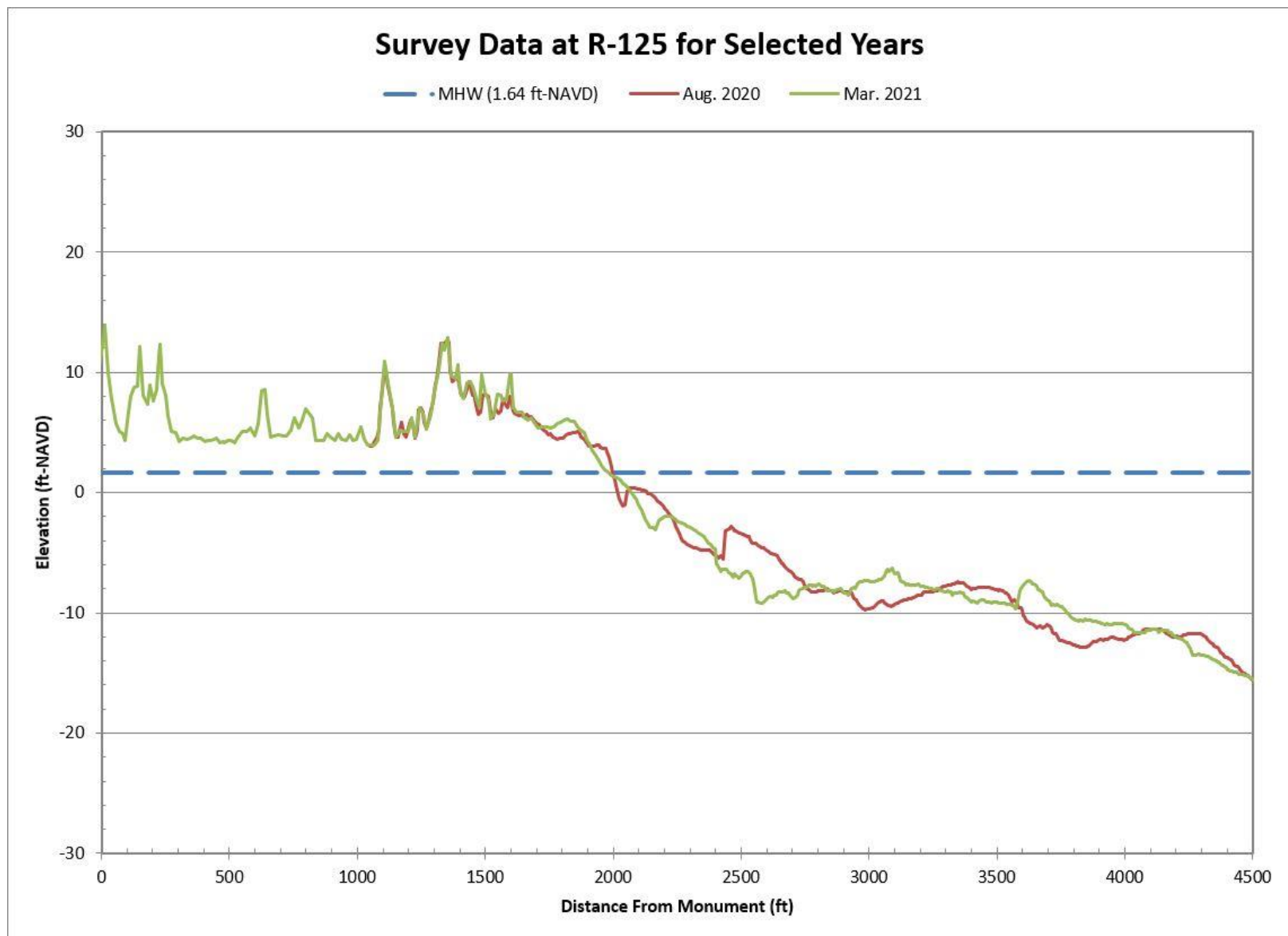
Figure B-49. Aug. 2020 Pre-Construction vs. Mar. 2021 Post-Construction Beach Profiles Along R-125
