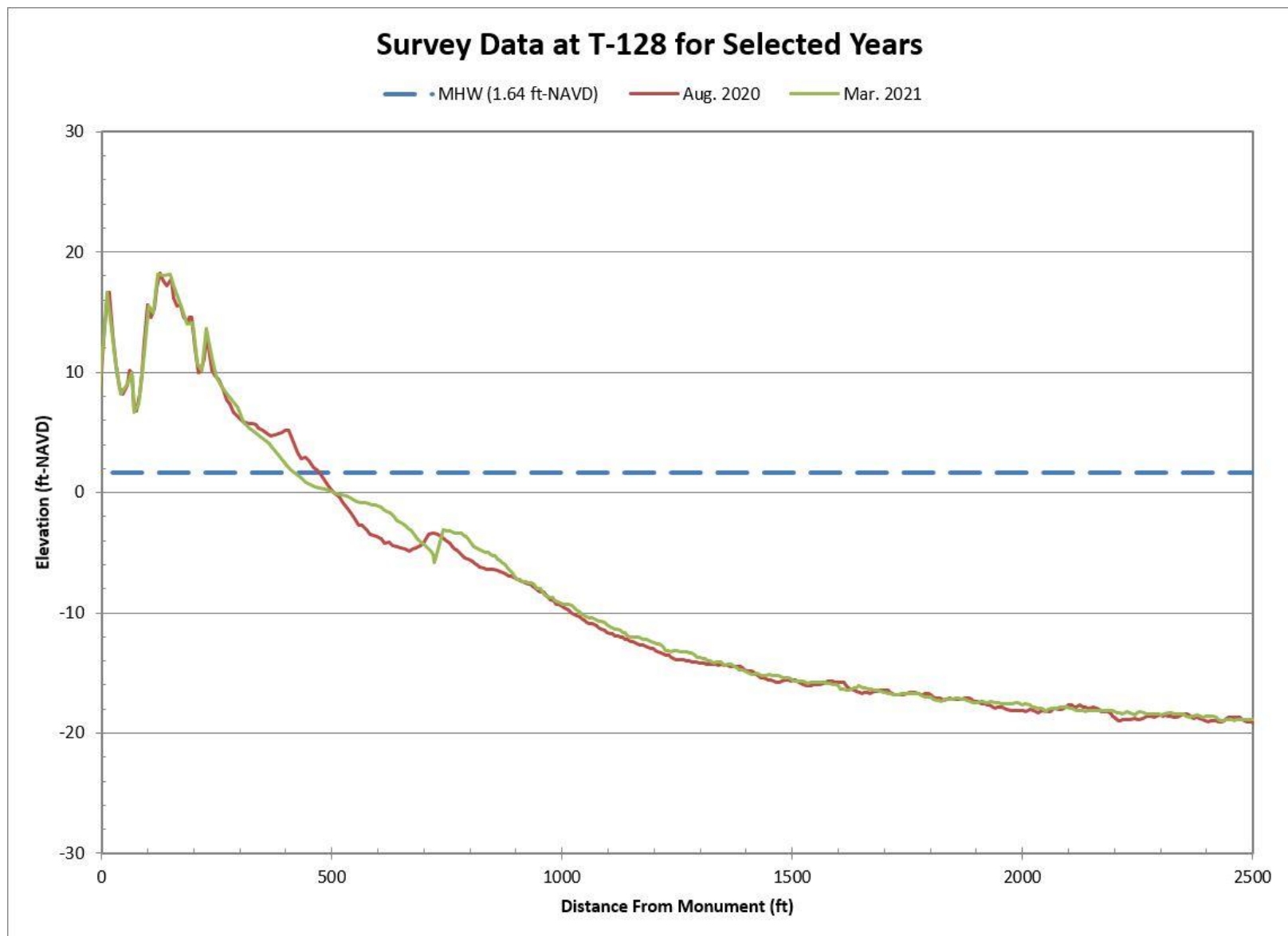
Figure B-52. Aug. 2020 Pre-Construction vs. Mar. 2021 Post-Construction Beach Profiles Along T-128
