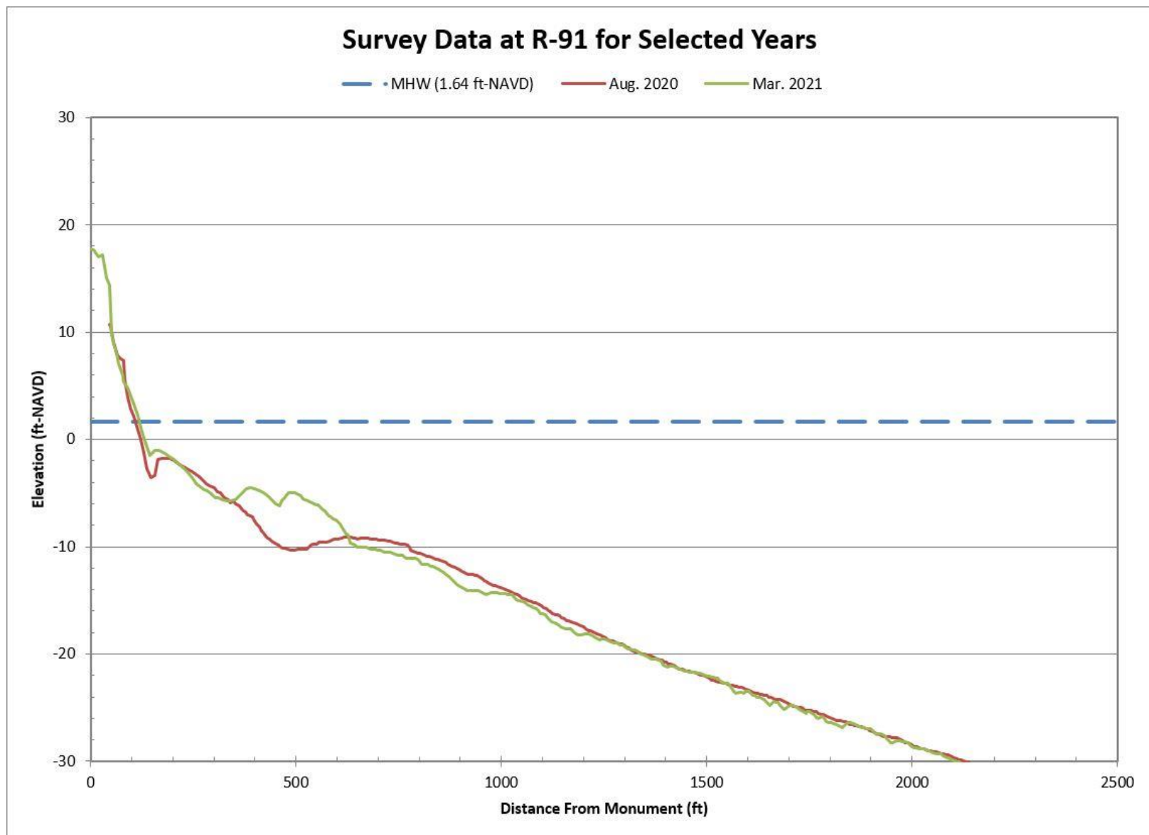
Figure B-12. Aug. 2020 Pre-Construction vs. Mar. 2021 Post-Construction Beach Profiles Along R-91
