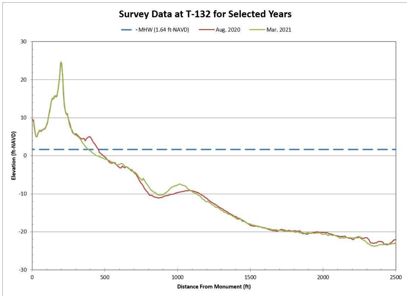
Figure B-56. Aug. 2020 Pre-Construction vs. Mar. 2021 Post-Construction Beach Profiles Along T-132
