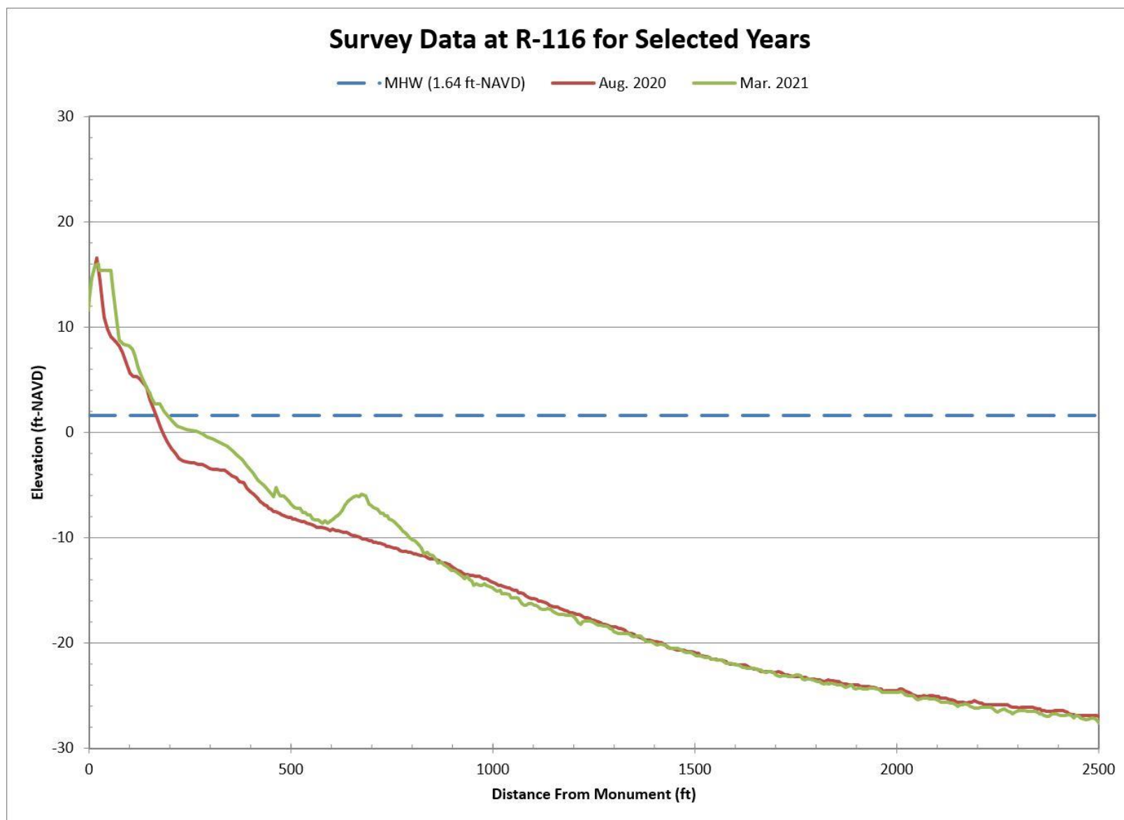
Figure B-37. Aug. 2020 Pre-Construction vs. Mar. 2021 Post-Construction Beach Profiles Along R-116
