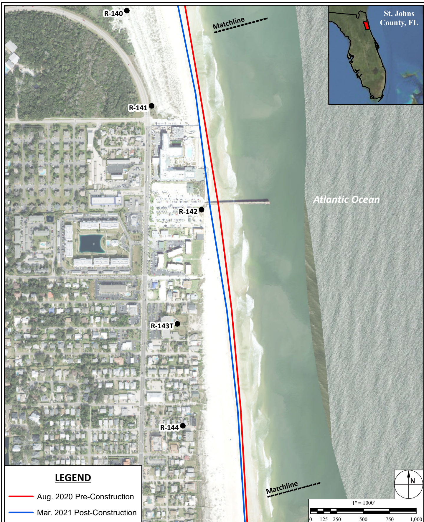
Figure C - 15 Mean High Water Contour Position South Ponte Vedra and Vilano Beach Coastal Storm Risk Management Project
