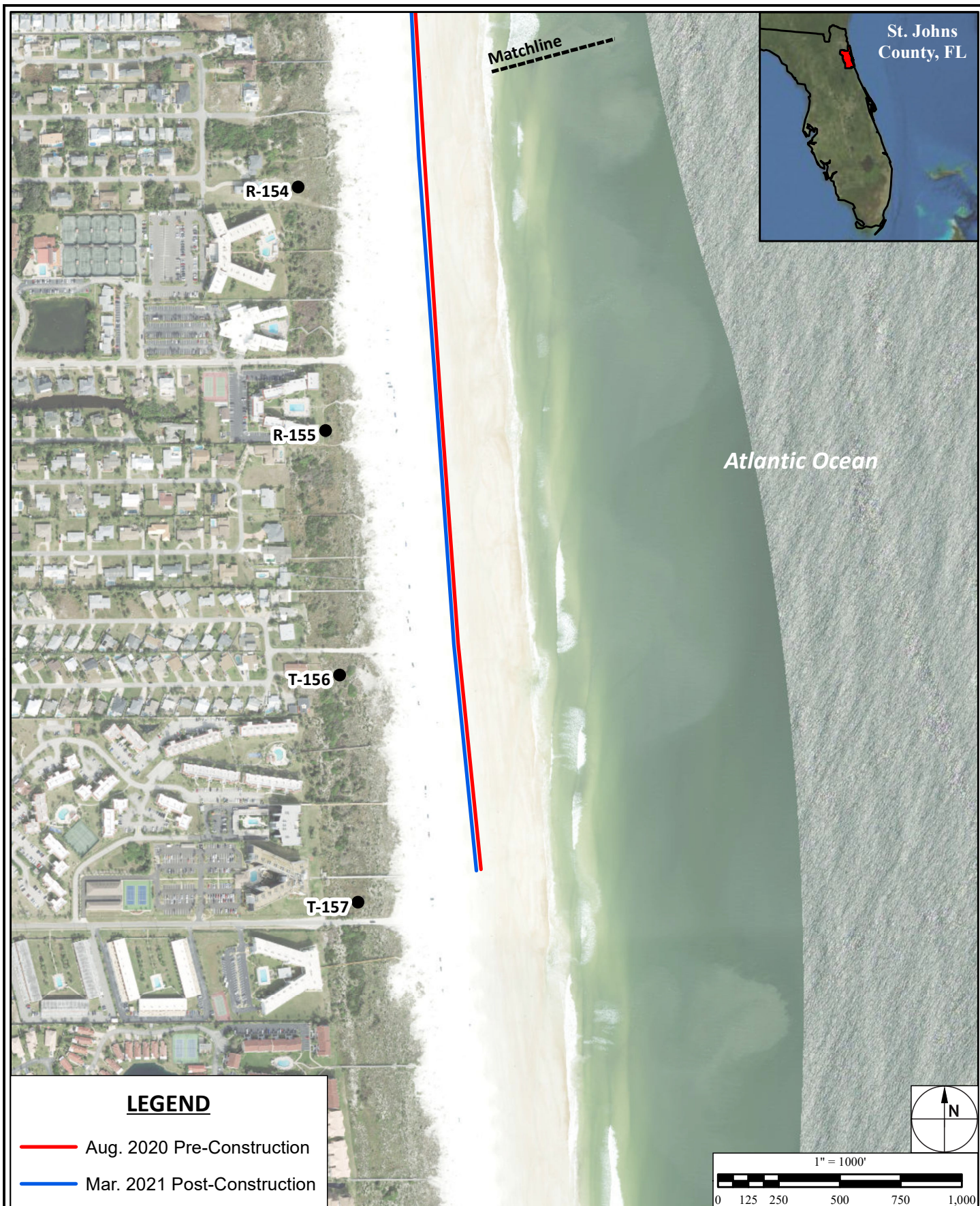
Figure C - 18 Mean High Water Contour Position South Ponte Vedra and Vilano Beach Coastal Storm Risk Management Project
