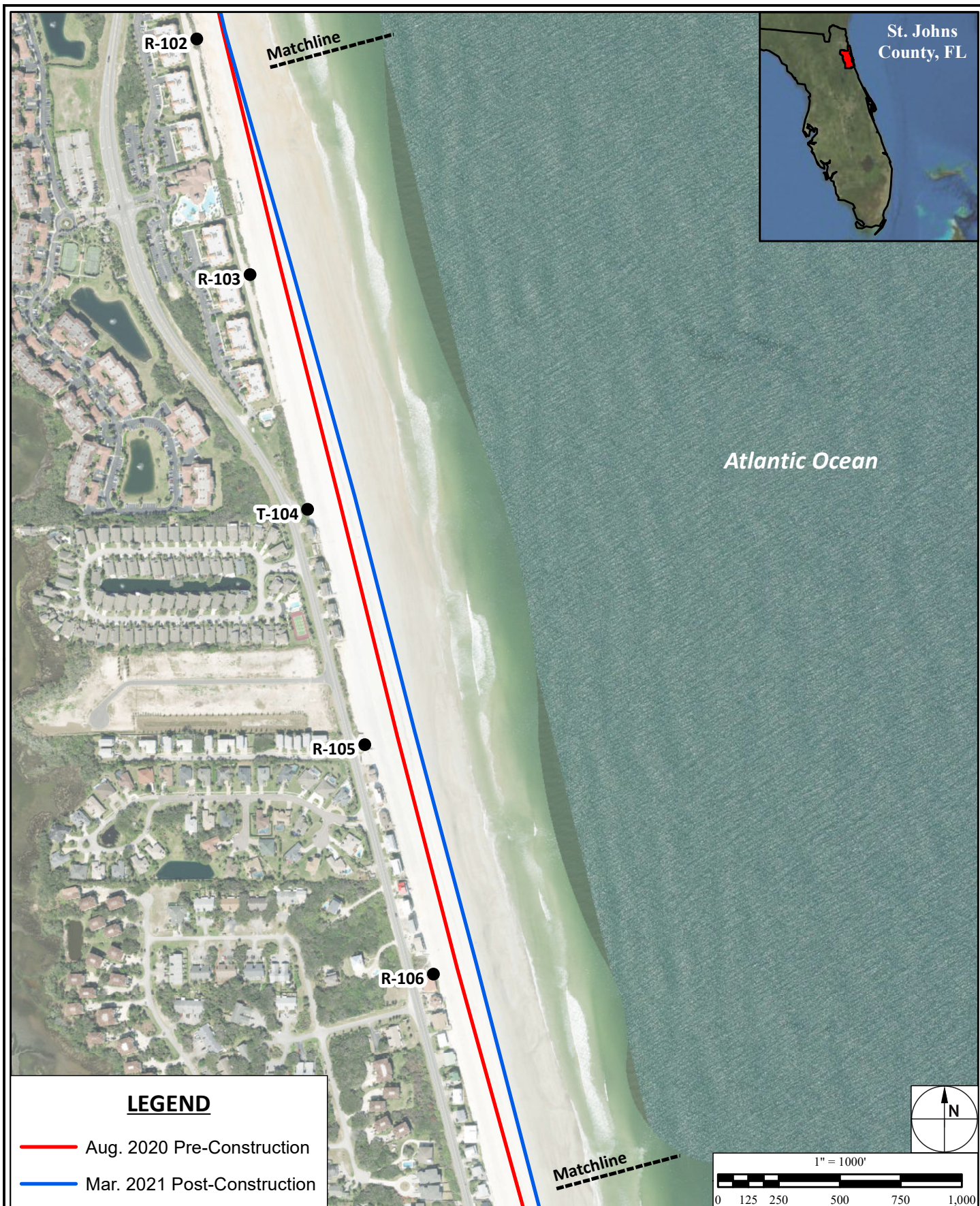
Figure C - 6 Mean High Water Contour Position South Ponte Vedra and Vilano Beach Coastal Storm Risk Management Project
