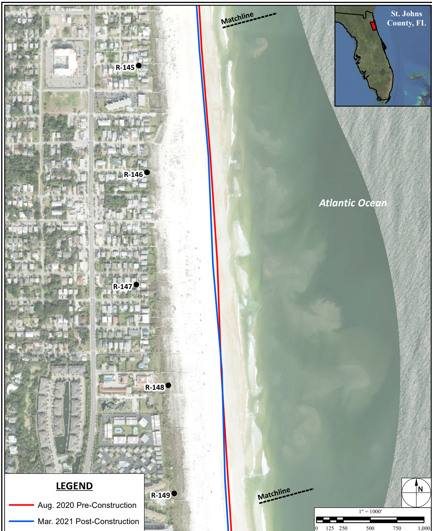
Figure C - 16 Mean High Water Contour Position South Ponte Vedra and Vilano Beach Coastal Storm Risk Management Project
