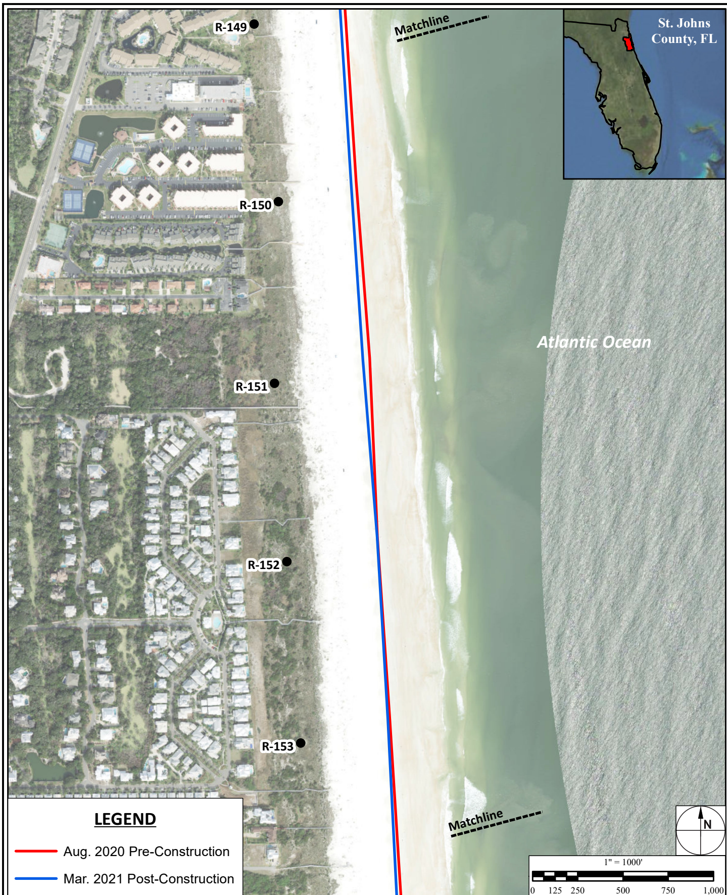
Figure C - 17 Mean High Water Contour Position South Ponte Vedra and Vilano Beach Coastal Storm Risk Management Project
