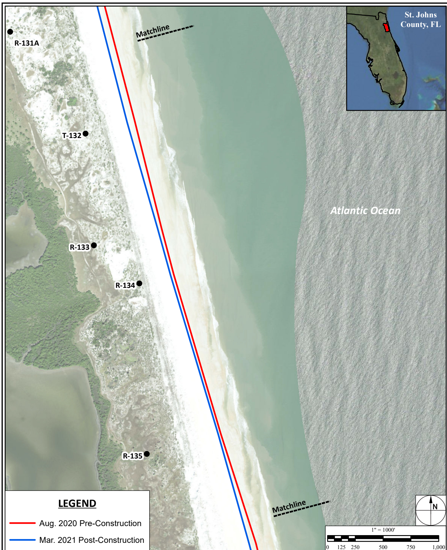
Figure C - 13 Mean High Water Contour Position South Ponte Vedra and Vilano Beach Coastal Storm Risk Management Project
