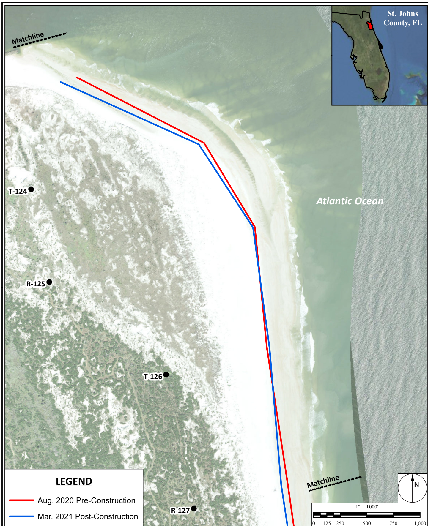
Figure C - 11 Mean High Water Contour Position South Ponte Vedra and Vilano Beach Coastal Storm Risk Management Project
