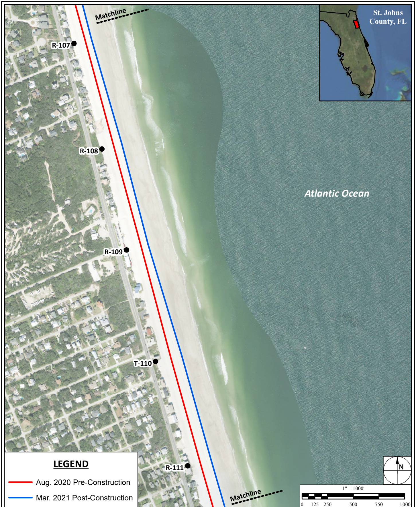
Figure C - 7 Mean High Water Contour Position South Ponte Vedra and Vilano Beach Coastal Storm Risk Management Project
