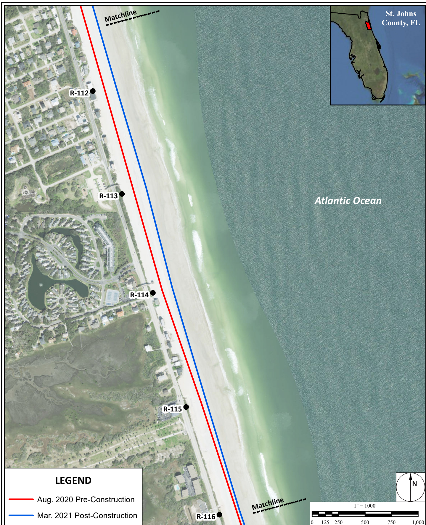
Figure C - 8 Mean High Water Contour Position South Ponte Vedra and Vilano Beach Coastal Storm Risk Management Project
