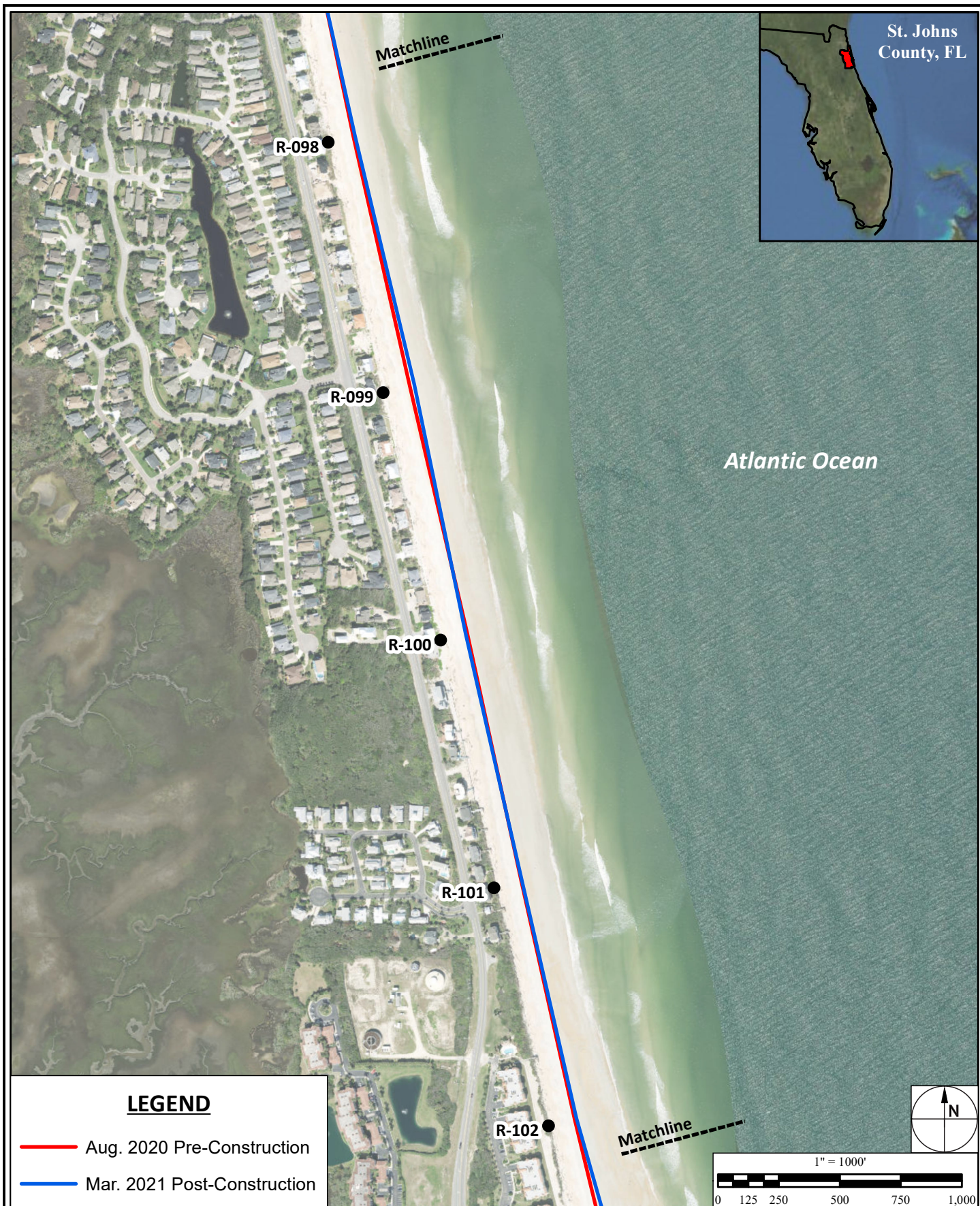
Figure C - 5 Mean High Water Contour Position South Ponte Vedra and Vilano Beach Coastal Storm Risk Management Project
