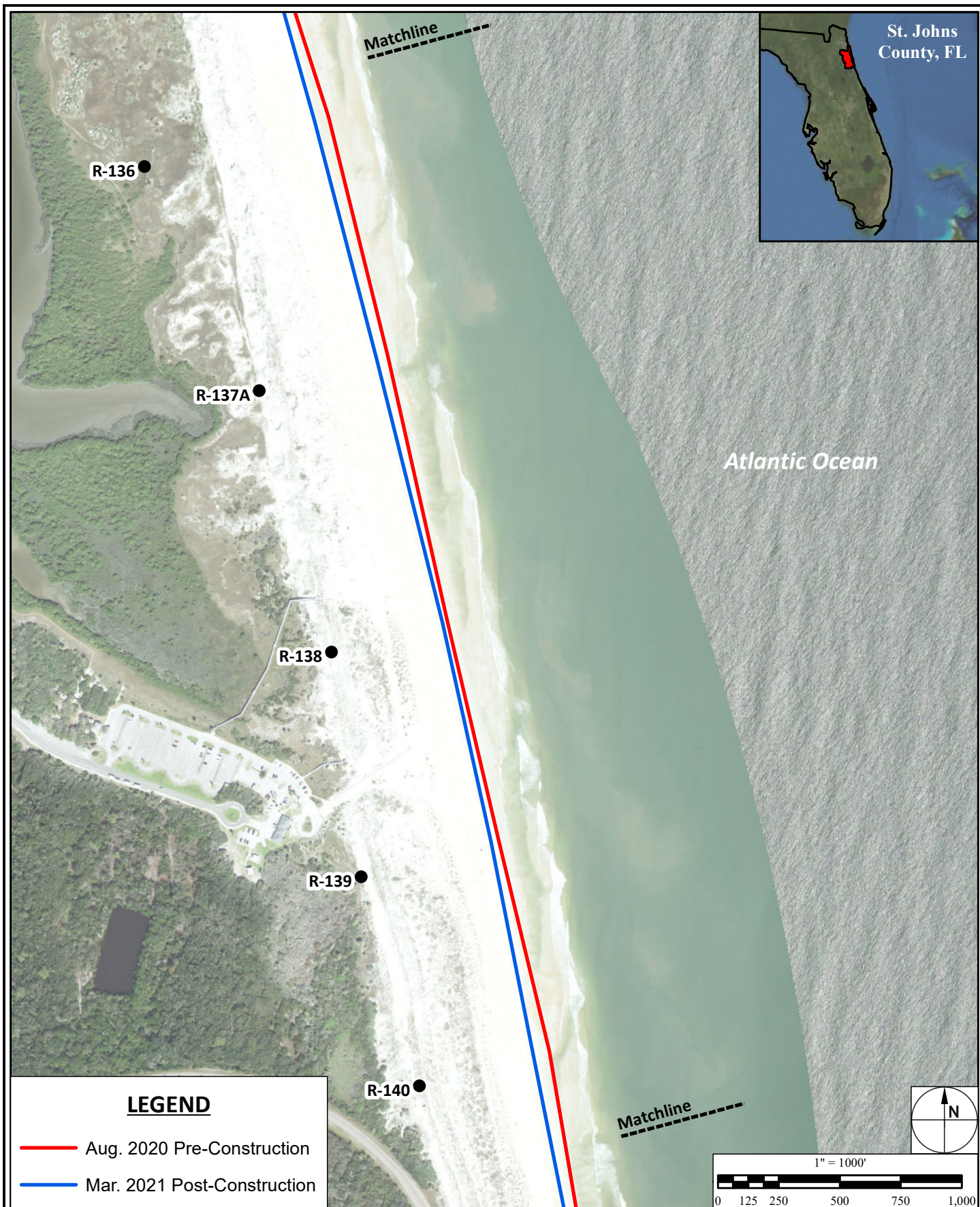
Figure C - 14 Mean High Water Contour Position South Ponte Vedra and Vilano Beach Coastal Storm Risk Management Project
