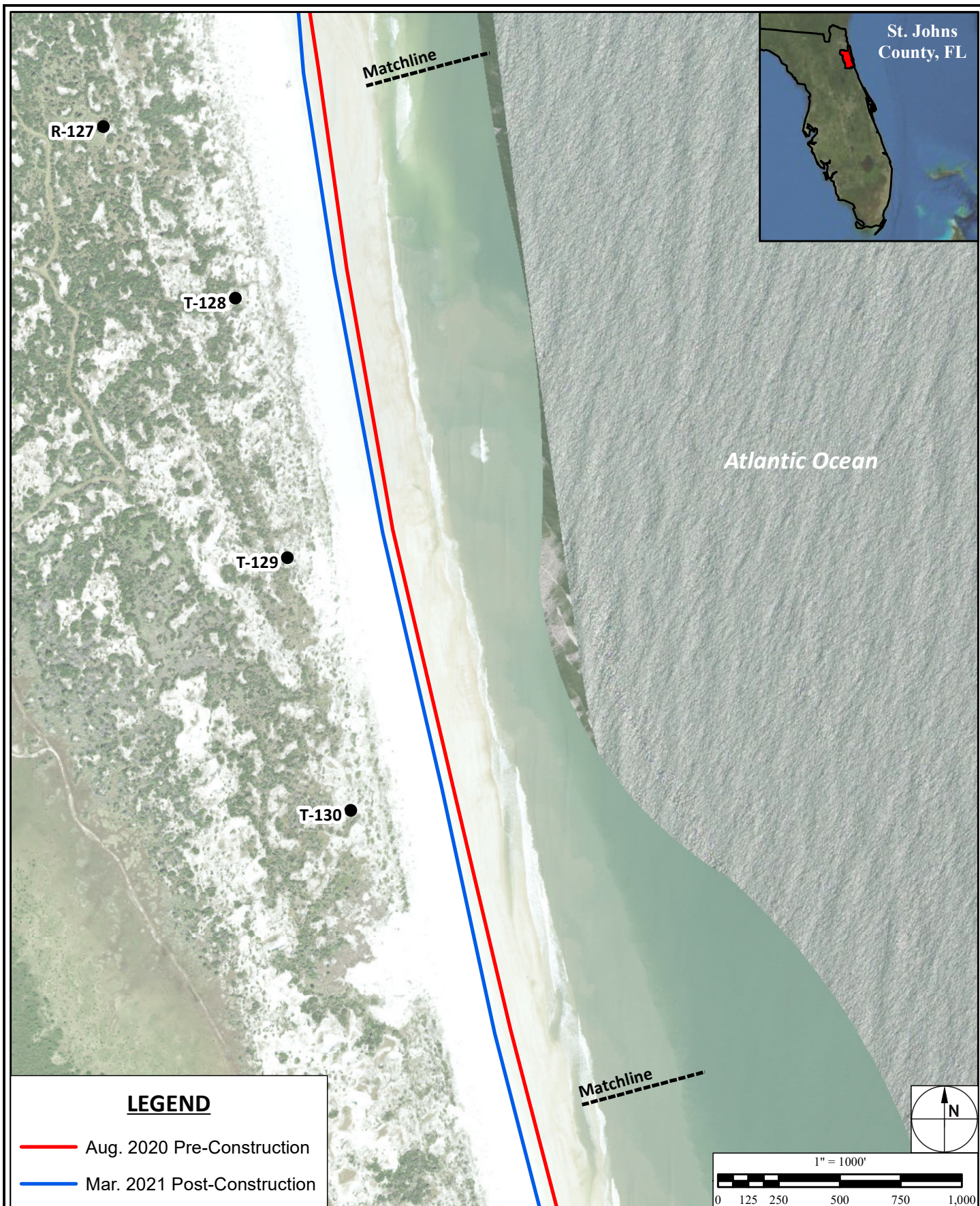
Figure C - 12 Mean High Water Contour Position South Ponte Vedra and Vilano Beach Coastal Storm Risk Management Project
