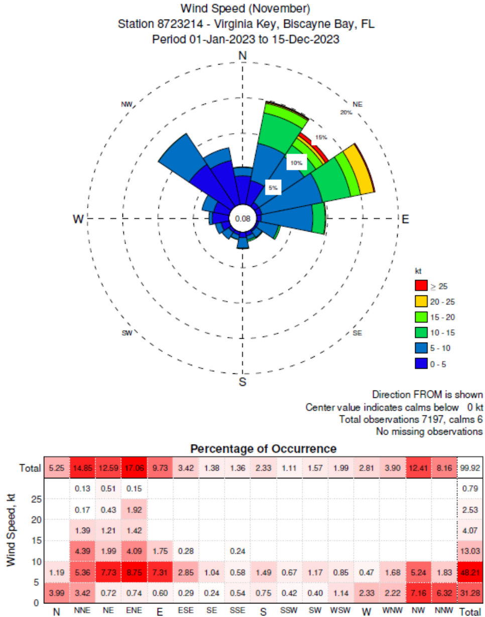
Figure 3. Wind Rose from NOAA Tidal Station 8722314 Virginia Key, Biscayne Bay, FL
