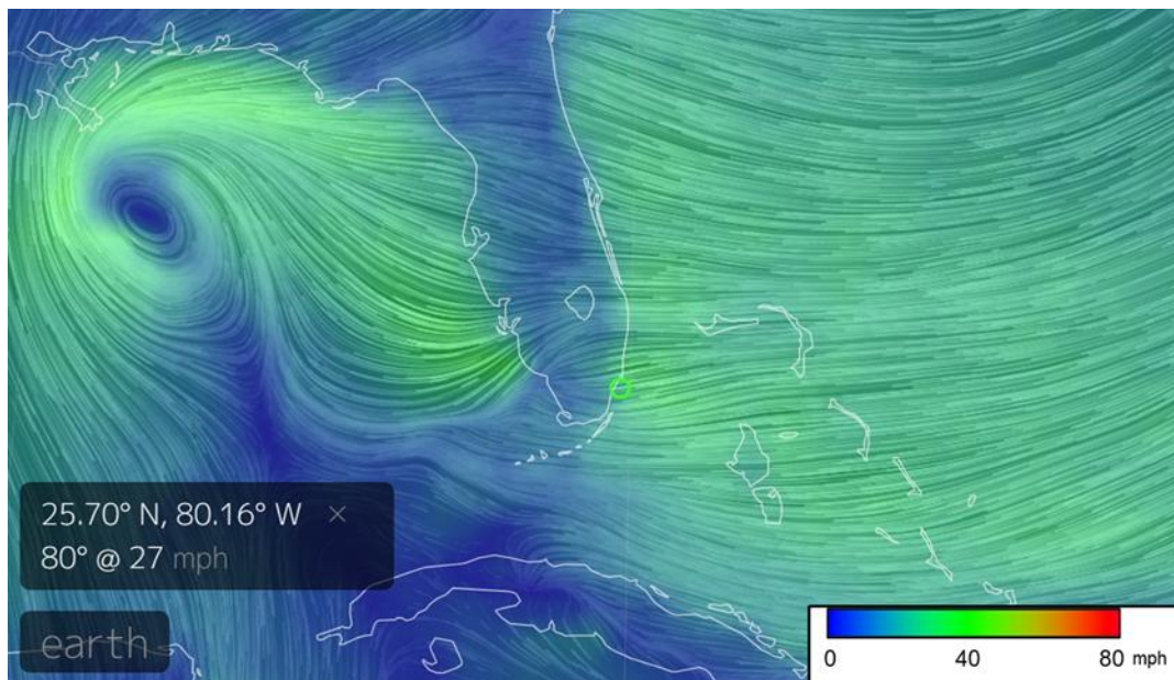
Figure 5. Visualization of Wind Conditions on November 15 th , 2023 provided by Earth.Nullschool.net
