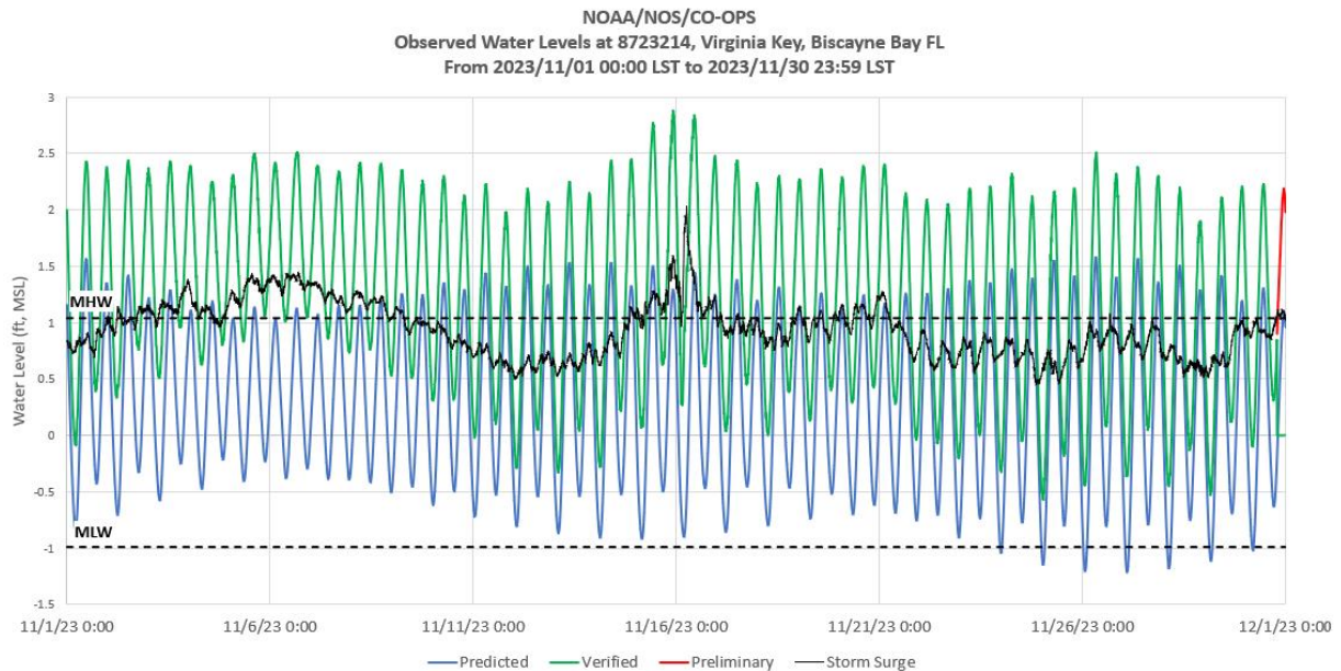
Figure 1. Predicted vs. Preliminary Water Levels and Estimated Storm Surge at NOAA Tidal Station 8723214, Virginia Key, Biscayne Bay, FL for November 2023
