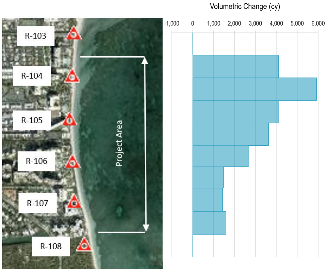
FIGURE 6: VOLUMETRIC CHANGES ABOVE THE DOC (CY) – PRE-CON VS IMMEDIATE POST-CON SURVEYS
