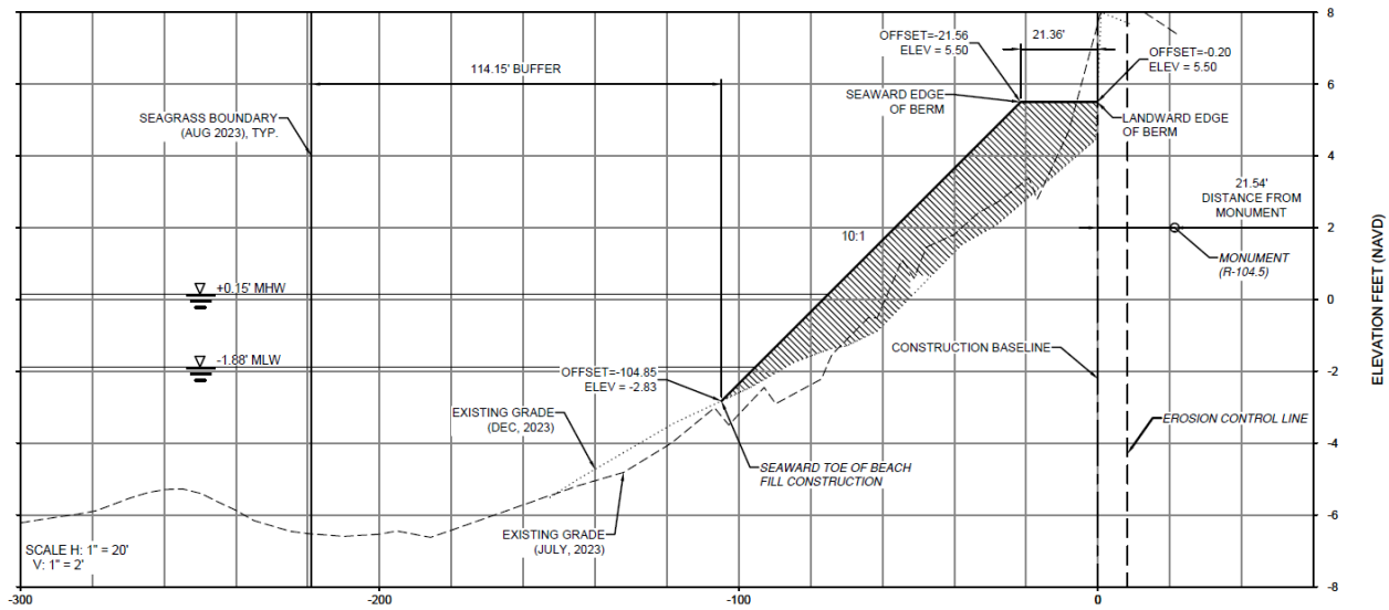
Figure 9. Beach Profile Comparison at R-104.5 and Revised Fill Volume (7.01 cy/ft)
