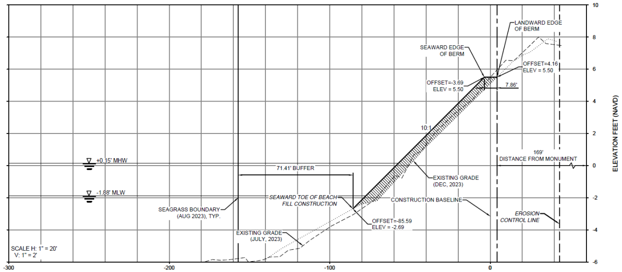
Figure 14. Beach Profile Comparison R-107 and Revised Fill Volume (2.32 cy/ft)
