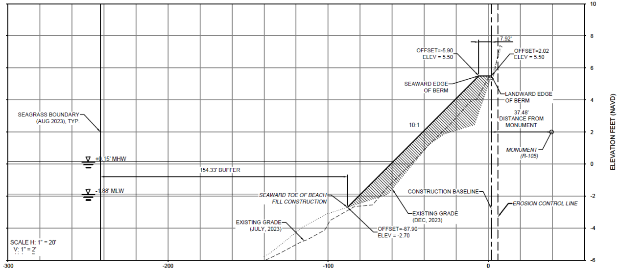
Figure 10. Beach Profile Comparison at R-105 and Revised Fill Volume (4.73 cy/ft)
