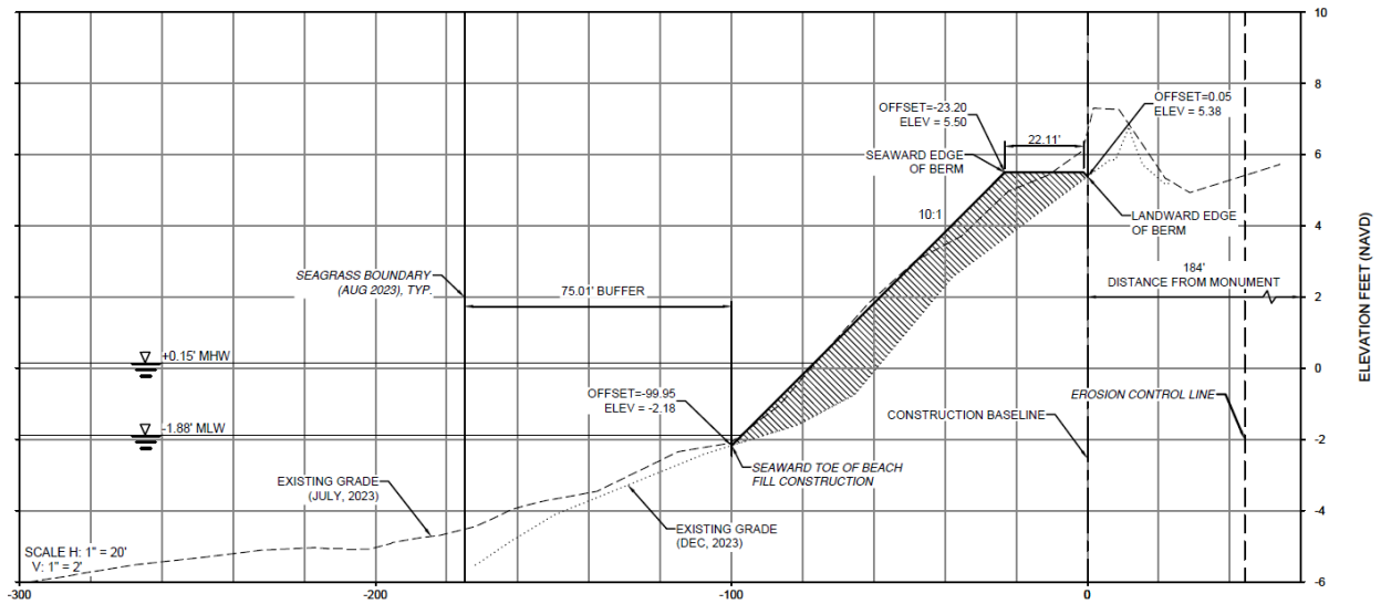
Figure 15. Beach Profile Comparison R-107.5 and Revised Fill Volume (4.95 cy/ft)
