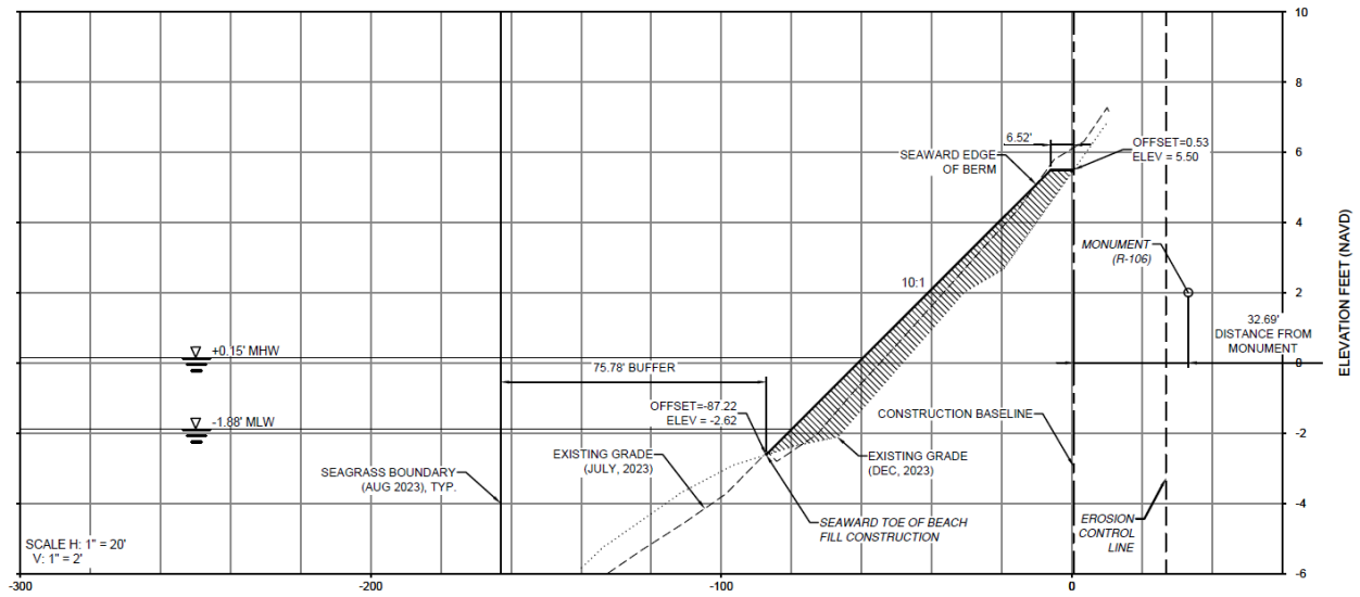
Figure 12. Beach Profile Comparison at R-106 and Revised Fill Volume (3.49 cy/ft)
