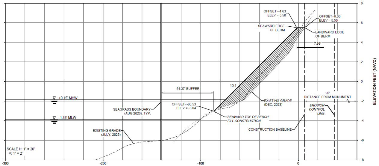
Figure 13. Beach Profile Comparison R-106.5 and Revised Fill Volume (4.79 cy/ft)
