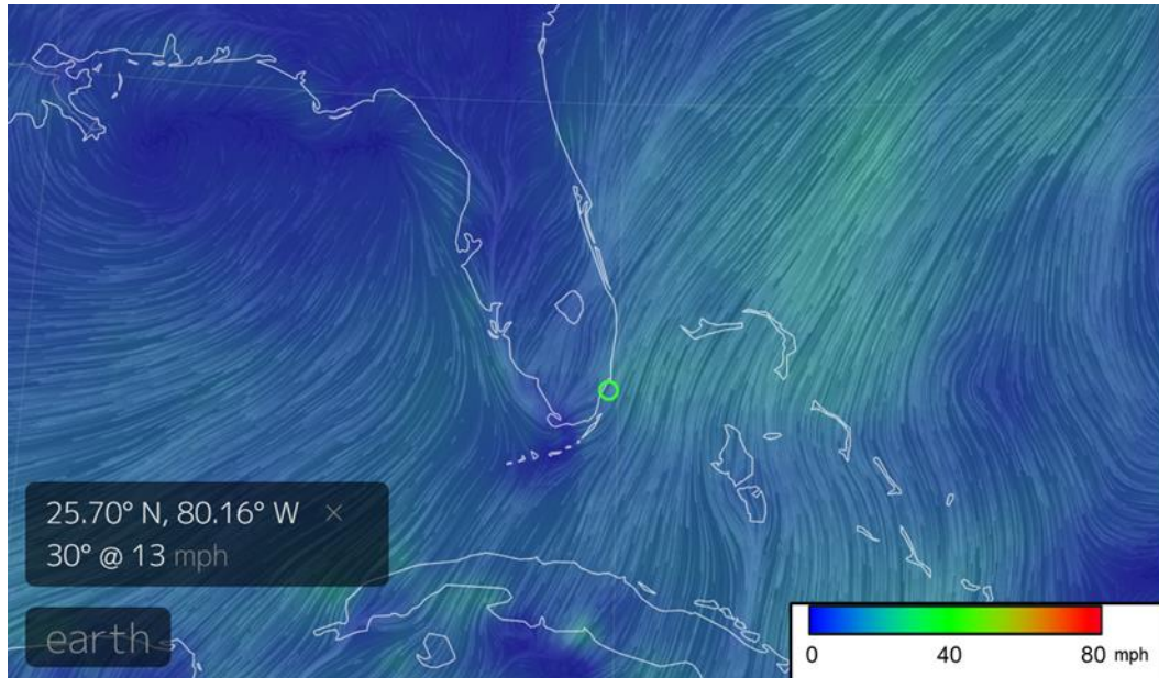
Figure 4. Visualization of Wind Conditions on November 6 th , 2023 provided by Earth.Nullschool.net
