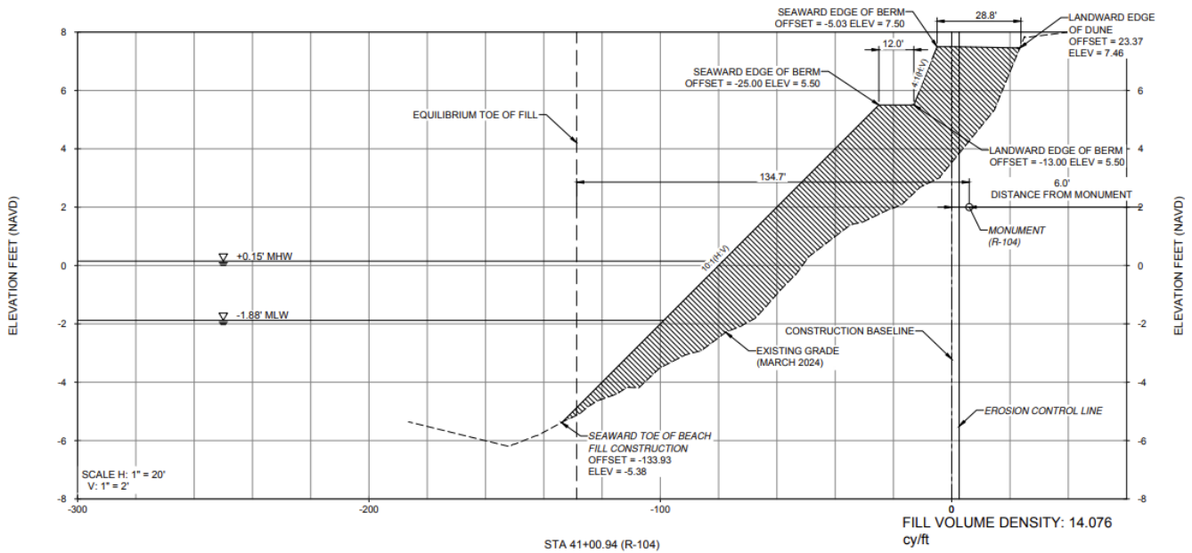
FIGURE 4: EXAMPLE OF IN-WATER SEDIMENT PLACEMENT
