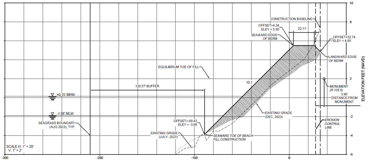
Figure 11. Beach Profile Comparison at R-105.5 and Revised Fill Volume (7.86 cy/ft)
