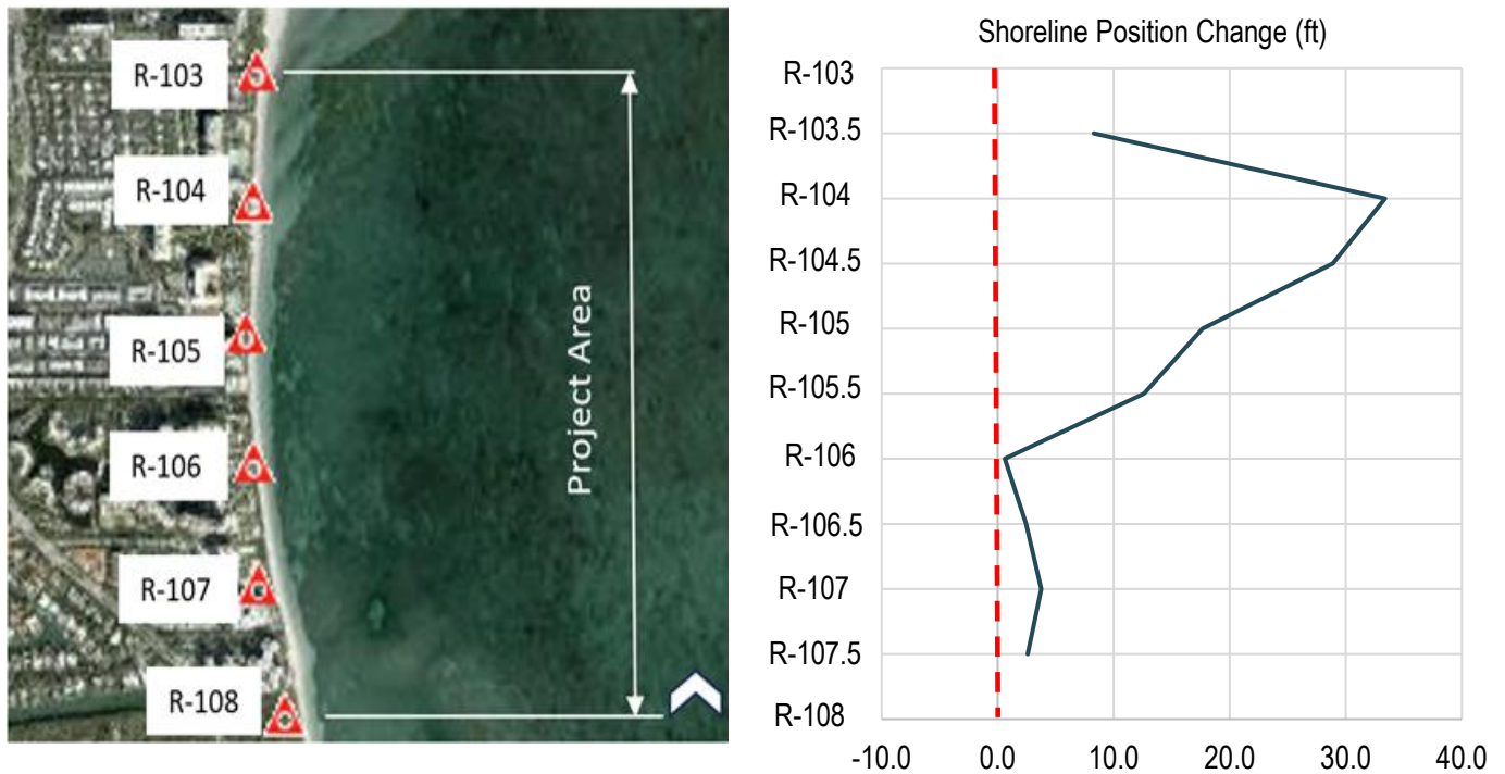
FIGURE 5: SHORELINE POSITION CHANGE AT MHW (FT) – PRE-CON VS IMMEDIATE POST-CON SURVEYS
