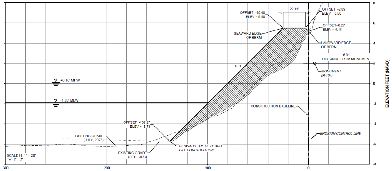
Figure 8. Beach Profile Comparison at R-104 and Revised Fill Volume (11.49 cy/ft)
