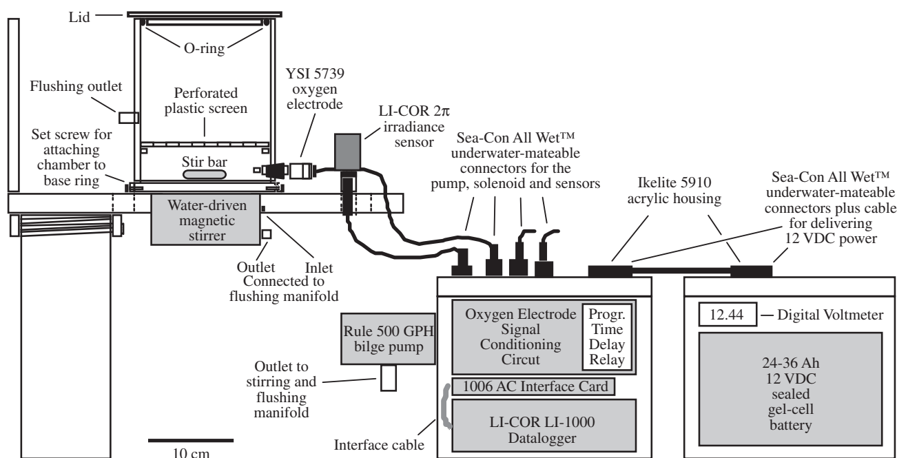
Fig. 1. Computer controlled respirometry system (only 1 of 6 chambers is shown). 500 GPH: bilge pump rate in gallons \text{h}^{-1} (= 1895 l \text{h}^{-1} ); Ah: ampere-hour; VDC: volt direct current; Progr.: programmable
