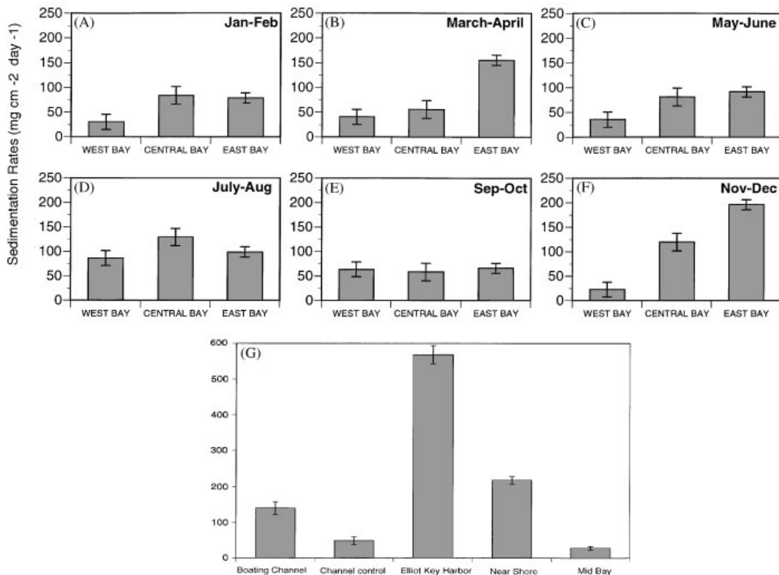
Figure 3. (A)–(F) Mean sedimentation rates (mg cm -2 day -1 ) for sites within Biscayne Bay during 2001. Values represent averages from three sites within each stratum. Four PVC sedimentation columns were deployed at each site. (G) Mean sedimentation rates (mg cm -2 day -1 ) for locations influenced by boating activities. Values represent averages from four sedimentation columns at each location deployed from March 28 to Monday, March 31, 2001. For site locations refer to Figure 1.
