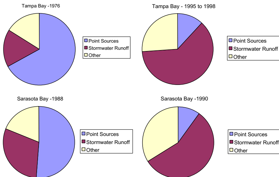
Fig. 2. Sources of nitrogen loads (kg TN year -1 ) for Tampa Bay in 1976 and the 1995–1998 annual average, and for Sarasota Bay in 1988 and 1990. “Point Sources” includes both industrial sites and domestic wastewater treatment plants. “Stormwater Runoff” includes both gaged and ungaged surface flows. “Other” includes atmospheric deposition, baseflow, septic tank systems, etc. (see materials and methods for details). Data are summarized from Pribble et al. (2001) for Tampa Bay, and summarized from Tomasko et al. (1996) for Sarasota Bay.
