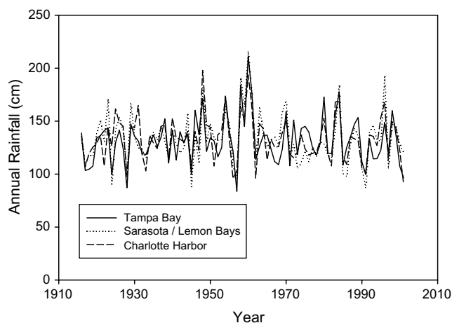
Fig. 3. Annual rainfall (cm year -1 ) for pooled data from gages within the watersheds of Tampa Bay, Sarasota Bay plus Lemon Bay, and Upper Charlotte Harbor from 1916 to 2001. Data from SWFWMD.
