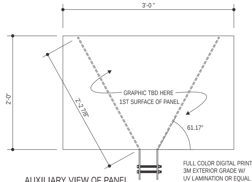
AUXILIARY VIEW OF PANEL SCALE: 1" = 1'-0"
