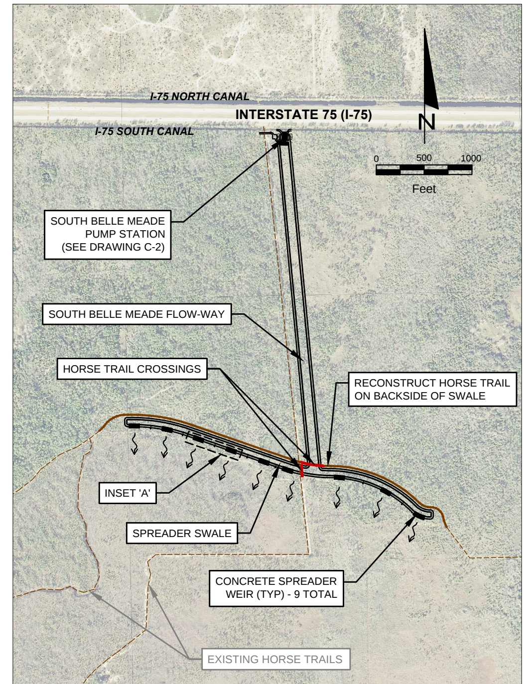
PLAN VIEW
