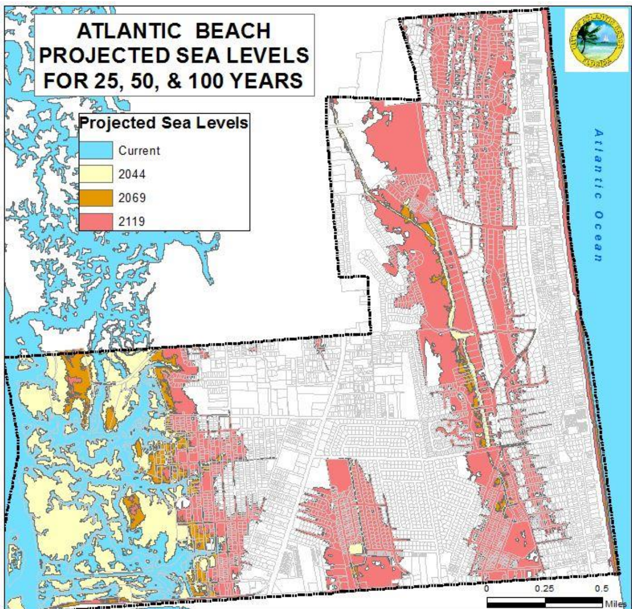
Figure 3-1– NOAA 2017 Intermediate-High SLR Projects for 2044, 2069 and 2119
