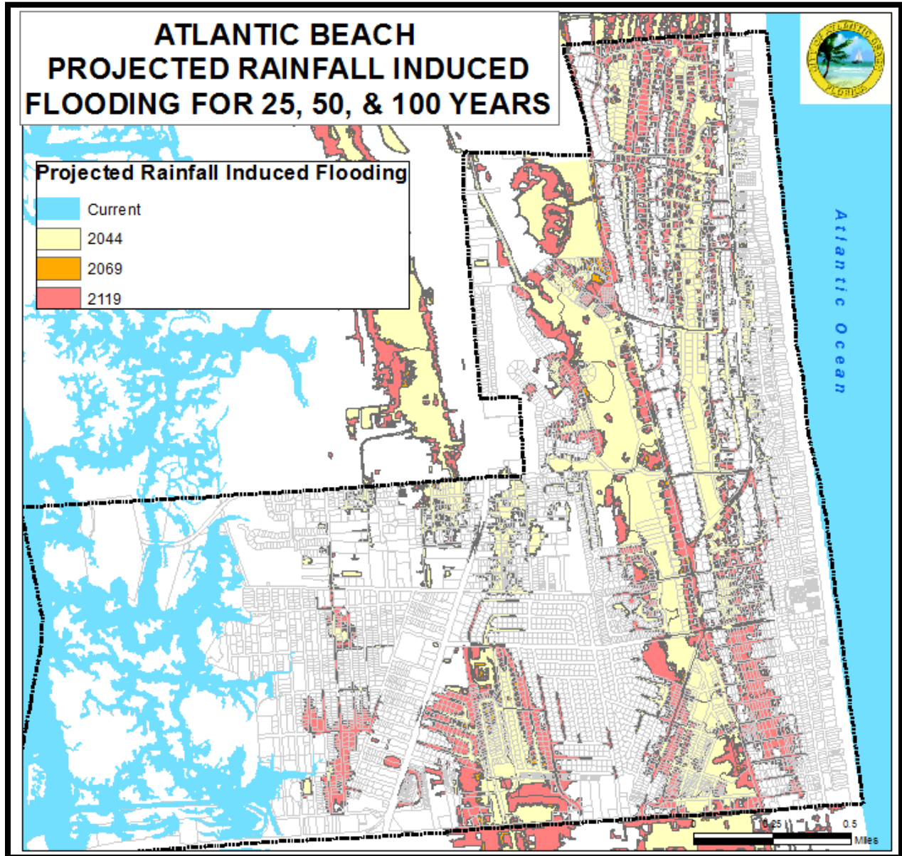
Figure 3-4 – Projected 100-Year Storm Event Rainfall Induced Flooding
