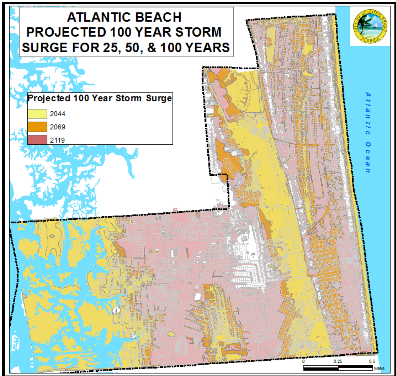
Figure 3-3 – Projected 100-Year Event Storm Surge
