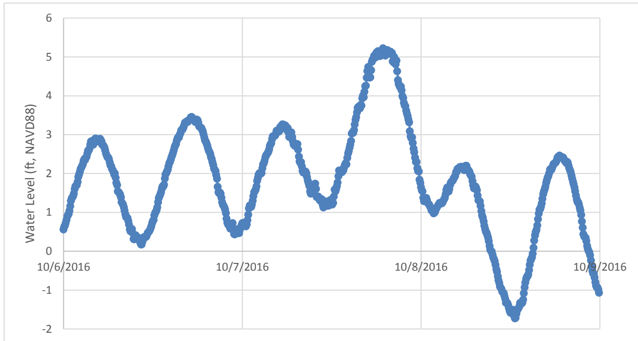
Figure 2-2 – Hurricane Matthew Water Levels - October 2016 at Mayport Bar Pilot's Dock
