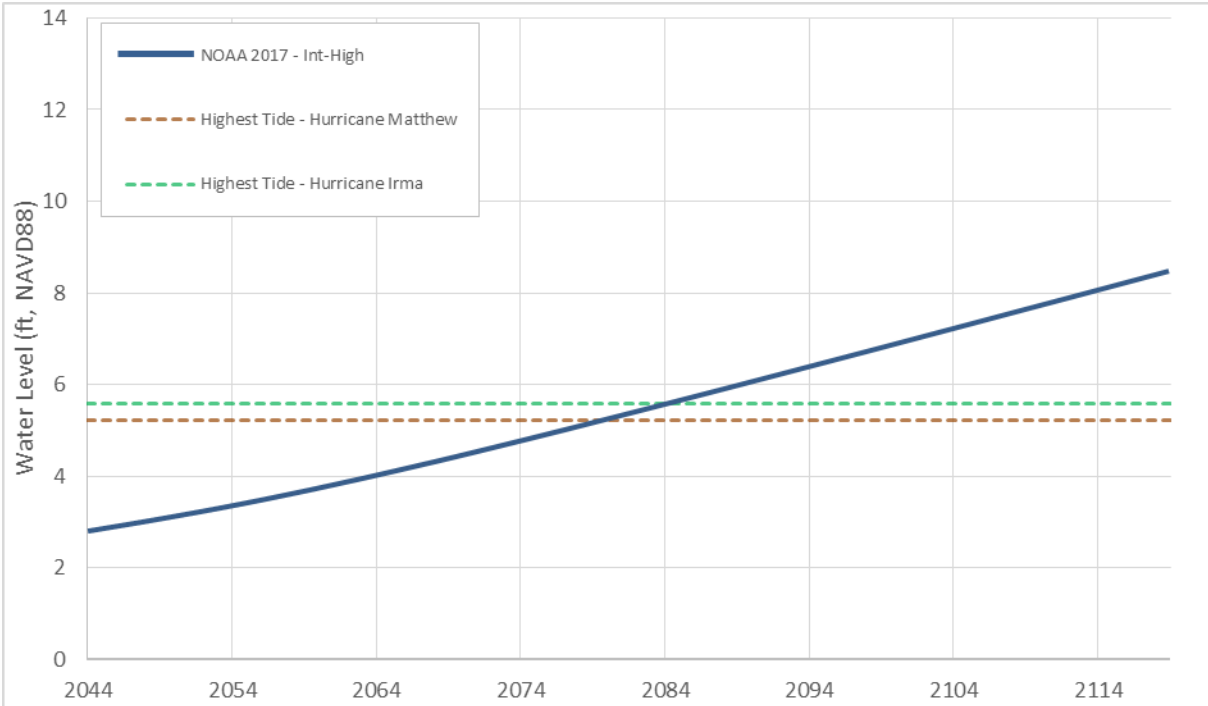
Figure 2-4 – Comparison of Matthew and Irma Water Levels with Projected Mean SLR
