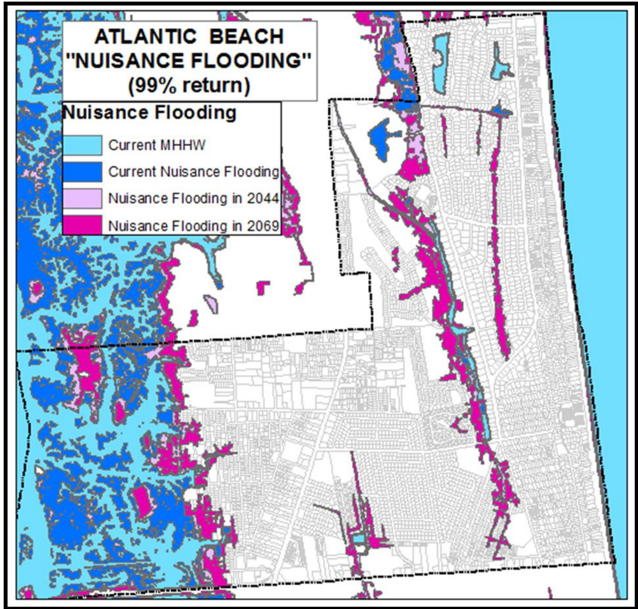
Figure 3-2 – Projected Nuisance Flooding Due to SLR
