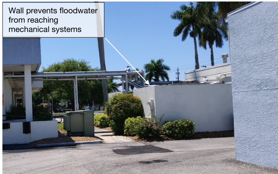
Photograph 4.12 Dry Floodproofed Mechanical Systems at County Tax Collector's Office
