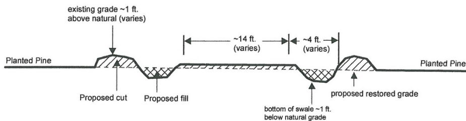
TYPICAL SECTION LOOKING WEST (from southern segment)
