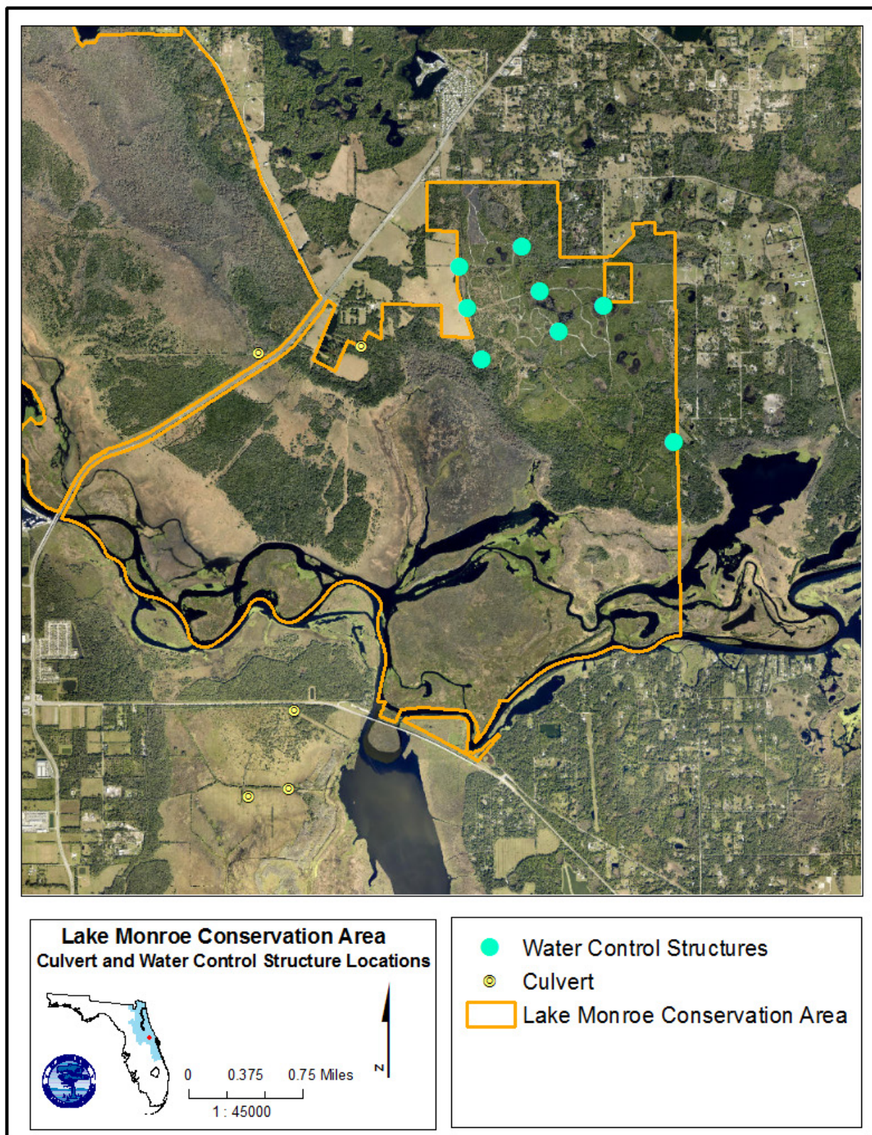
Figure 13: Culverts and Water Control Structures
