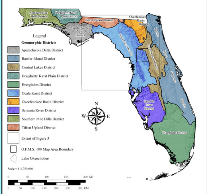
Figure 2. Geomorphic Districts (modified from Scott, 2005).
