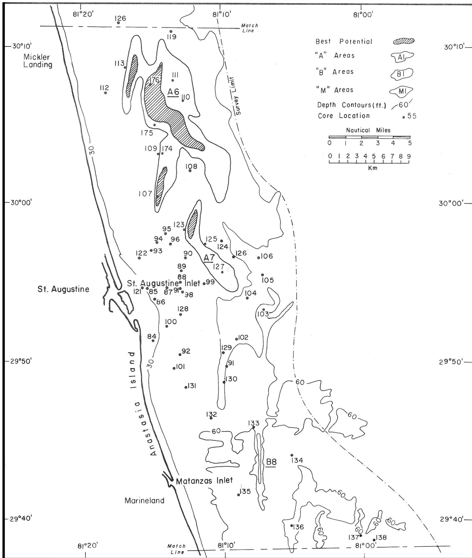
Figure 19. Potential offshore sand borrow areas between the Jacksonville area and Matanzas Inlet.
