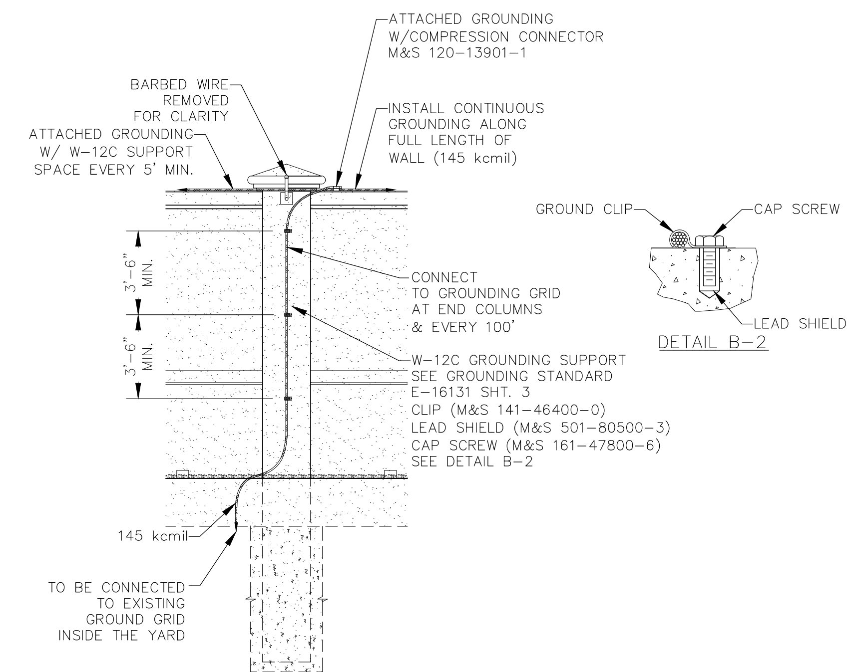
CONNECTION TO GROUNDING GRID DETAIL SCALE: 1/4"=1'-0"
