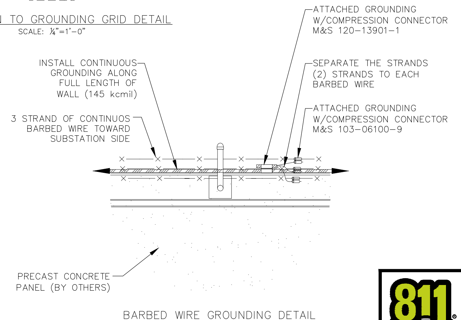
BARBED WIRE GROUNDING DETAIL NTS
