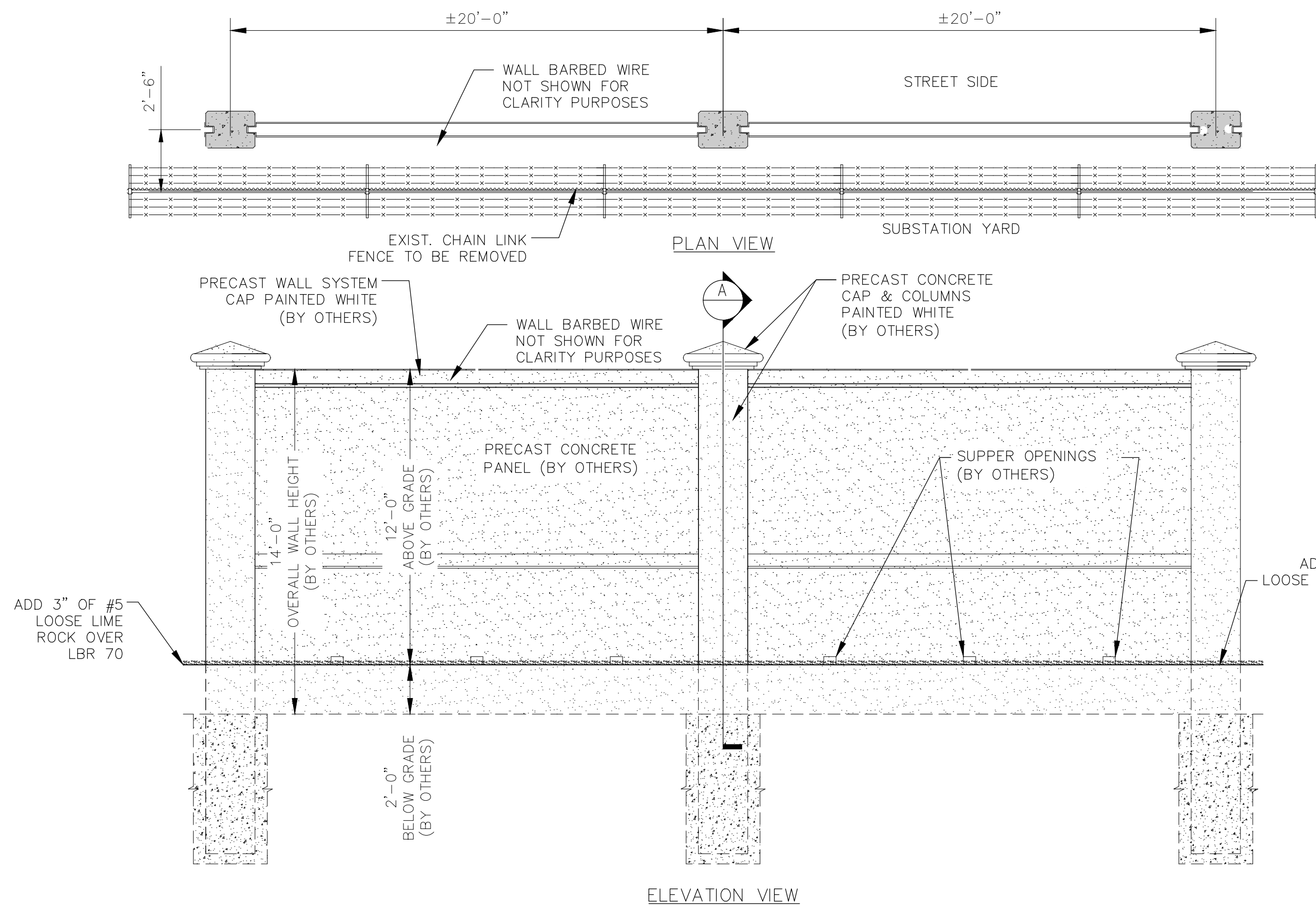
CHAIN LINK FENCE REMOVAL SCALE: 1/4"=1'-0"
