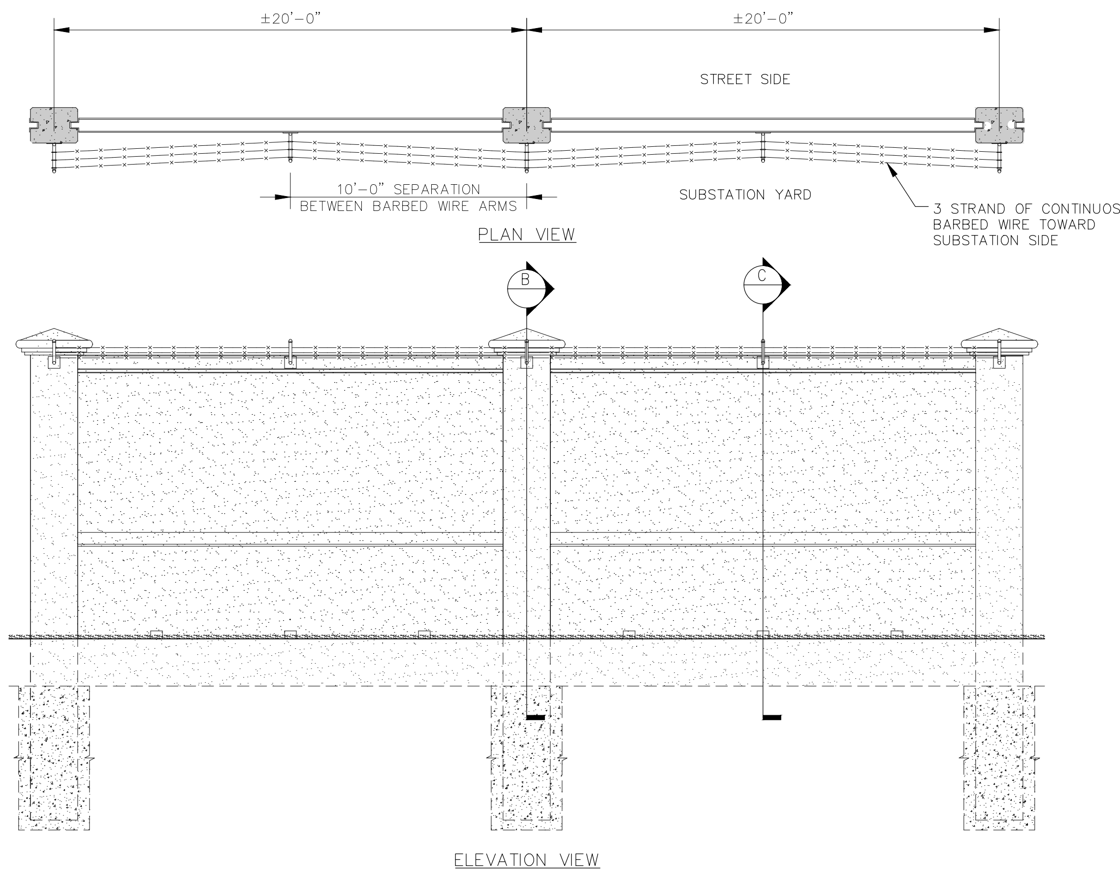
BARBED WIRE INSTALLATION SCALE: 1/4"=1'-0"
