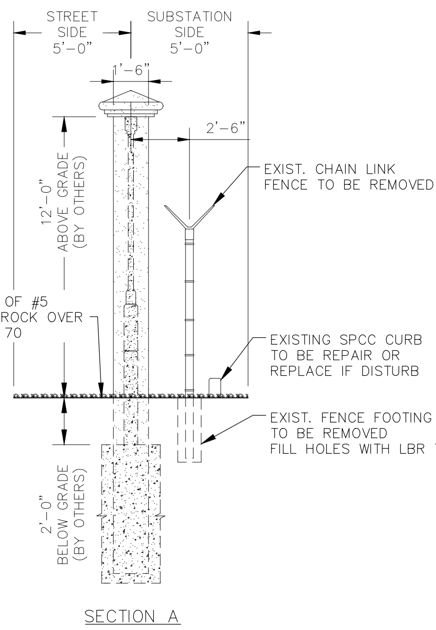
SECTION A
