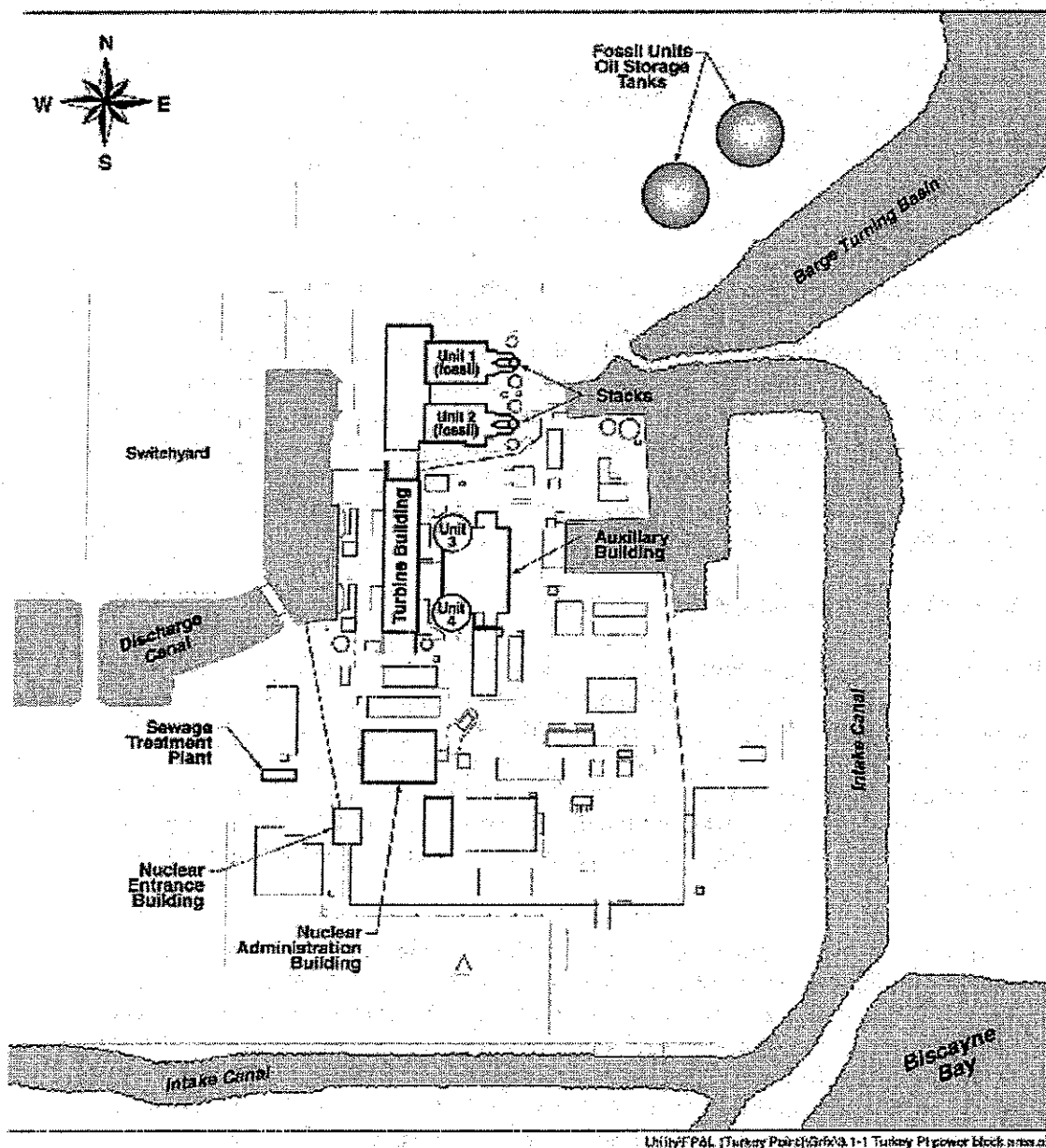
Figure 2-3. Turkey Point Site Powerblock Area
