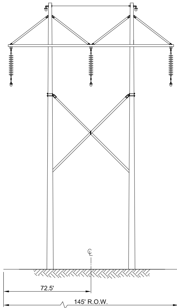
ORIGINAL STRUCTURE DESIGN
