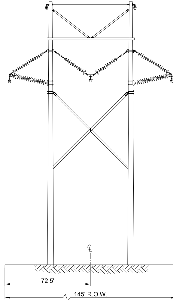
MODIFIED STRUCTURE DESIGN (T-MOD)
