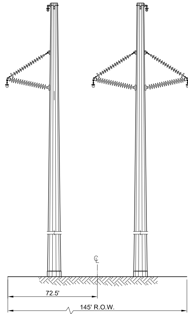
NEW 2-POLE STRUCTURE (TO BE USED AT STRUCTURES 38 TO 41 AND 43 TO 54)
