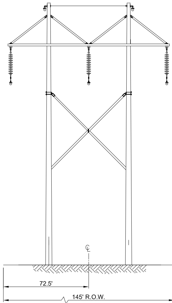
EXISTING H-FRAME STRUCTURE
