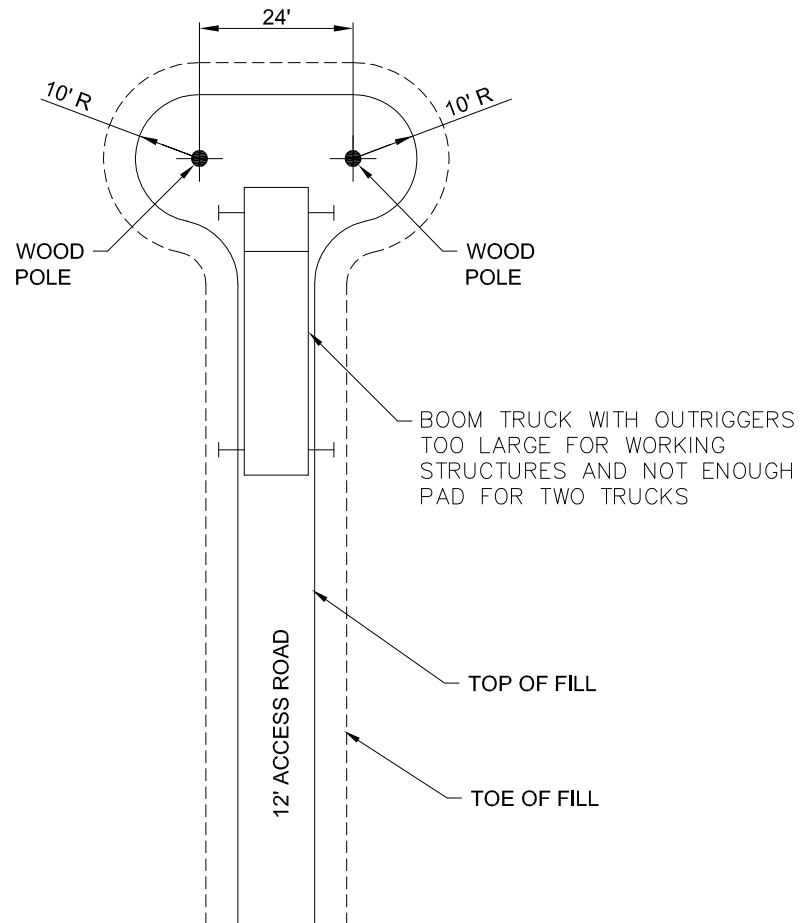
EXISTING ACCESS PAD WOOD H-FRAME STRUCTURES
