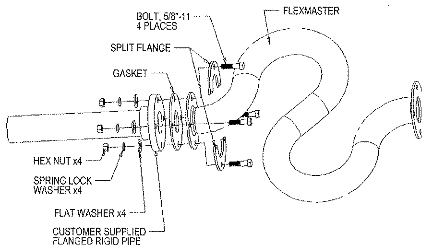
Figure 7.12 – Exploded Assembly
