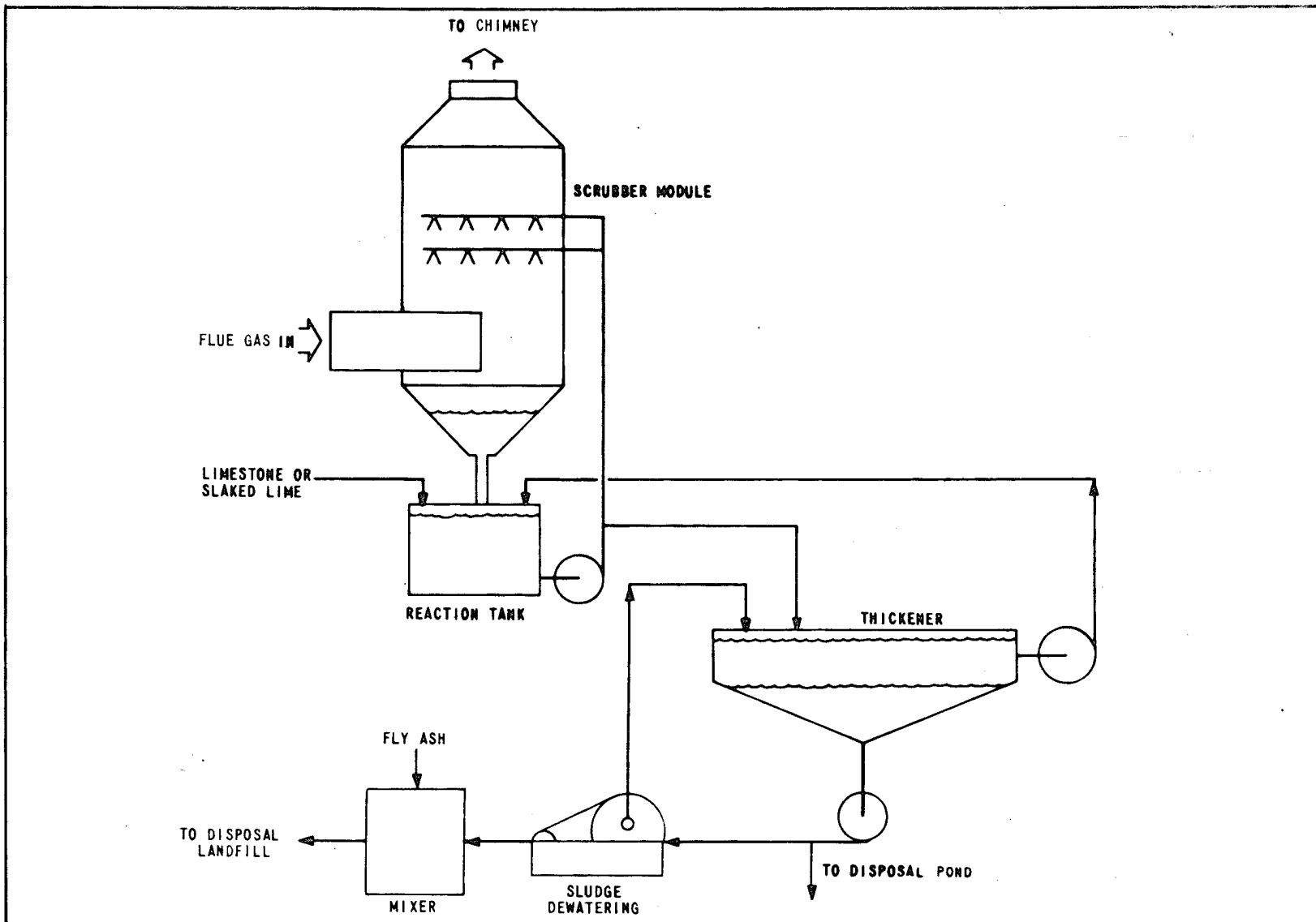
FIGURE 3.7B-3. LIME OR LIMESTONE PROCESS
