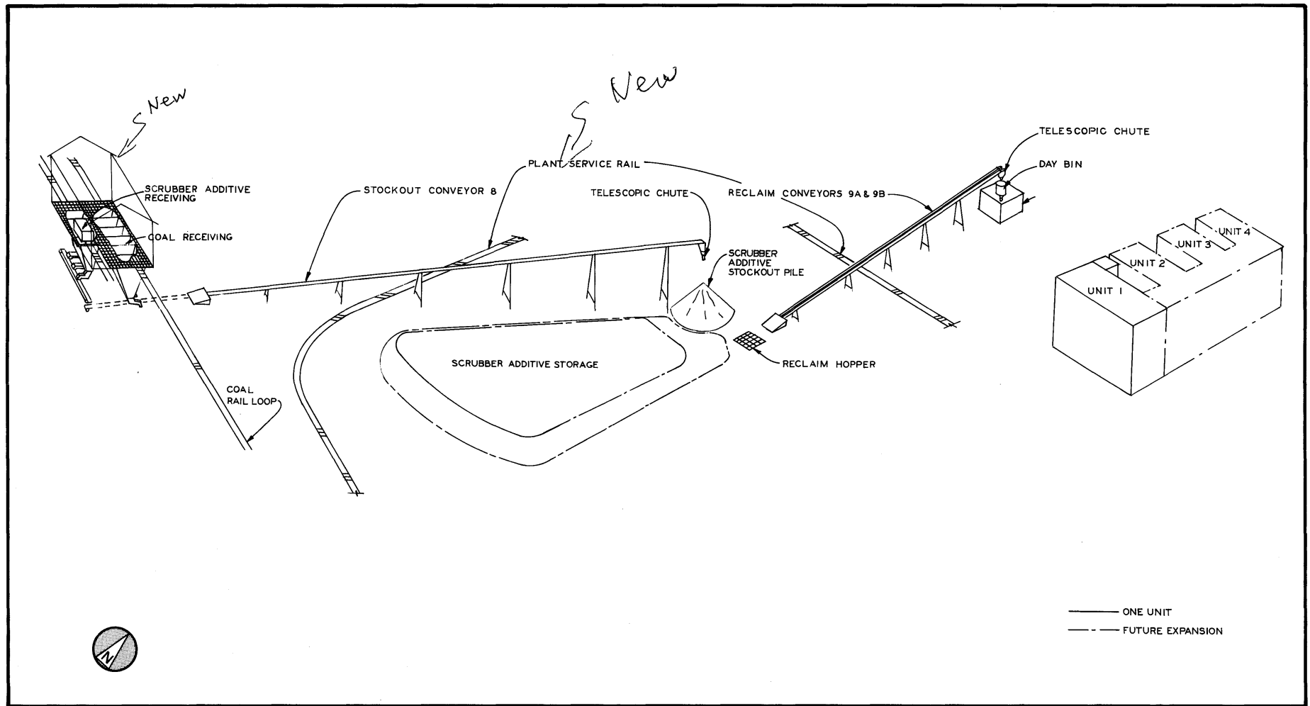
FIGURE 3.9-11. PERSPECTIVE OF SCRUBBER ADDITIVE HANDLING SYSTEM
