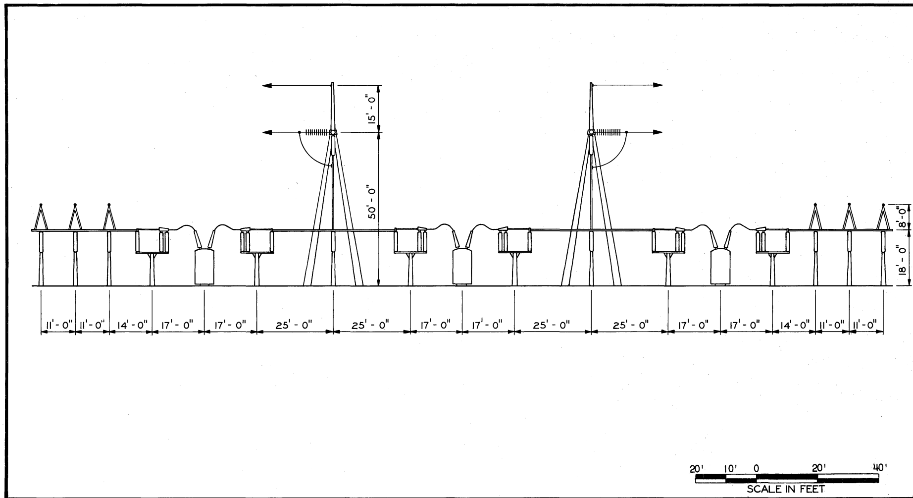
FIGURE 3.8-7. STANTON ENERGY CENTER SUBSTATION ELEVATION LOOKING WEST
