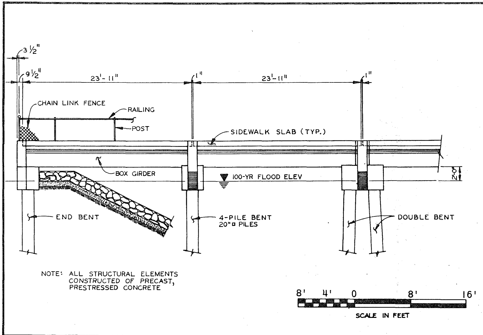
FIGURE 3.9-4. TYPICAL RAILROAD TRESTLE DETAIL
