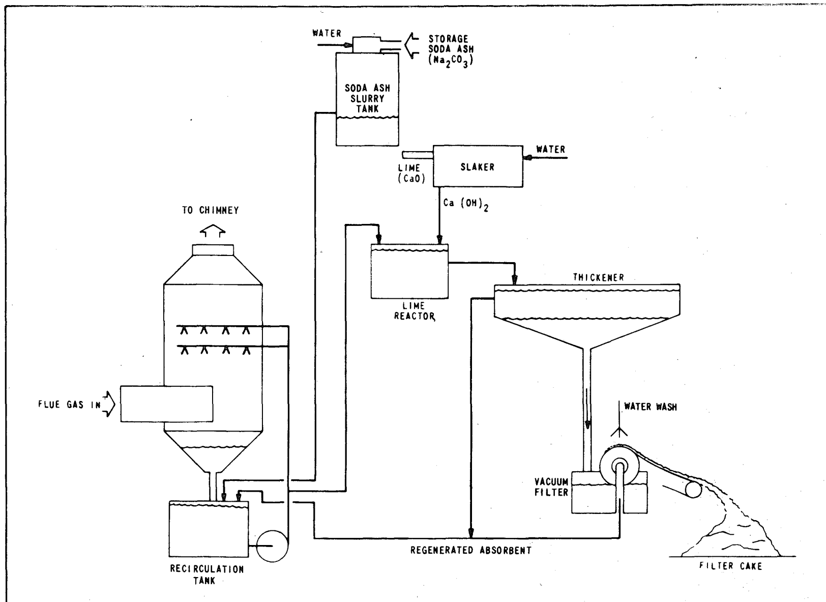
FIGURE 3.7B-5. DOUBLE-ALKALI PROCESS
