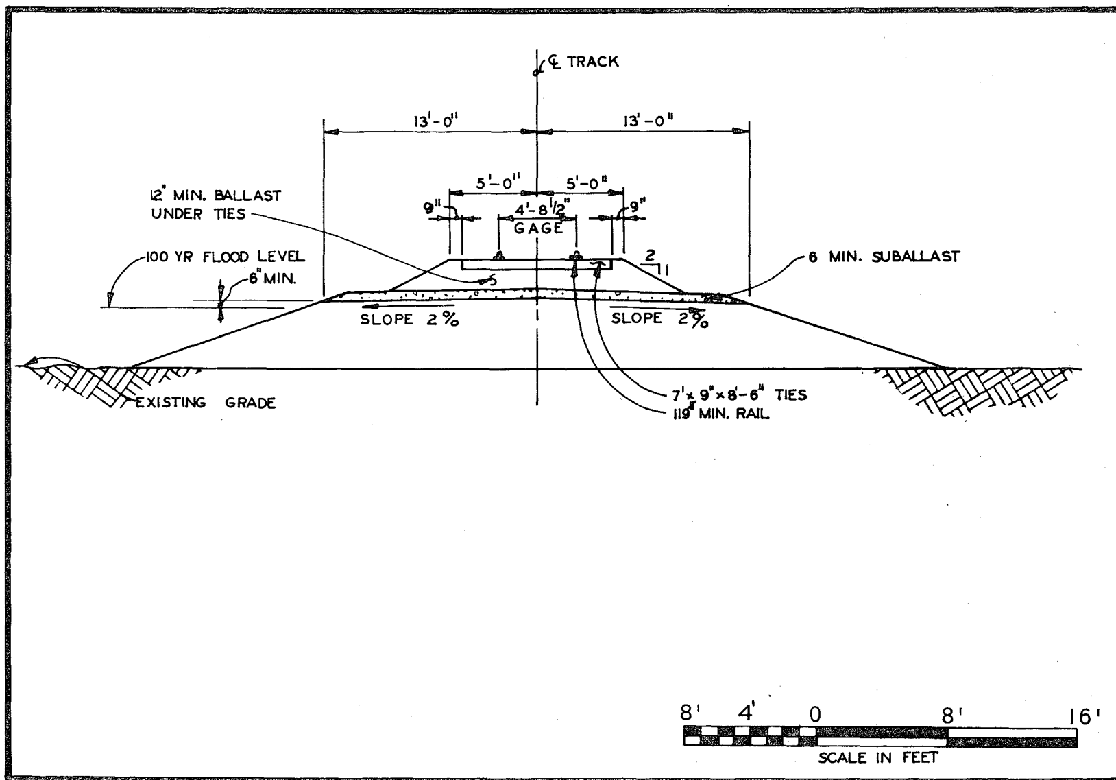
FIGURE 3.9-3. TYPICAL RAILROAD SECTION
