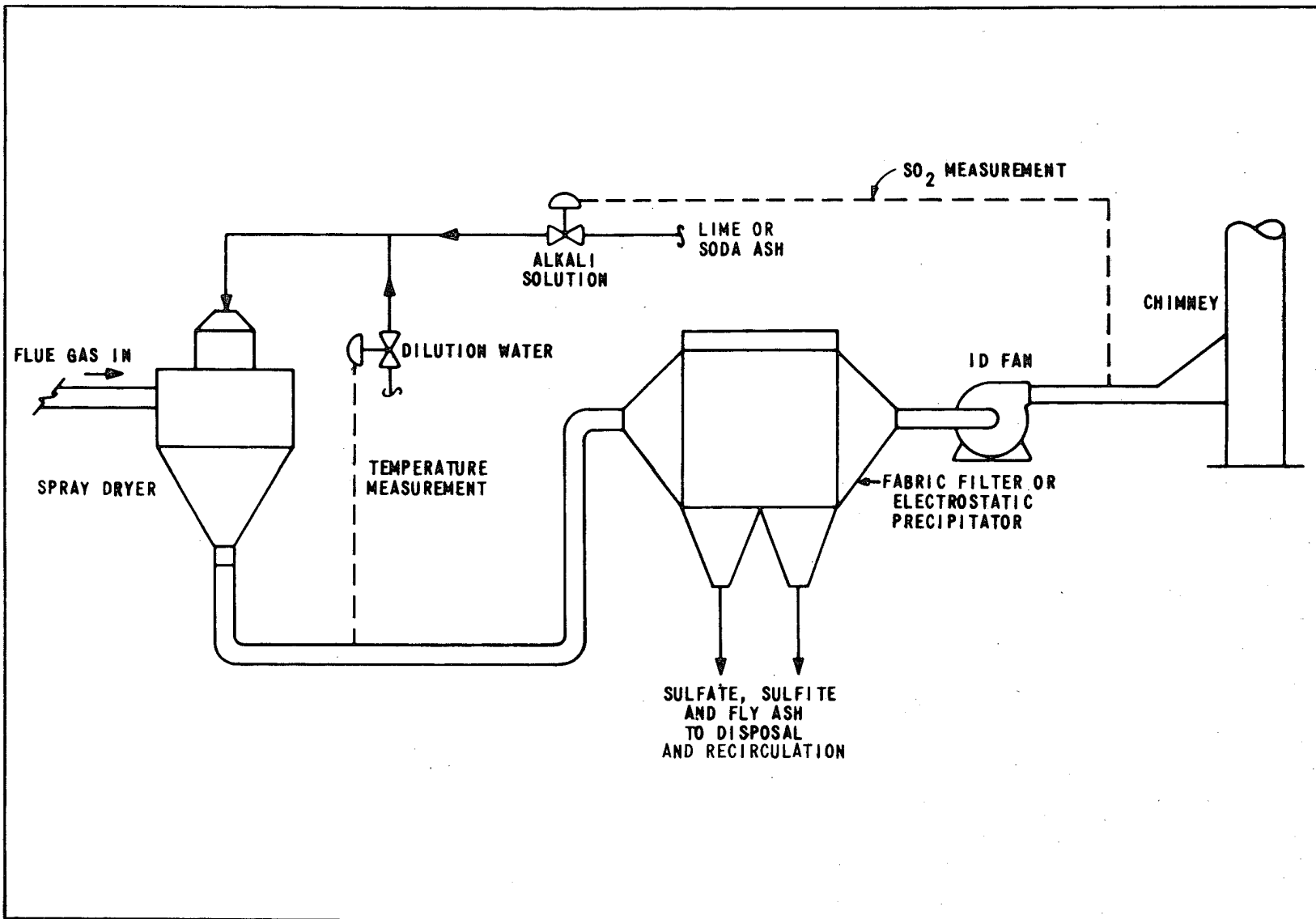
FIGURE 3.7B-4. SPRAY ABSORBER PROCESS
