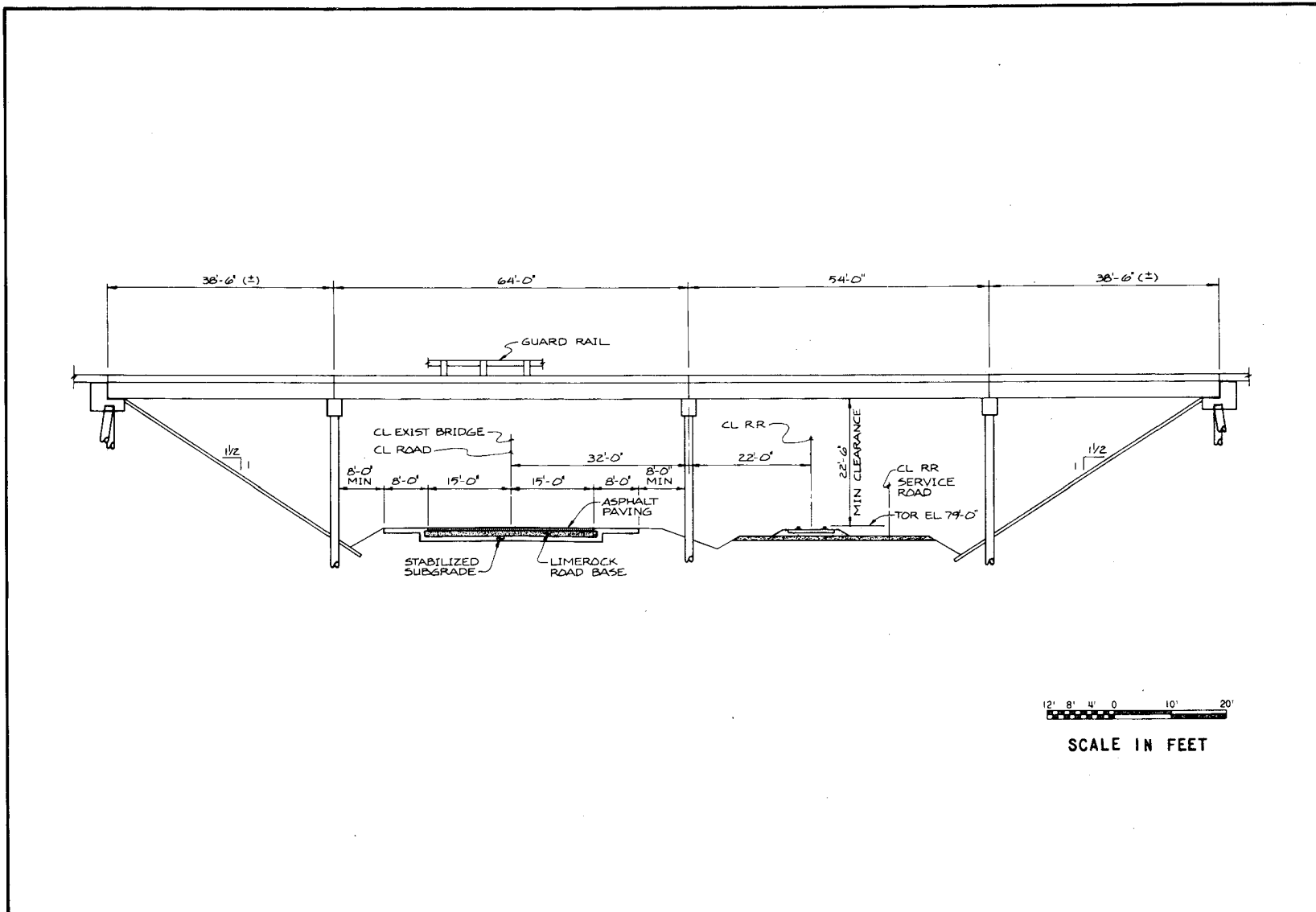
FIGURE 3.9-5. BEE LINE EXPRESSWAY RAILROAD UNDERPASS
