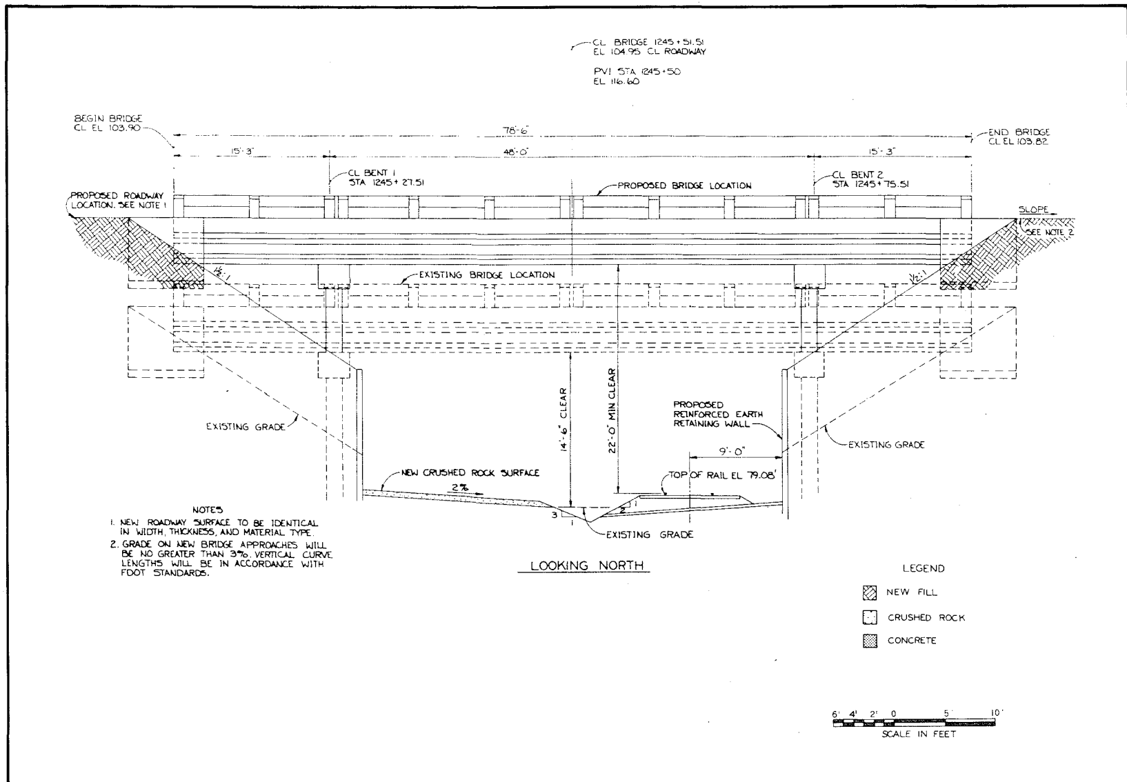
FIGURE 3.9-5. BEE LINE EXPRESSWAY RAILROAD UNDERPASS
