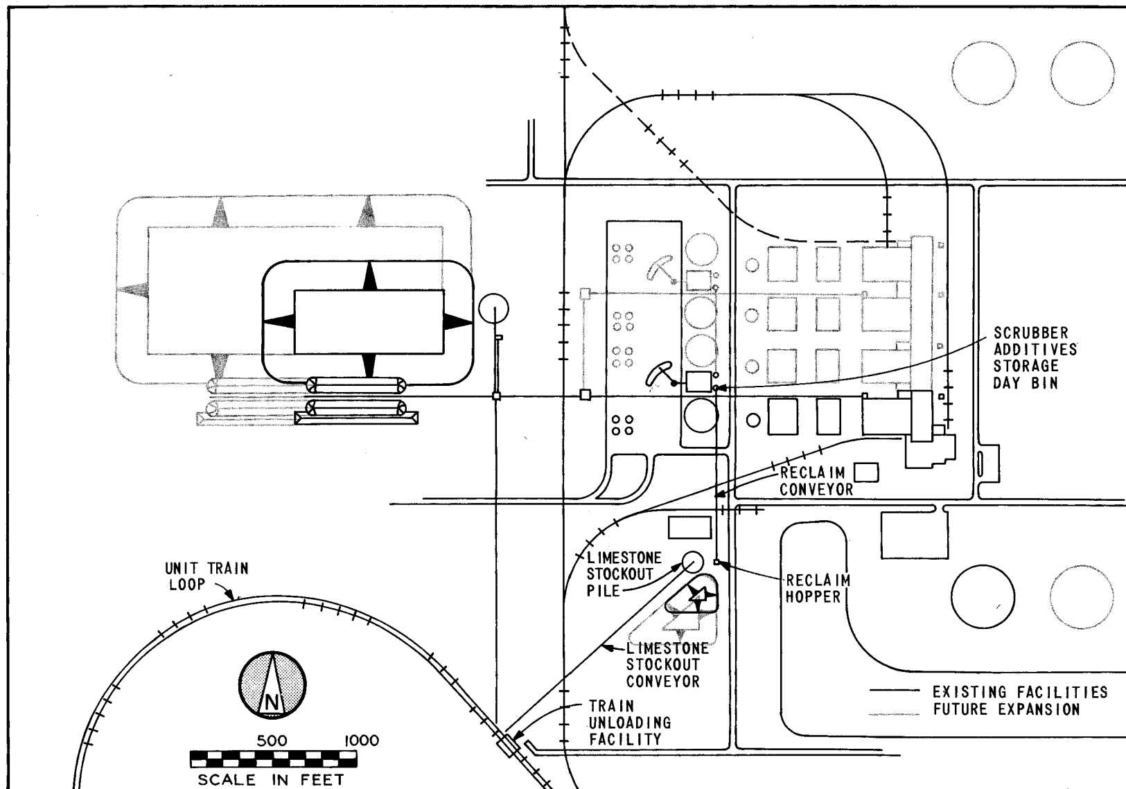
FIGURE 3.9-10. SCRUBBER ADDITIVE HANDLING SYSTEM LAYOUT
