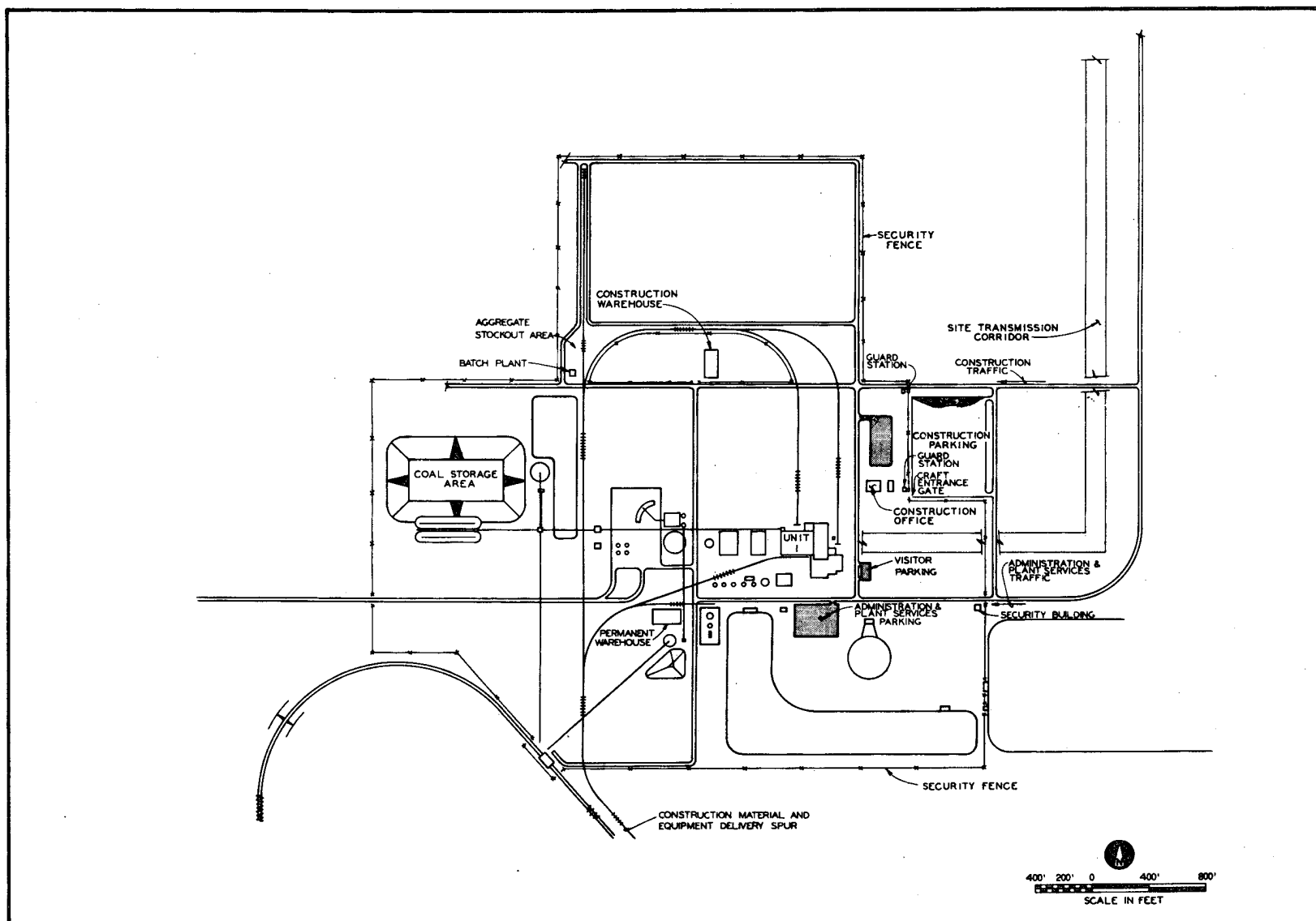
FIGURE 3.9-7. SITE ROADS AND SECURITY
