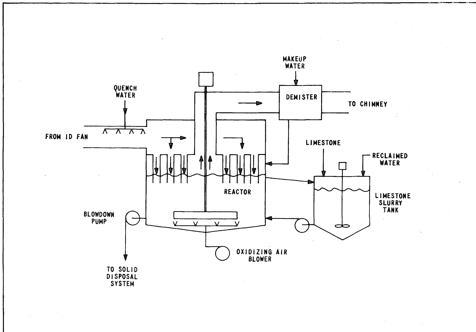
FIGURE 3.7B-7. FLUE GAS SPARGING (CHIYODA) PROCESS
