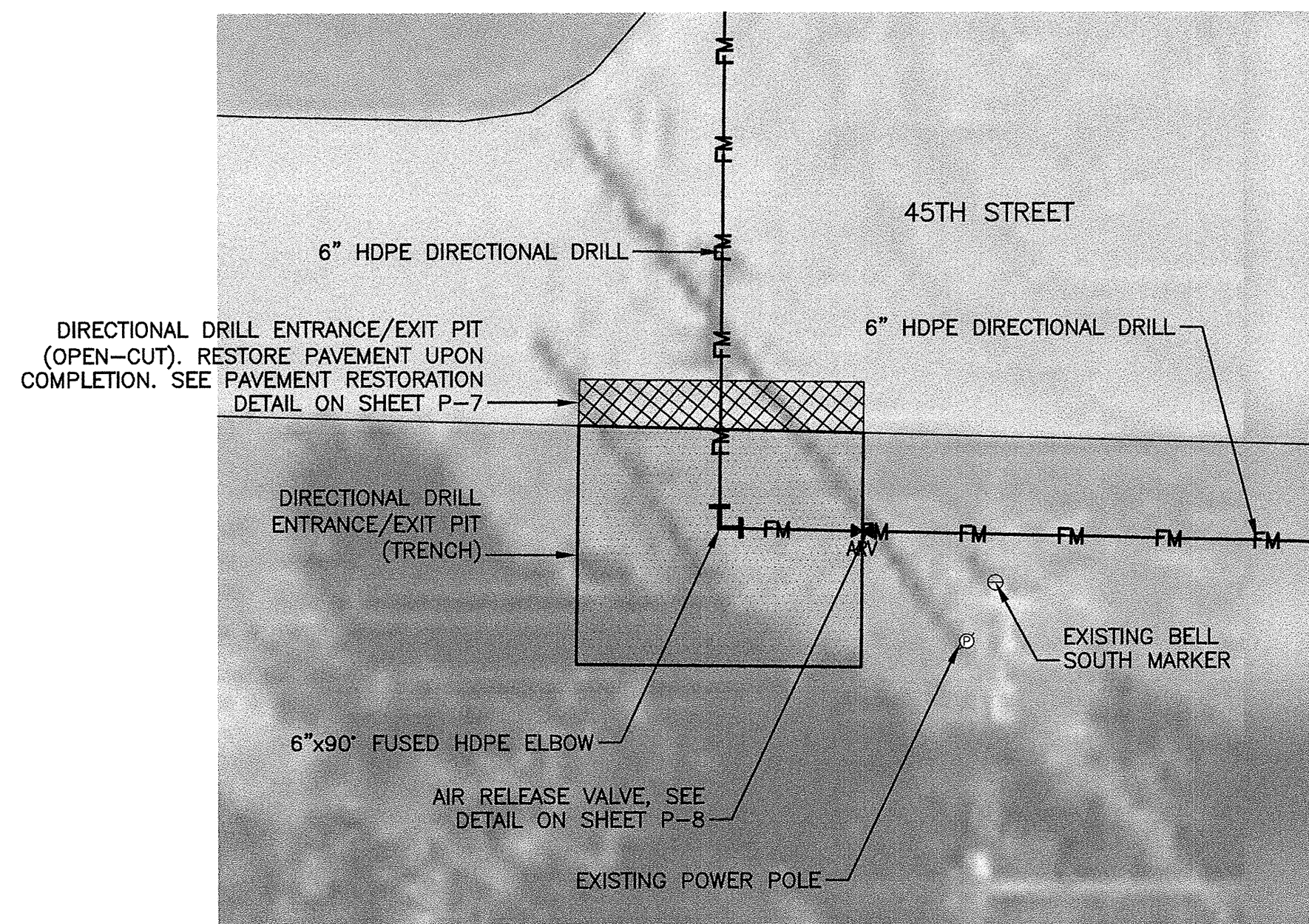
FORCEMAIN 6"x90" BEND - ENLARGED PLAN VIEW STA:12+59.06 SCALE: 1"=10.0'
