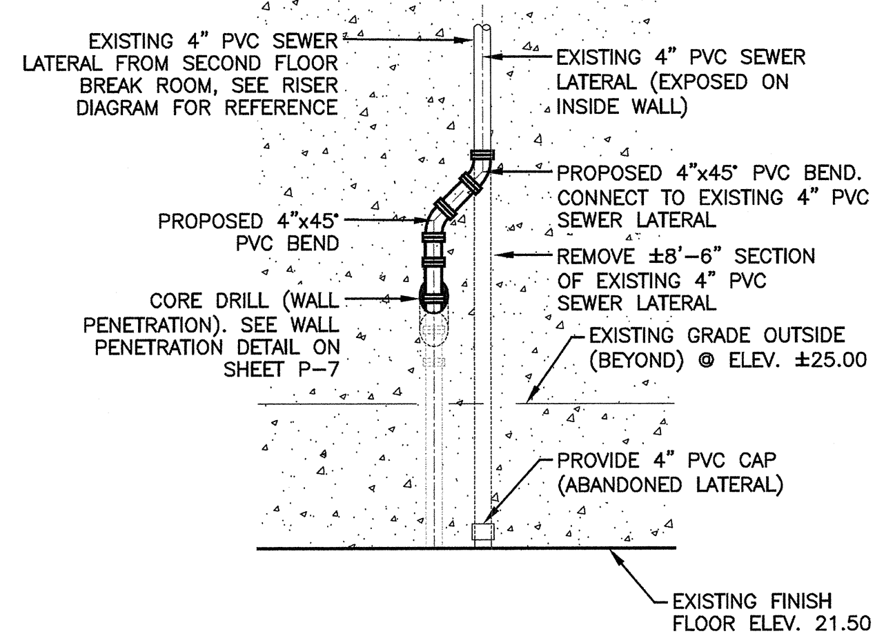
FRONT VIEW - INTERIOR WALL CONNECTION TO EXISTING LATERAL SCALE: N.T.S.
