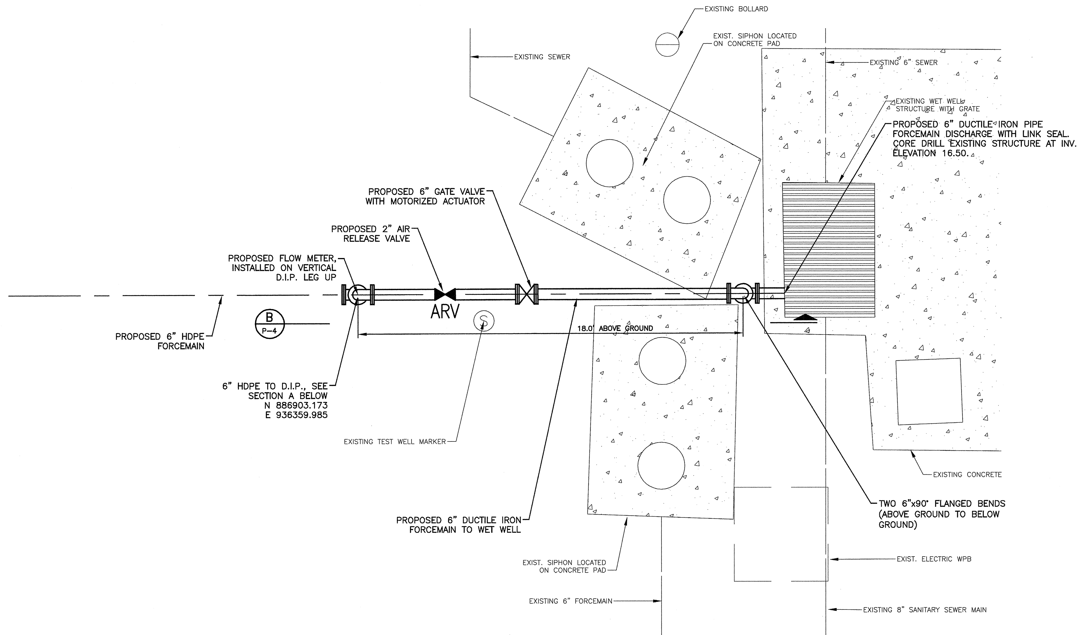
FORCEMAIN DISCHARGE PLAN VIEW SCALE: 3/8" = 1'-0"
