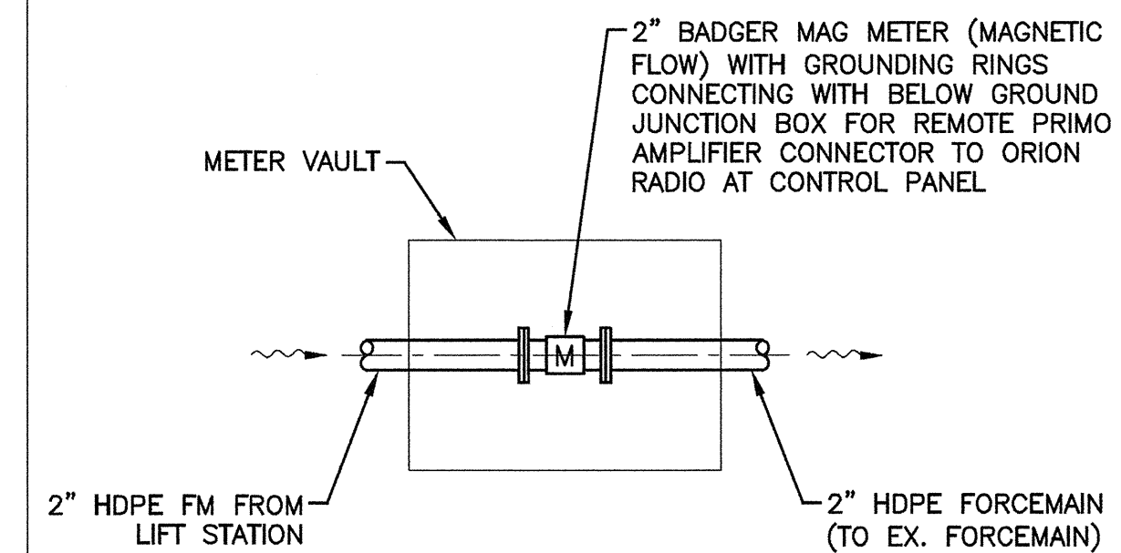
SAMPLE POINT CONNECTION N.T.S.
