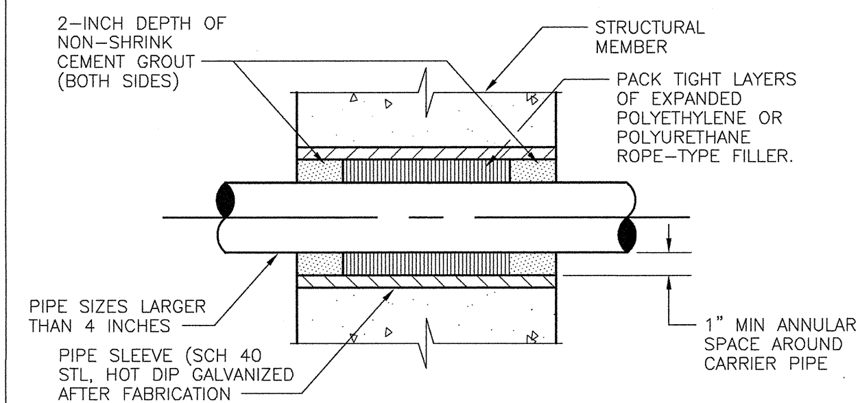
PIPE DIAMETER OVER 4 INCHES
