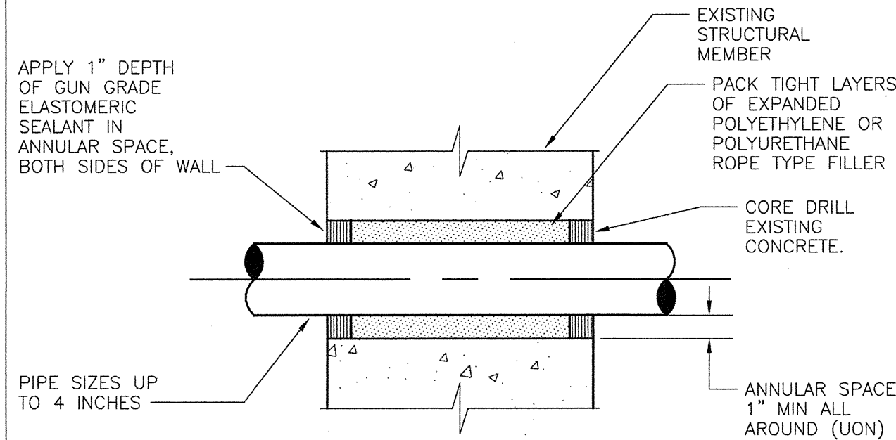
PIPE DIAMETER UP TO 4 INCHES
