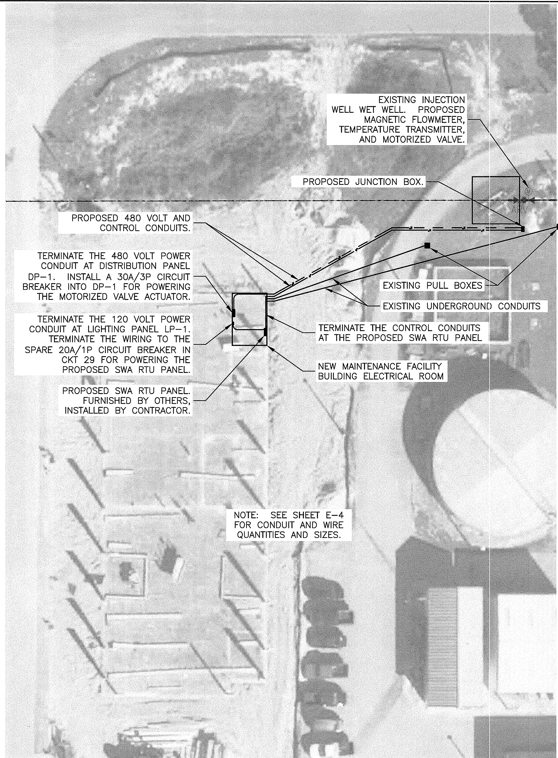
SWA SITE SCALE: 1"=20.00'
