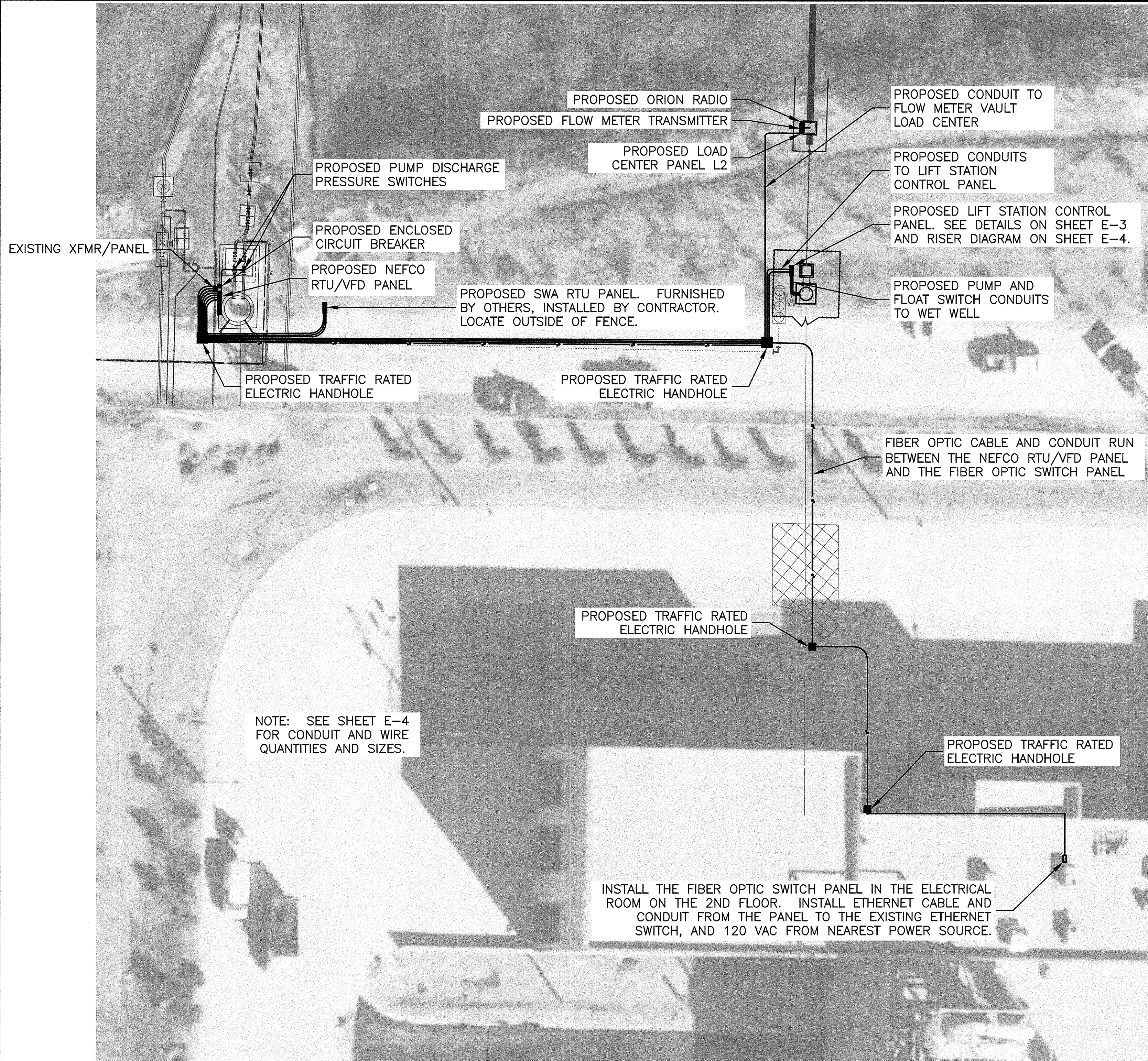
NEFCO SITE SCALE: 1"=20.00'
