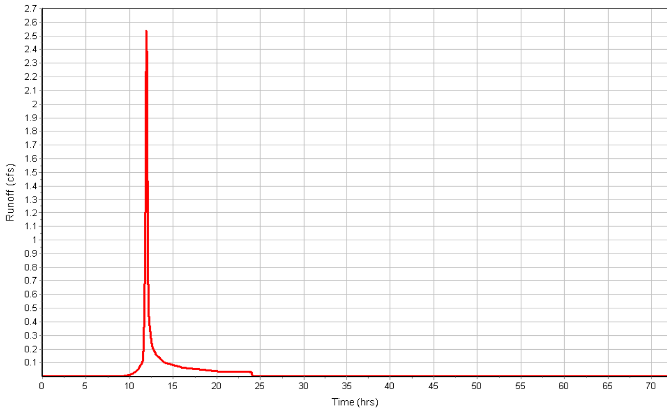
Runoff Hydrograph
