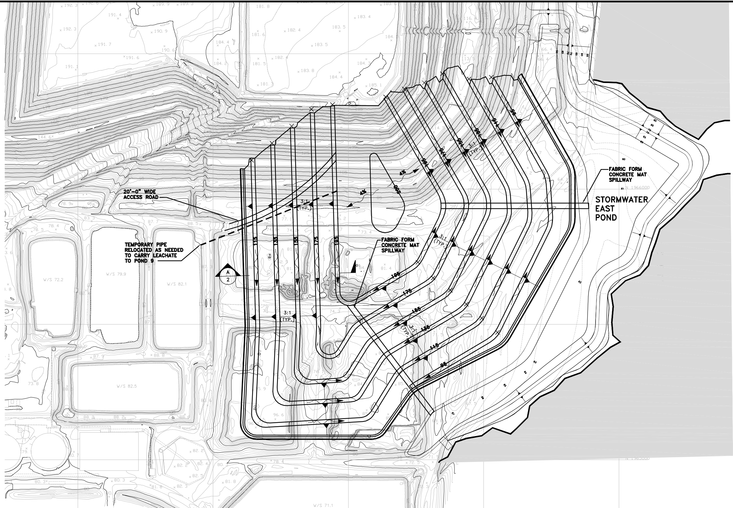
SITE PLAN 1 SCALE: 1" = 200'
