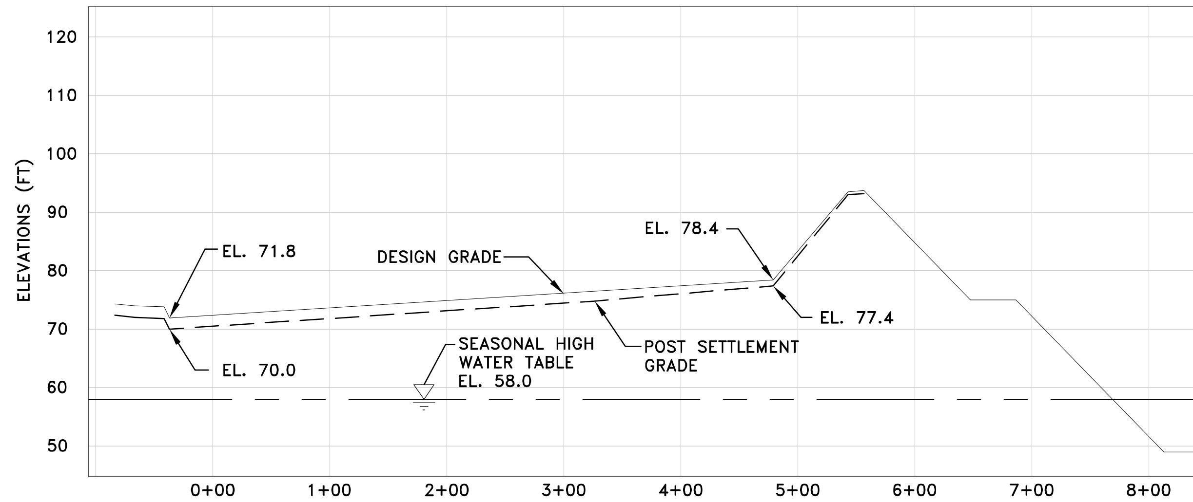
SECTION A SCALE: 1"=80' H 1"=16' V
