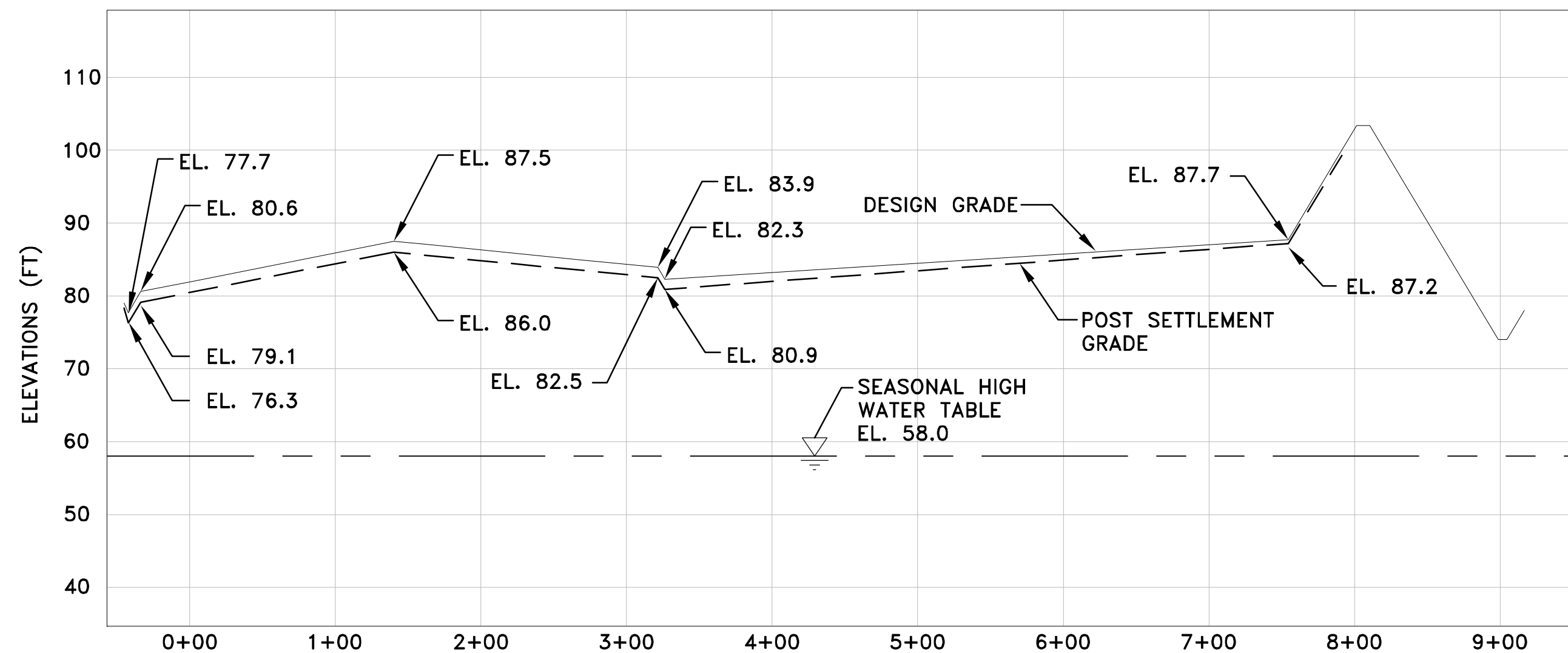
SECTION B SCALE: 1"=80' H 1"=16' V
