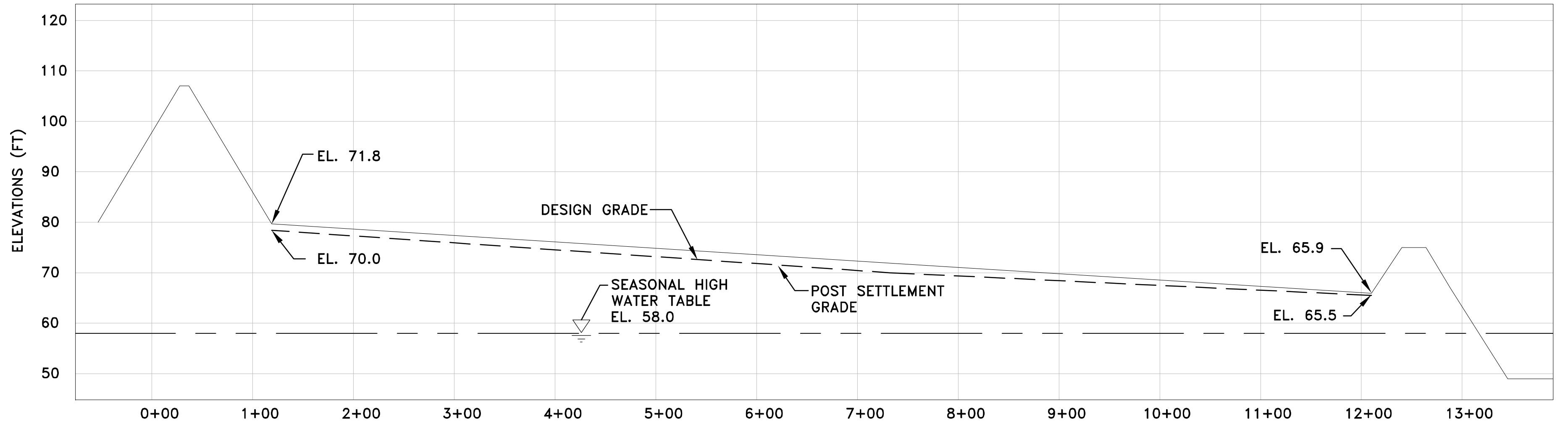
SECTION C SCALE: 1"=80' H 1"=16' V
