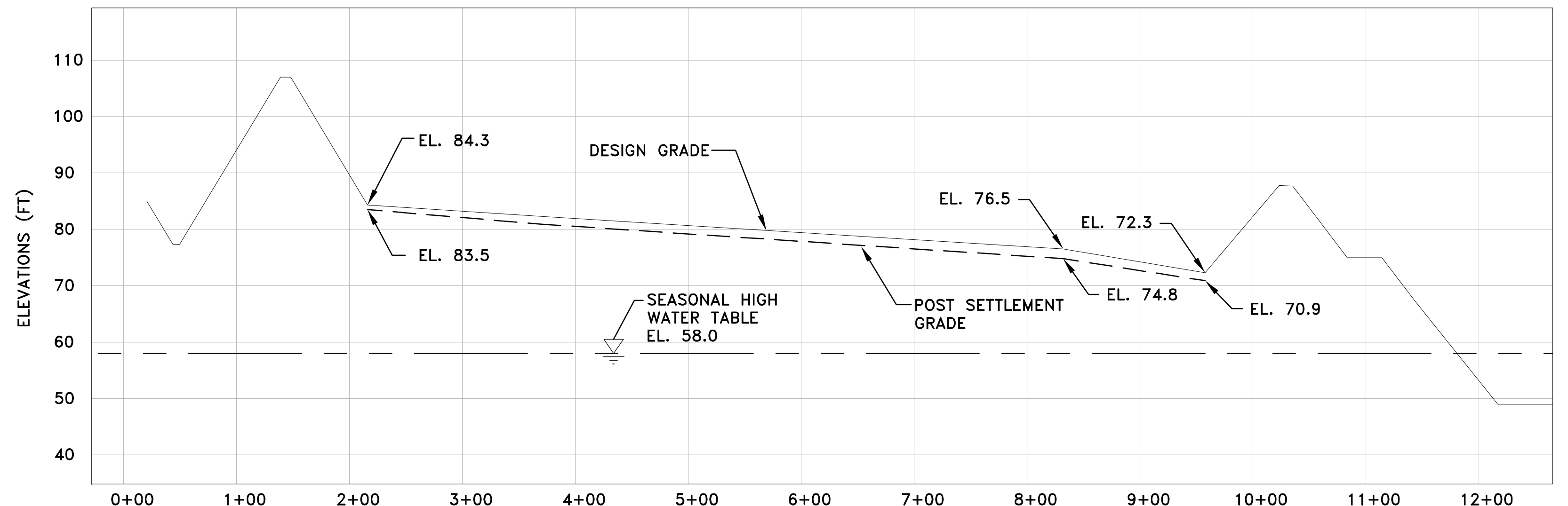
SECTION D SCALE: 1"=80' H 1"=16' V
