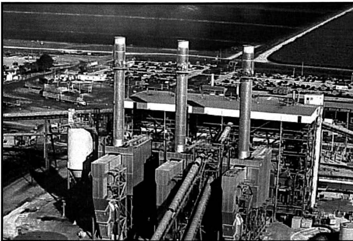
3.2-3c. NHPP Existing Biomass Boilers (view looking north).
