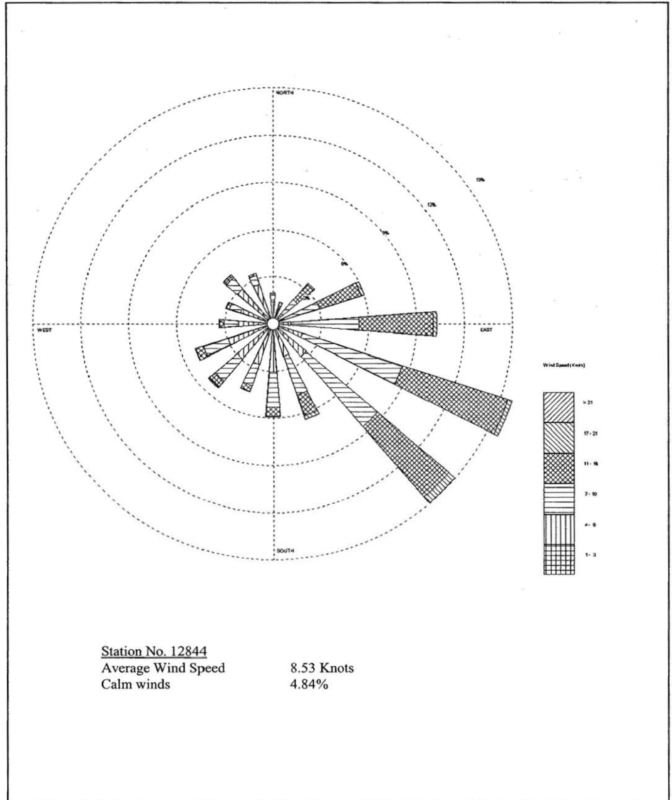
Figure 2.3-4. Summer Wind Rose for Palm Beach International Airport, Florida (June - August 1987 - 1991)
