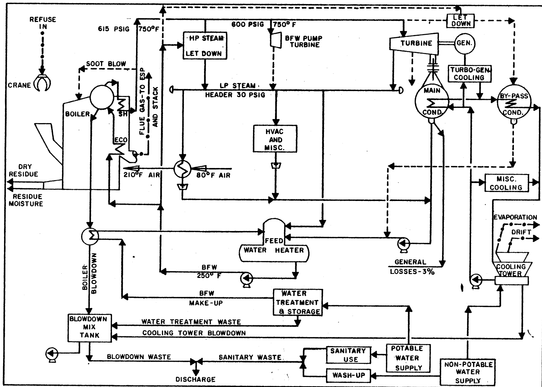
PROCESS FLOW DIAGRAM
