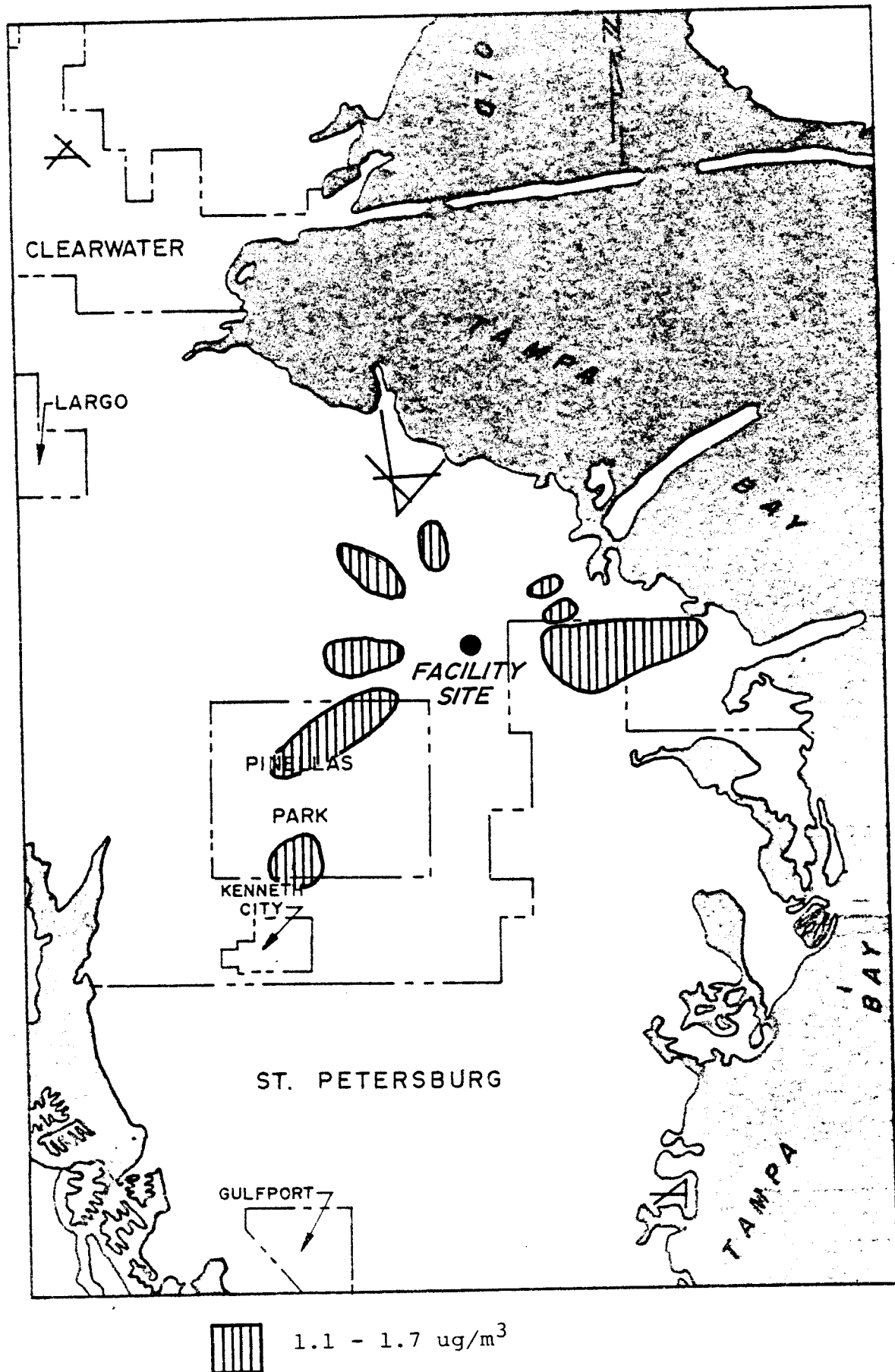
FIGURE 9 CALCULATED MAXIMUM 24-HOUR TSP CONCENTRATION ( \mu\text{g}/\text{m}^3 )
