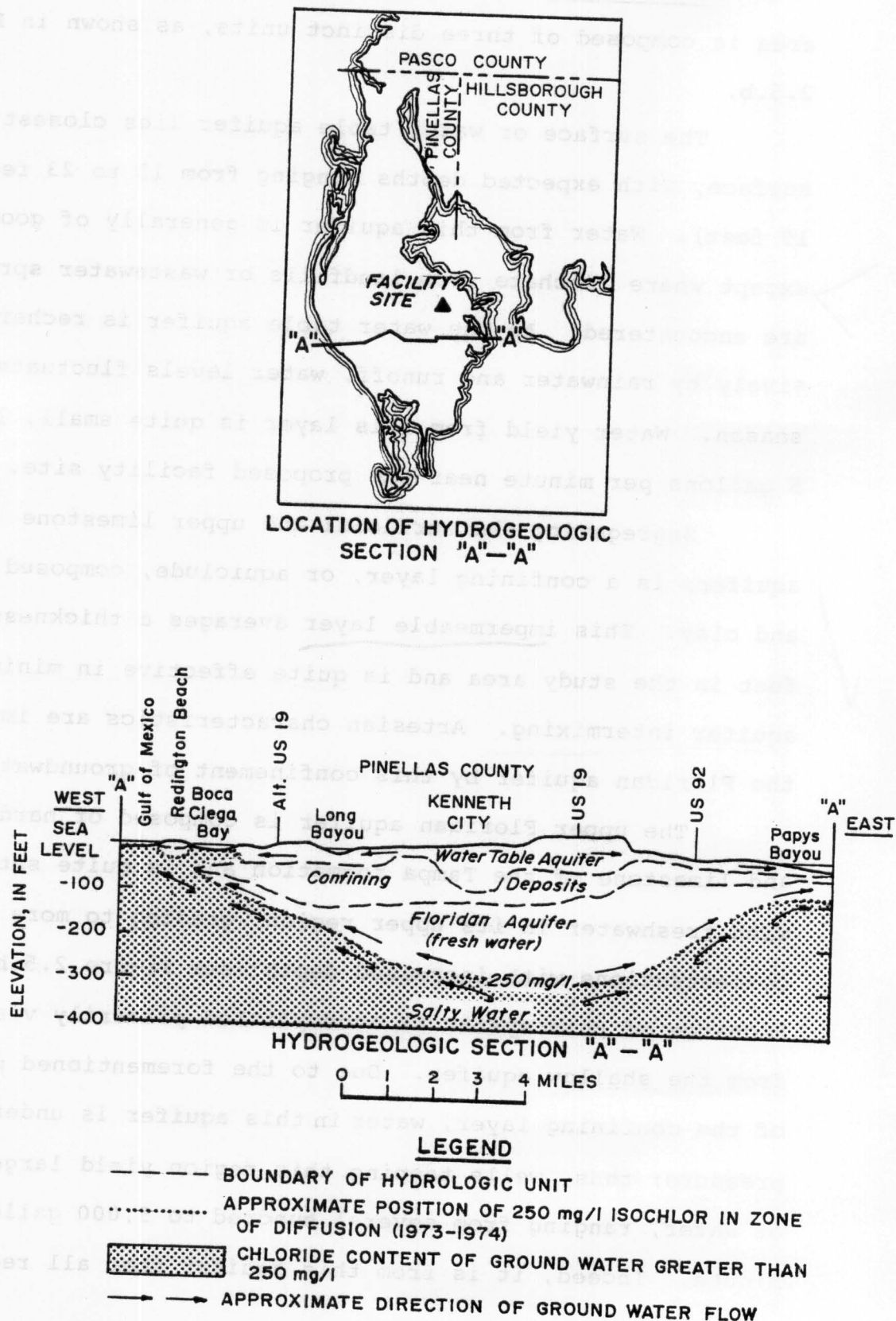
FIGURE 2.5.b. HYDROGEOLOGIC CROSS SECTION IN VICINITY OF STUDY AREA
