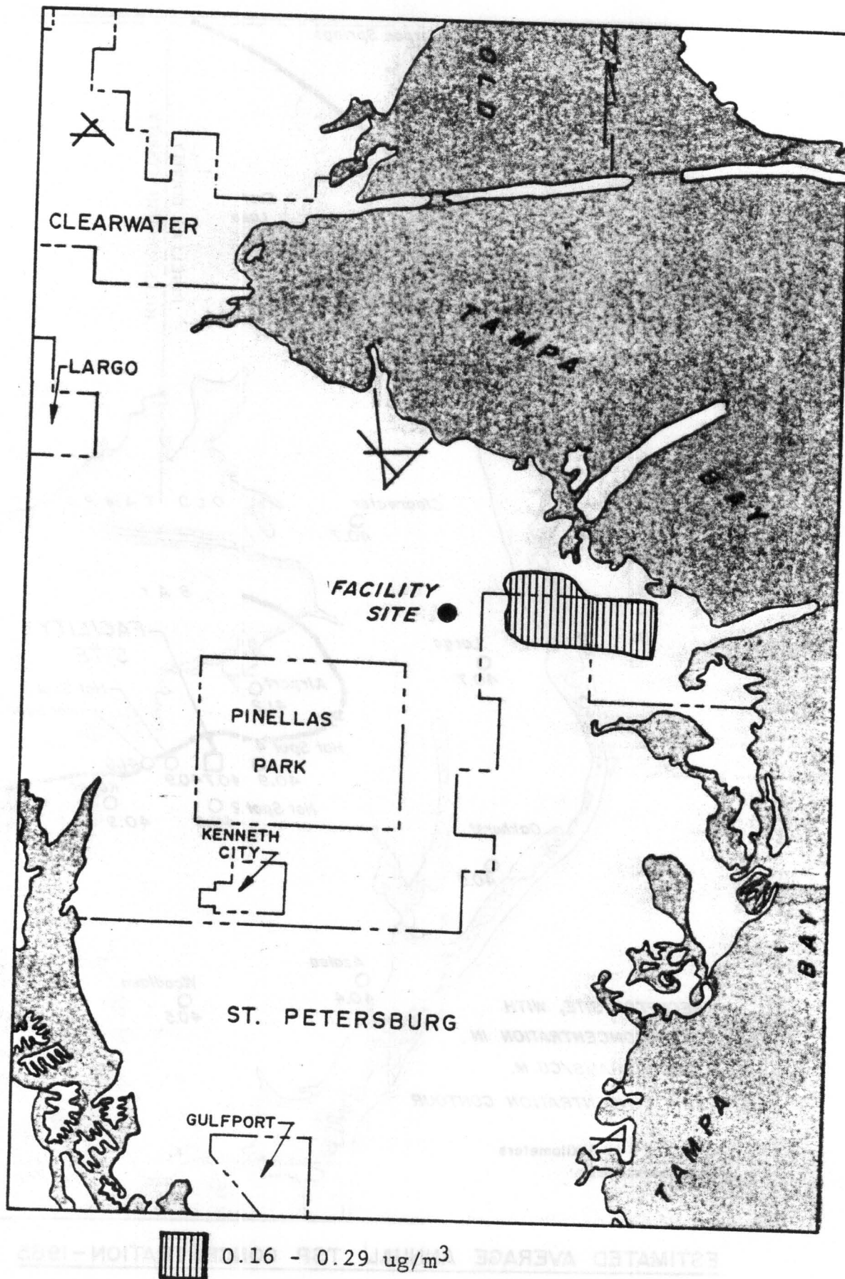
FIGURE 12 CALCULATED MAXIMUM ANNUAL MEAN \text{SO}_2 CONCENTRATION ( \mu\text{g}/\text{m}^3 ), to 5.0 KILOMETERS
