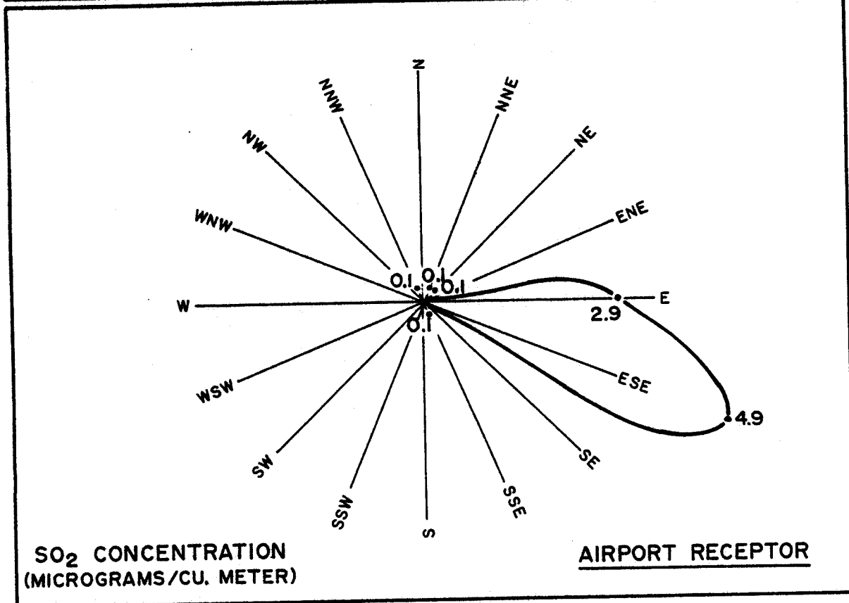
POINT ROSES FOR SO 2 , 1985 (FROM CDMQC)
