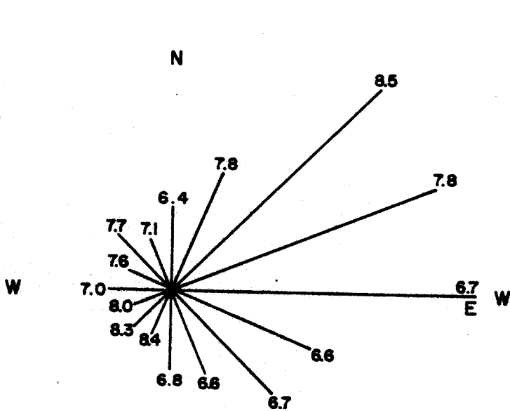
FIGURE 26.b. MONTHLY WIND ROSES McDILL AFB, 1942-1972
