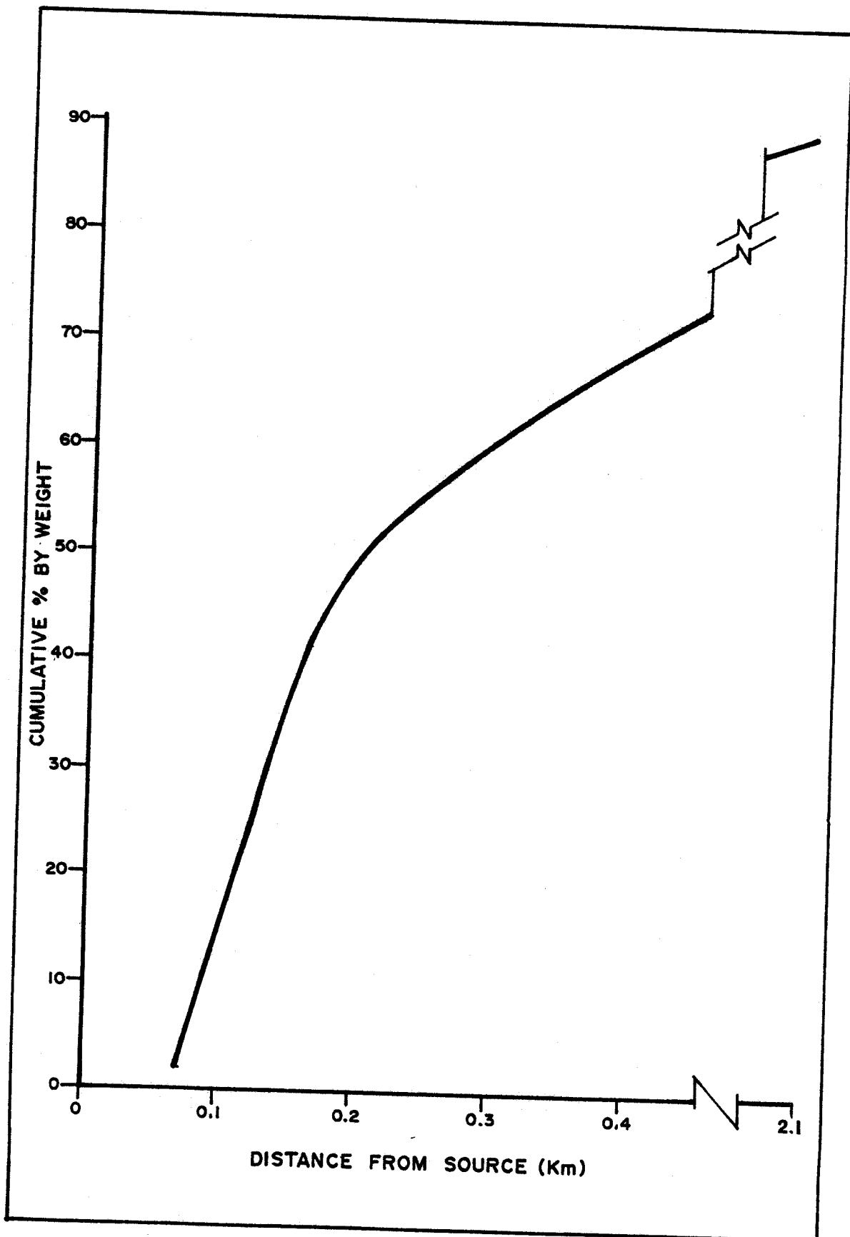
DEPOSITION DISTANCES FOR DRIFT PARTICLES
