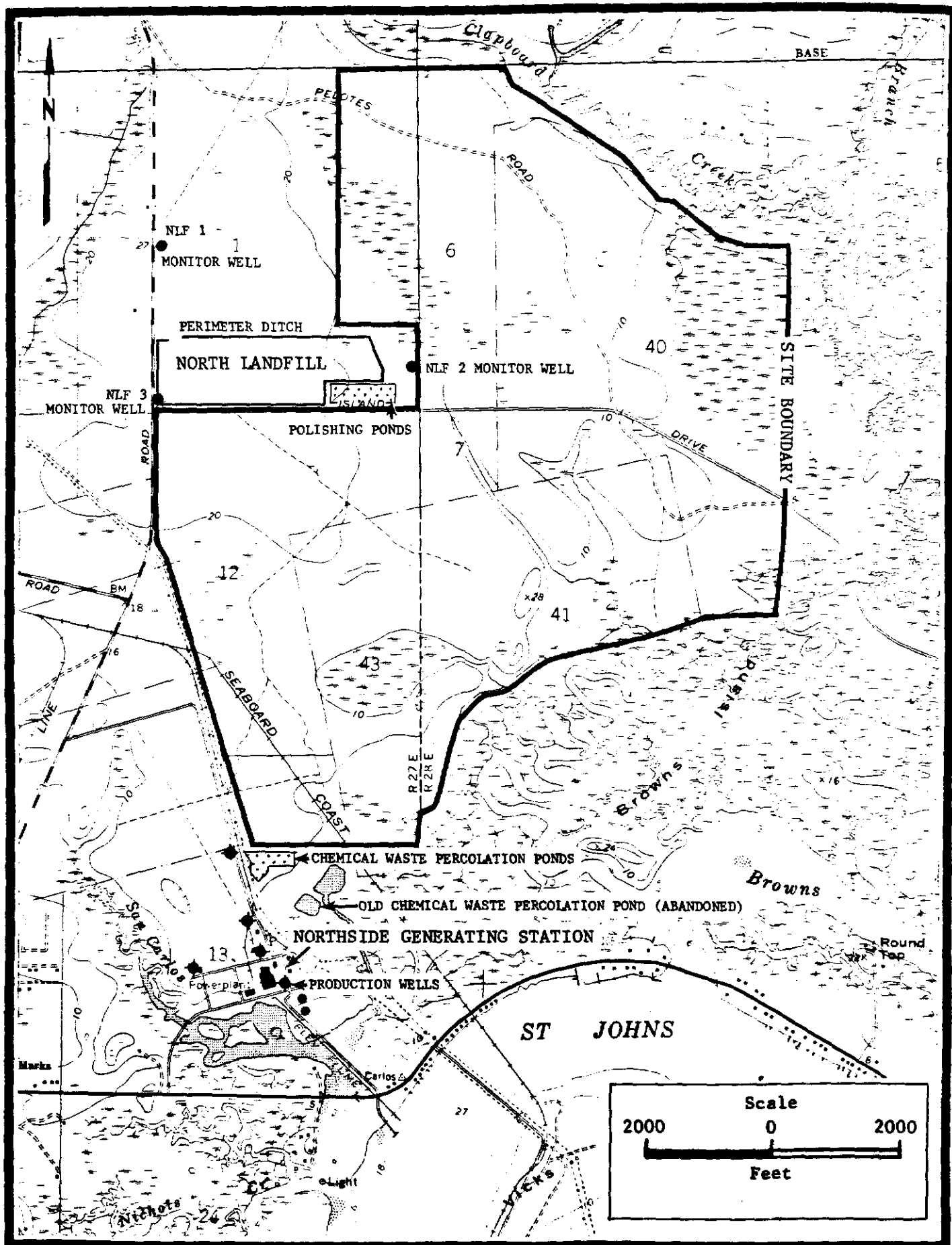
Figure D-19 Locations of Adjacent Facilities
