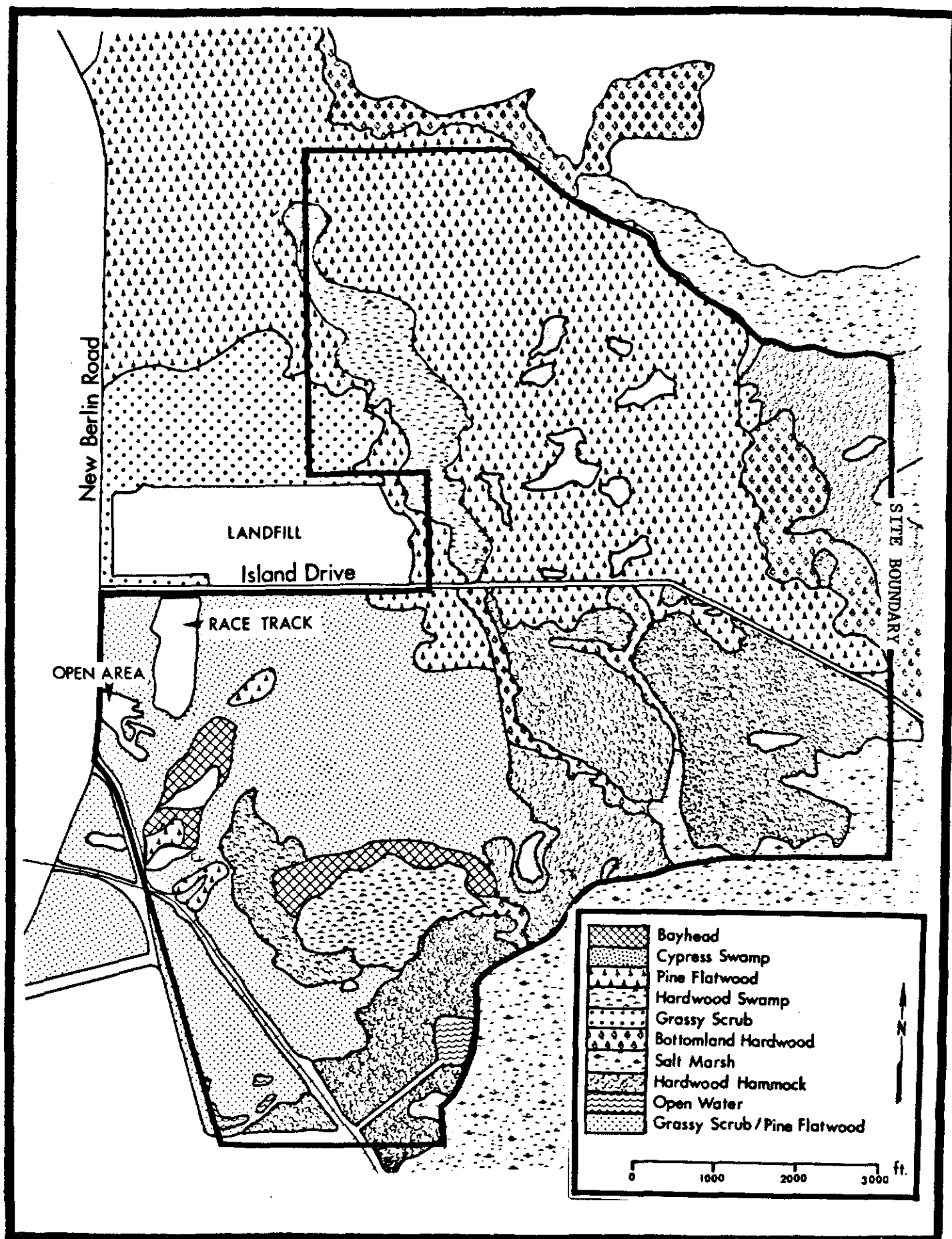
Figure A-1 Vegetation Communities of the Proposed Plant Site
