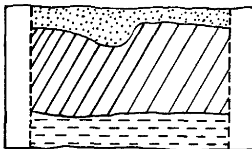
D. 8 Du 678 Test pit 17 Profile East wall
