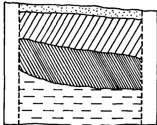
B. 8 Du 673 Test pit 16 Profile East wall
